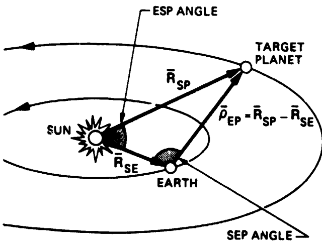
Fig. 2. Definition of Sun- and Earth-to-planet distances, and Earth-Sun- and Sun-Earth-planet angles at any epoch
