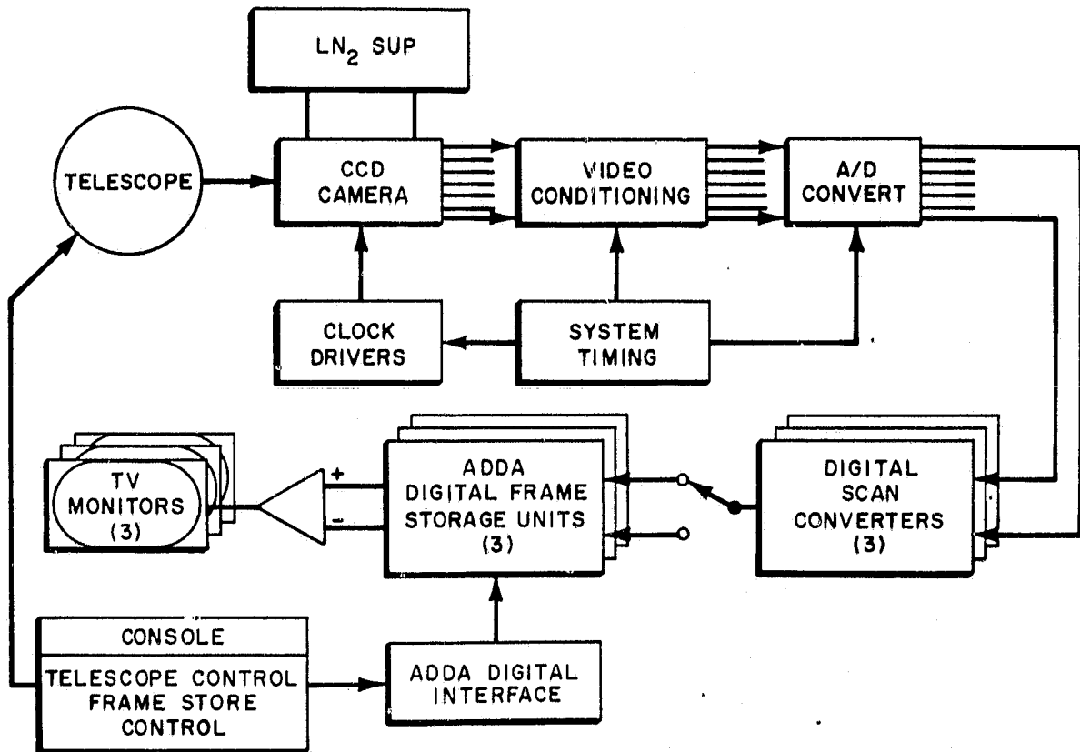
Figure 16. Six-element CCD camera system.
