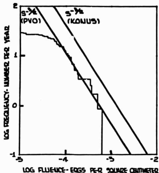
Figure 1. Log N-Log S for PVO data acquired through 1979. Power law functions with a slope of -3/2 as fit to these data and as have been fit to KONUS data 2 are included. (Note the impression that the KONUS data show a higher level of fluence than do the PVO data.)
