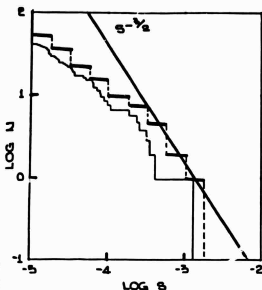
Figure 2. Two presentations of the KONUS data 2 for events with quoted levels of fluence >10^{-5} erg \text{cm}^{-2} . Data taken from the tables 2 are plotted as the lighter, irregular curve using the same convention as in Figure 1. Also shown as the bold histogram are a portion of the binned data with the -3/2 power-law slope transcribed from Figure 168 2 .
