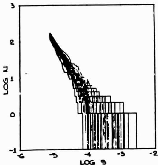
Figure 5. A family of Monte Carlo simulations representing 145 events per year drawn from an N \propto S^{-3/2} distribution. The average slope of the simulated observations was found to be -1.48 \pm 0.15 .
