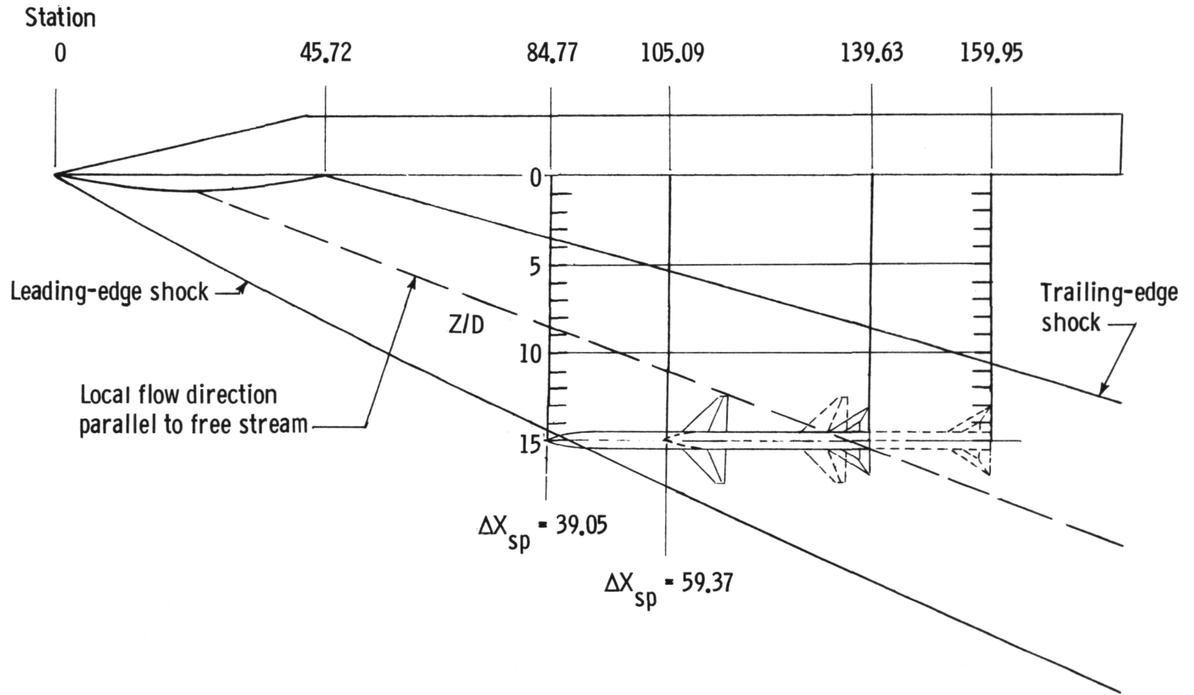
(a) x_p = 0 ; h = 1.27 cm.
