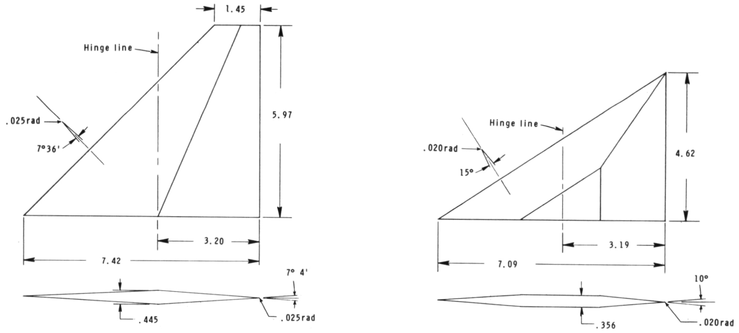
(b) Wing and tail.
