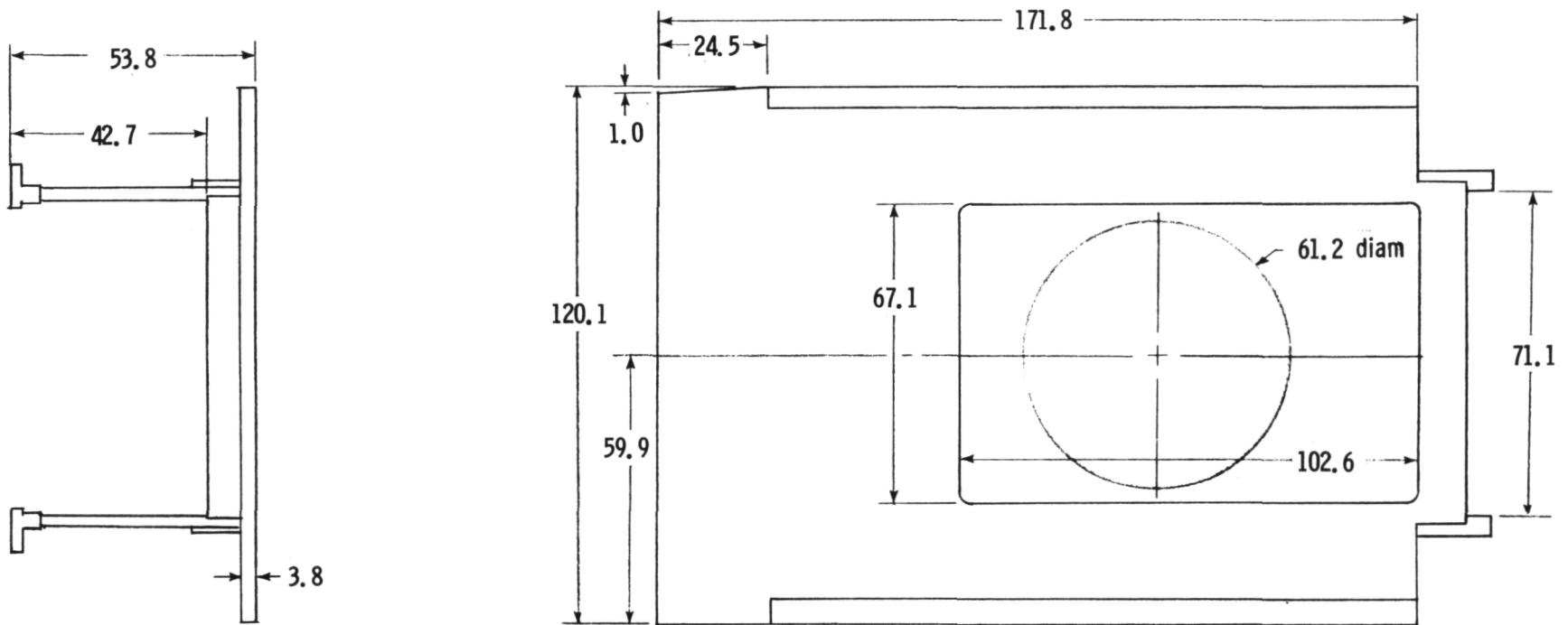
(a) Splitter-plate assembly.
