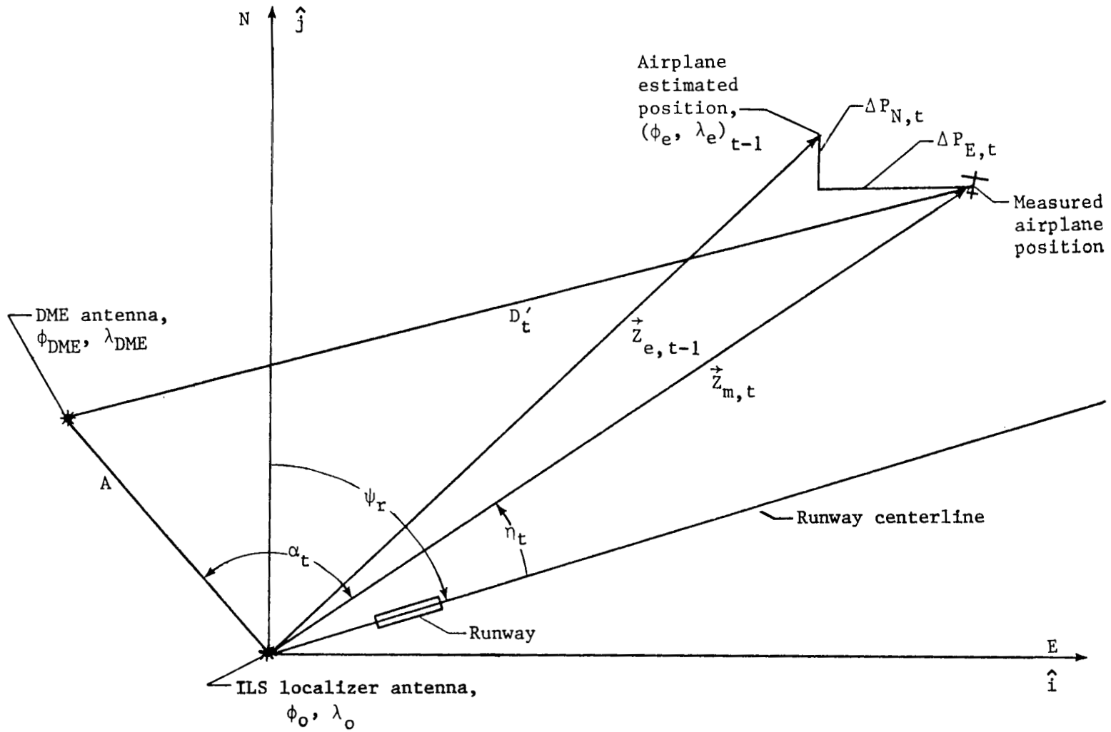
Figure 2.- Geometry pertaining to ILS single-component position estimate: ILS localizer antenna, DME, estimated and measured positions of airplane, and runway with extended centerline.
