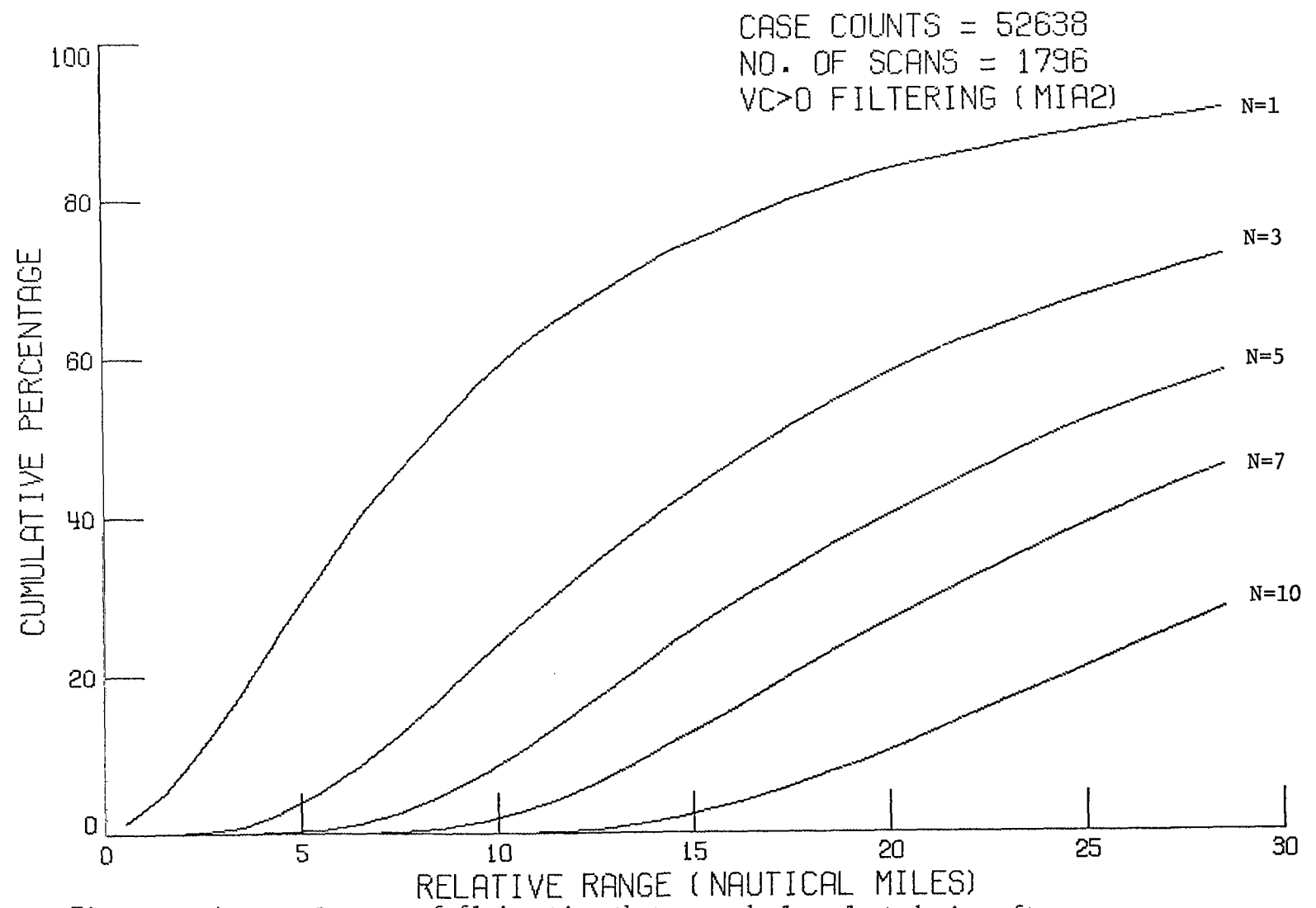
Figure 7.21 Average Percent of flying time that a randomly selected aircraft will have N other aircraft simultaneously displayed within a range value given along the horizontal axis. Closing velocity discrimination ( V_c > 0 ). Miami #2 data.
