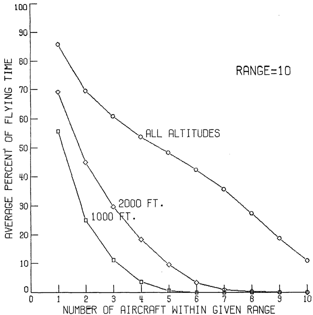
Figure 5.10. Average percentage of flying time in the terminal area vs. number of aircraft observed within a range of 10 n. mi. Curves are given for all altitudes, +1000 ft. altitude, and +2000 ft. altitude.
