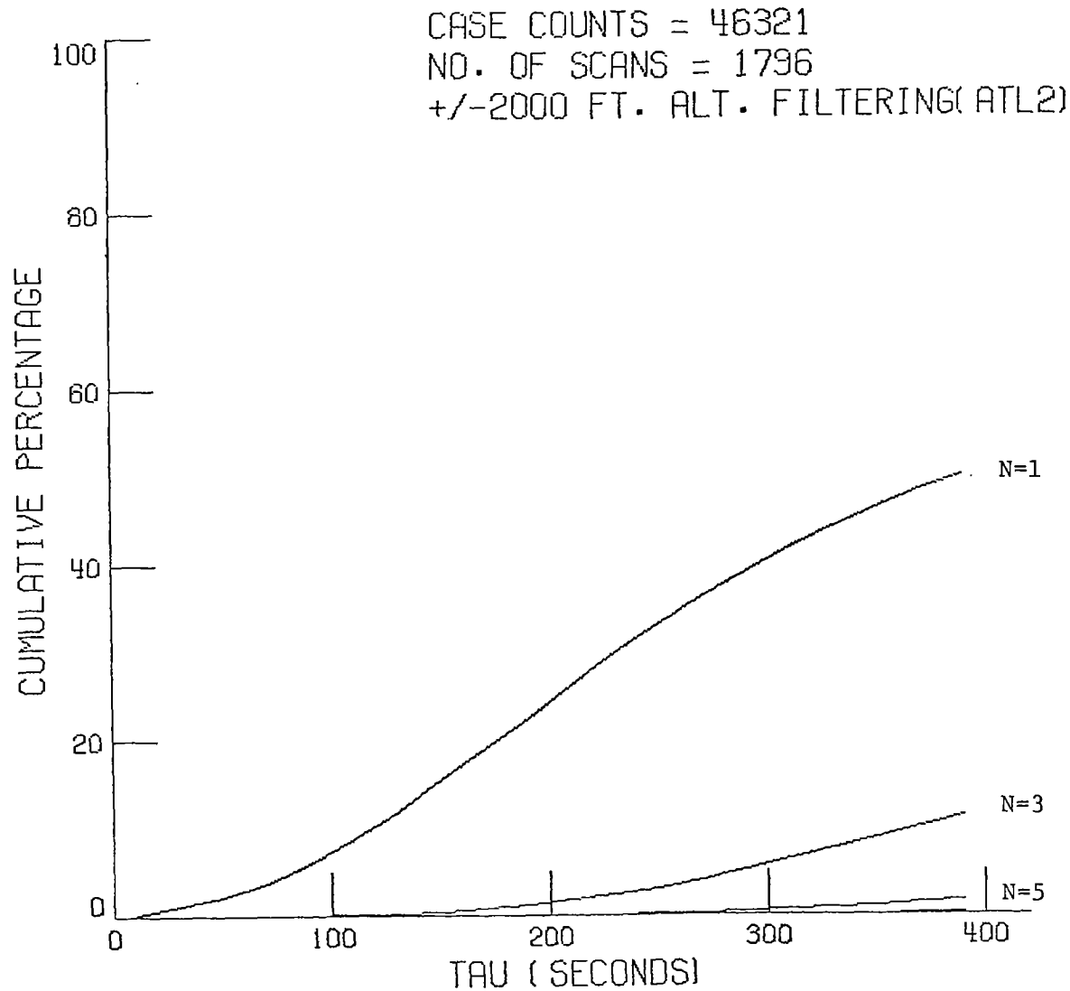
Figure 7.27 Average percent of flying time that a randomly selected aircraft will simultaneously observe N other aircraft with a value of the Tau parameter less than the value given along the horizontal axis. Altitude discrimination of \pm 2000 feet. Atlanta #2 data.
