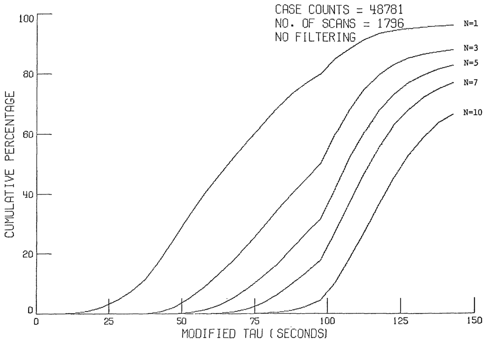
Figure 7.3D Average percent of flying time that a randomly selected aircraft will simultaneously observe N other aircraft with a value of the Modified Tau parameter less than the value given along the horizontal axis. No other discrimination is used. Atlanta #1 data.
