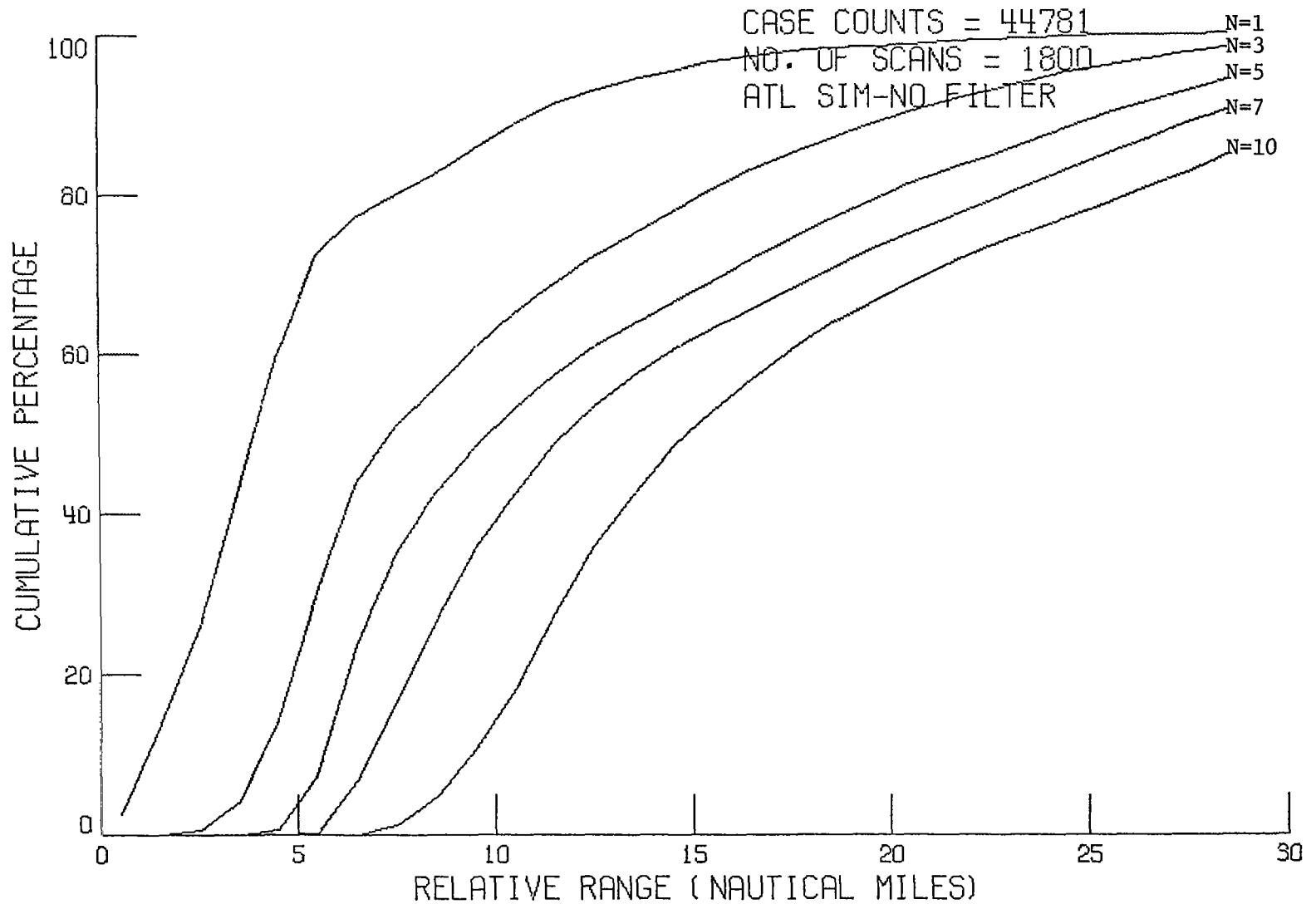
Figure 5.5 Average percent of flying time that a randomly selected aircraft will have N other aircraft simultaneously displayed within a range value given along the horizontal axis. No discrimination is used.
