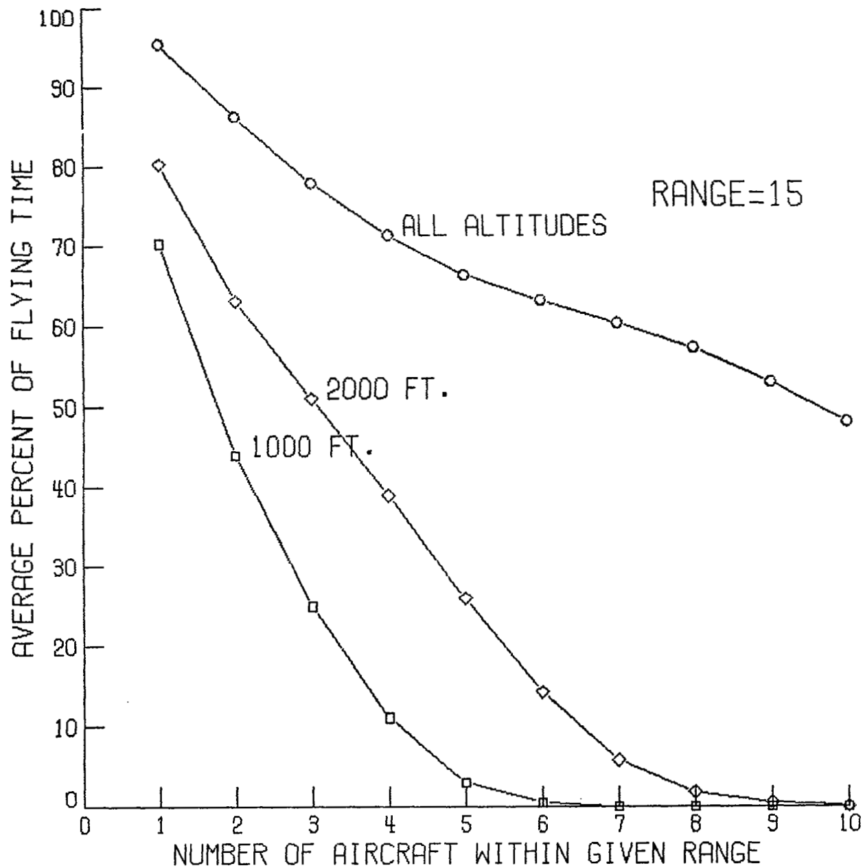
Figure 5.12. Average percentage of flying time in the terminal area vs. number of aircraft observed within a range of 15 n. mi. Curves are given for all altitudes, +1000 ft. altitude, and +2000 ft. altitude.
