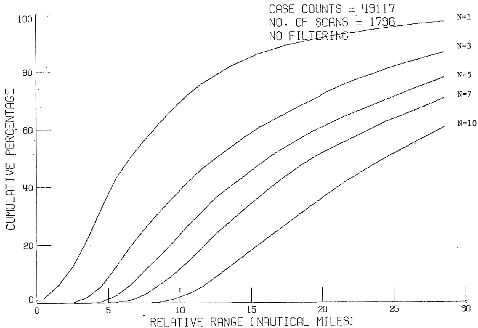
Figure 7.5 Average percent of flying time that a randomly selected aircraft will have N other aircraft simultaneously displayed within a range value given along the horizontal axis. No discrimination is used. Atlanta #1 data.
