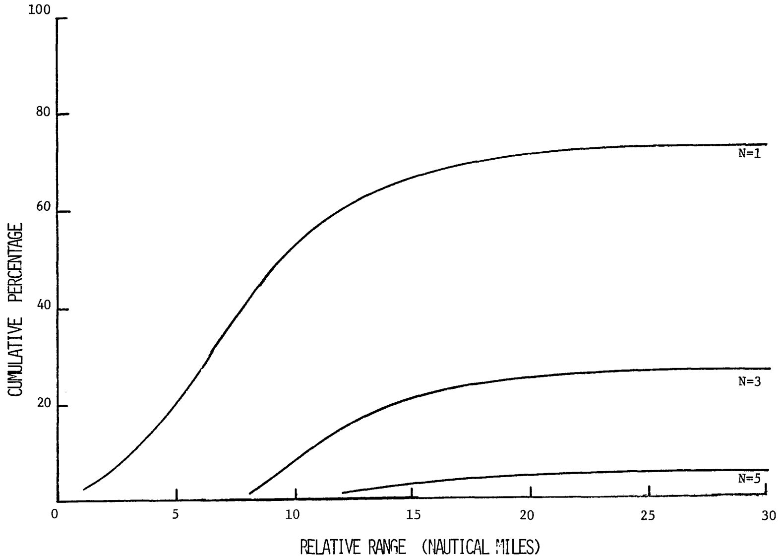
Figure 5.24. Average percent of flying time that a randomly selected aircraft will have N other aircraft simultaneously displayed within a range value given along the horizontal axis for \tau < 180 secs. discrimination.
