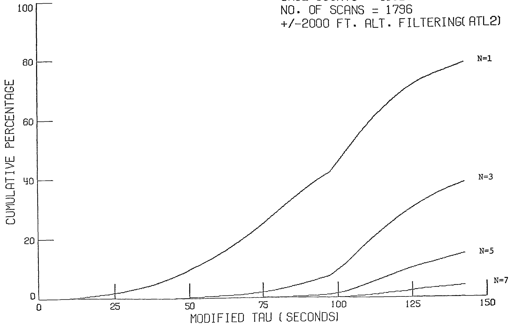
Figure 7.35 Average percent of flying time that a randomly selected aircraft will simultaneously observe N other aircraft with a value of the Modified Tau parameter less than the value given along the horizontal axis. Altitude discrimination of \pm 2000 feet. Atlanta #2 data.
