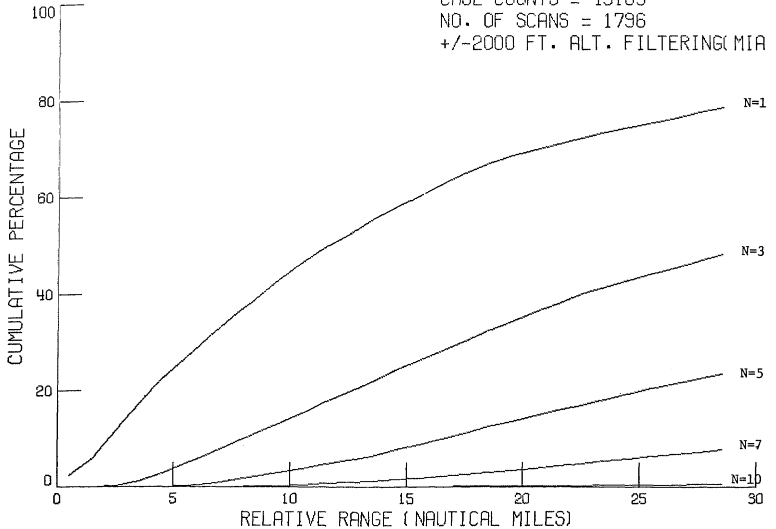
Figure 7.16 Average percent of flying time that a randomly selected aircraft will have N other aircraft simultaneously displayed within a range value given along the horizontal axis. Altitude discrimination of \pm 2000 feet. Miami #2 data.
