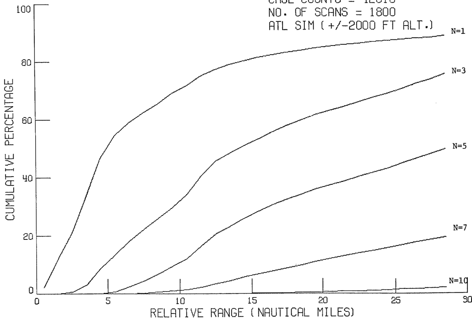
Figure 5.7 Average percent of flying time that a randomly selected aircraft will have N other aircraft simultaneously displayed within a range value given along the horizontal axis. Altitude discrimination of \pm 2,000 feet.
