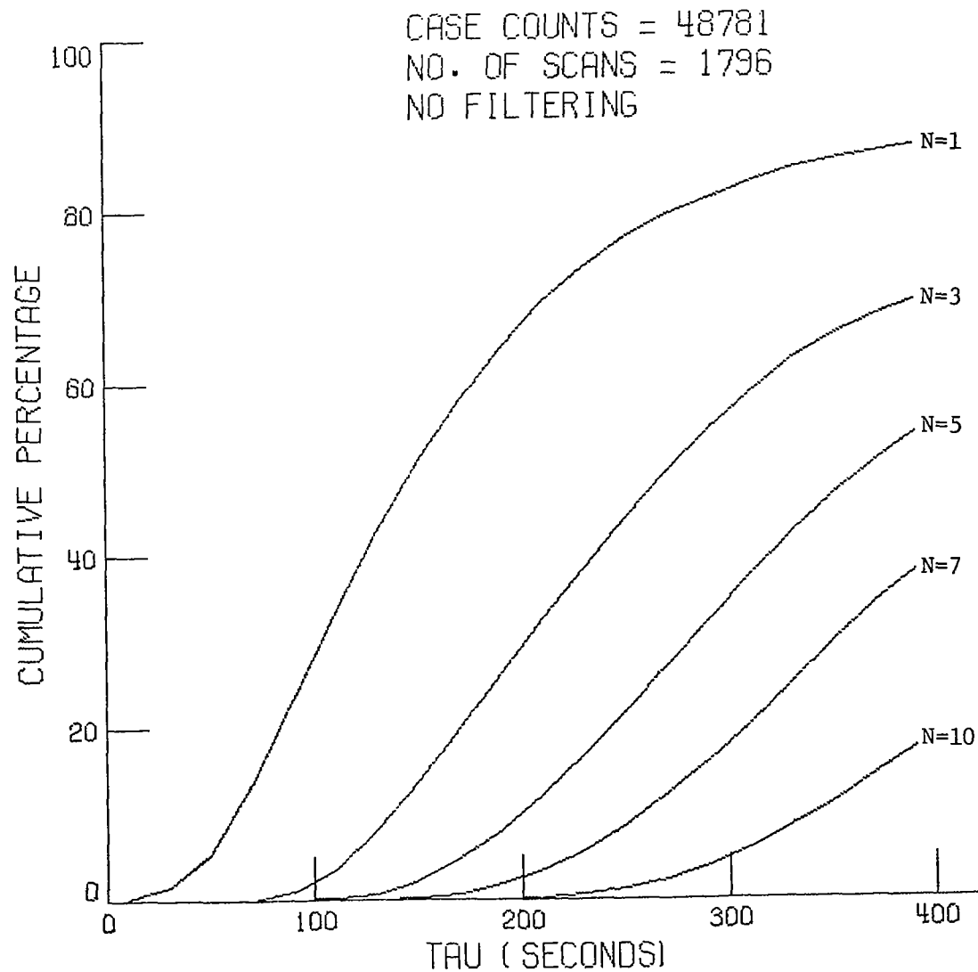
Figure 7.22 Average percentage of flying time that a randomly selected aircraft will simultaneously observe N other aircraft with a value of the Tau parameter less than the value given along the horizontal axis. No other discrimination is used. Atlanta #1 data.
