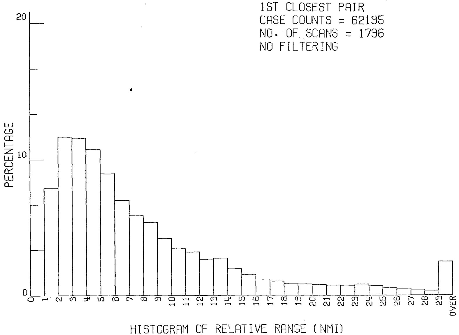
Figure 7.3 Histogram of the average percentage of flying time that a randomly selected aircraft will have at least one other aircraft within the range bins shown along the horizontal axis. No discrimination is used. Miami #1 data.
