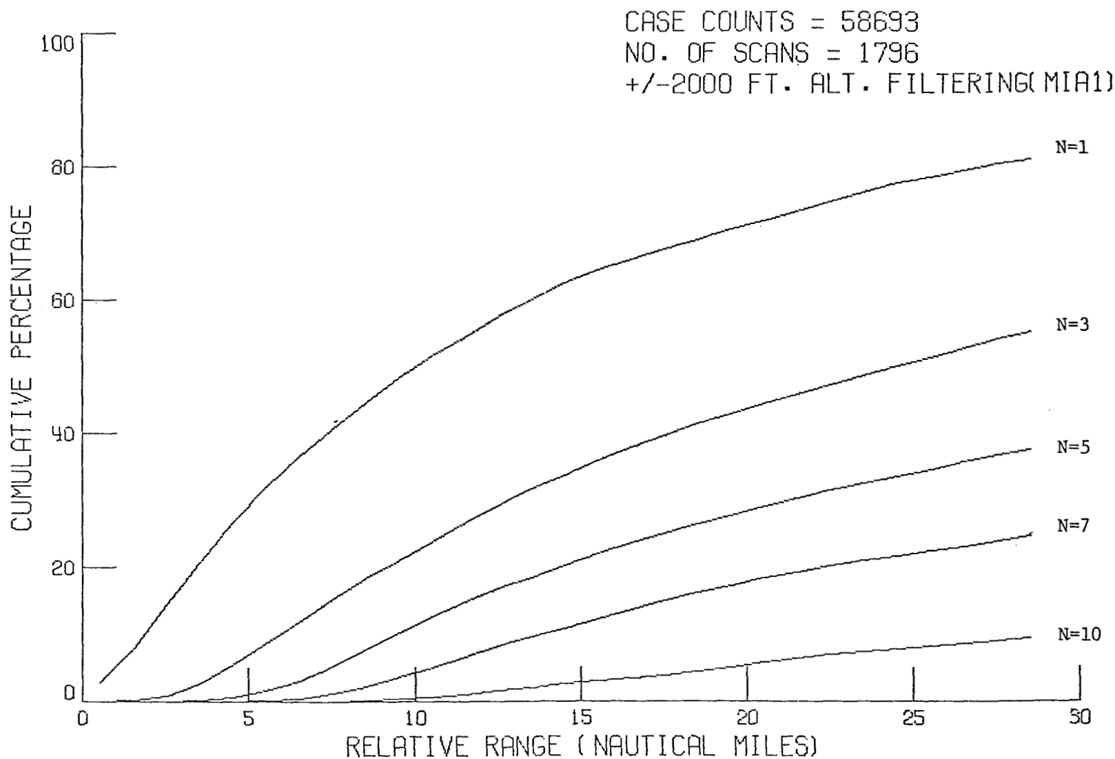
Figure 7.15 Average percent of flying time that a randomly selected aircraft will have N other aircraft simultaneously displayed within a range value given along the horizontal axis. Altitude discrimination of \pm 2000 feet. Miami #1 data.
