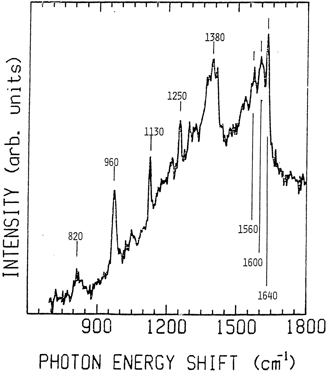
Figure 8 Raman Spectrum of a Dodecane Deposit Collected on Silver in a Stainless Steel Bomb
