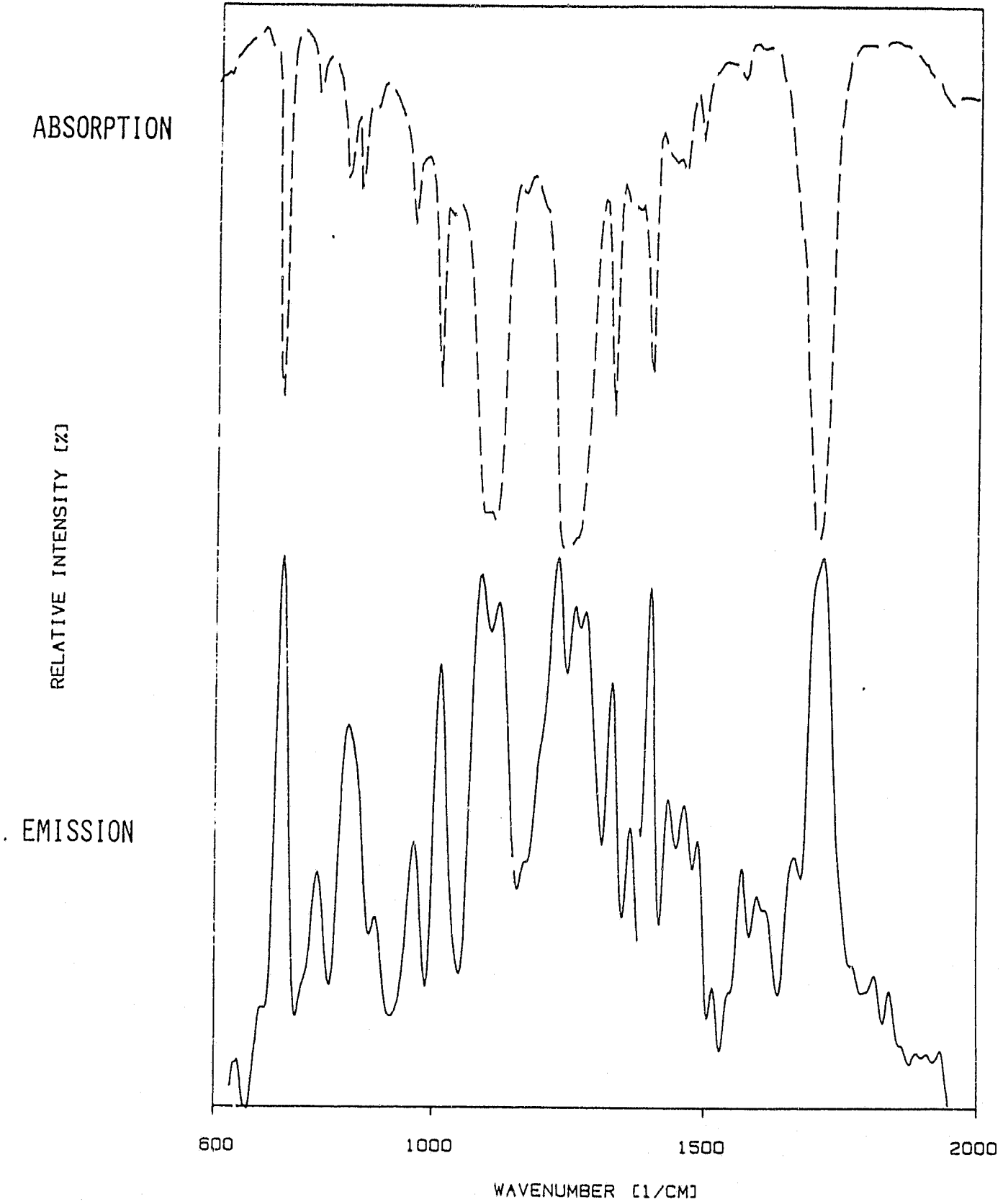
Figure 4 Absorption and Emission Spectrum of Mylar
