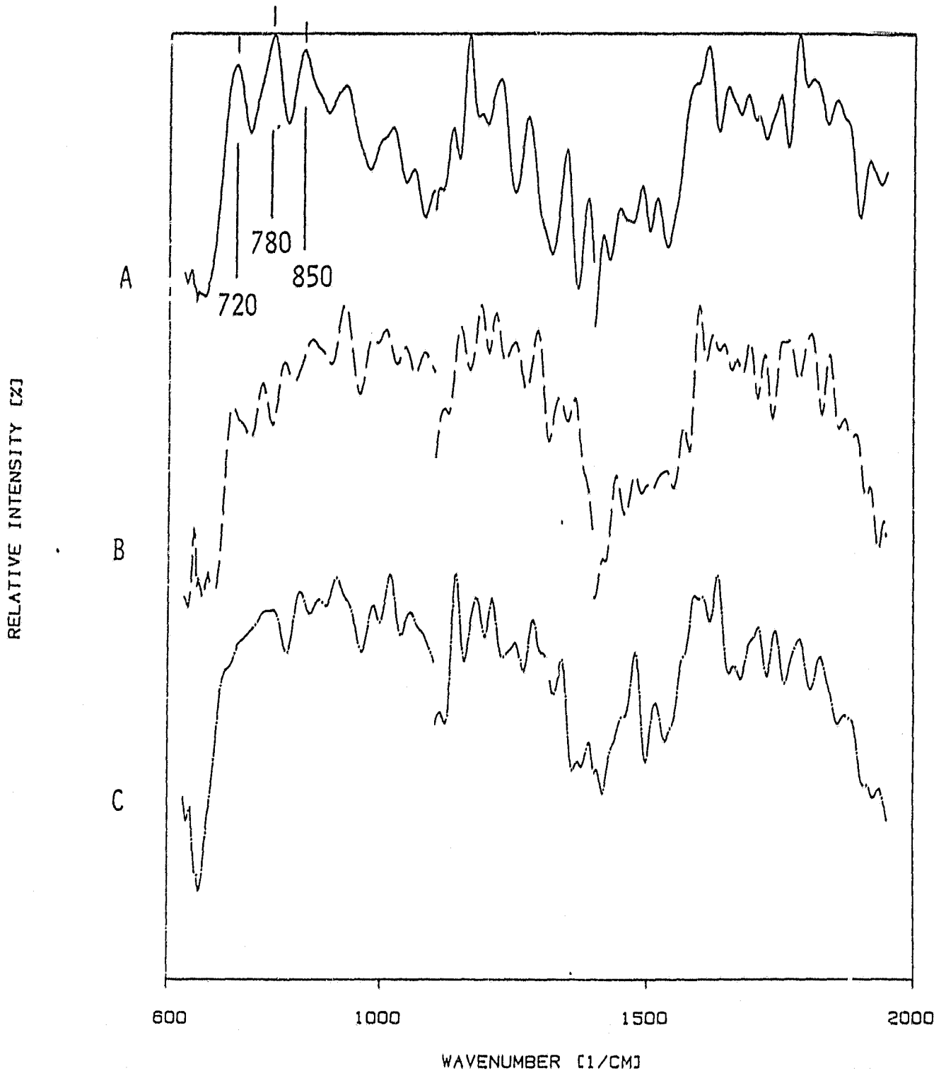
Figure 12 Emission Spectra of Jet A Fuel Deposits on MJFSR Stainless Steel Shims (A: neat fuel, B: with copper naphthenate, C: with iron naphthenate)
