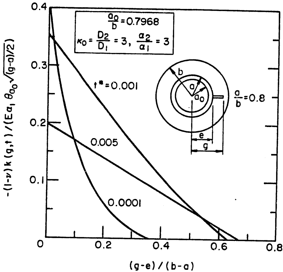
Figure 6. The normalized stress intensity factor \bar{k}(g) = -k(g,t)/E\alpha_1\theta_{a_0}\sqrt{(g-e)/2} / (1-\nu) in a reinforced cylinder which contains a crack terminating at the reinforcement-cylinder interface and which is subjected to a sudden change in the inner surface temperature ( E_1=E_2=E , \nu_1=\nu_2=\nu , (a-a_0)/(b-a) = 0.016 , the case of plane strain).
