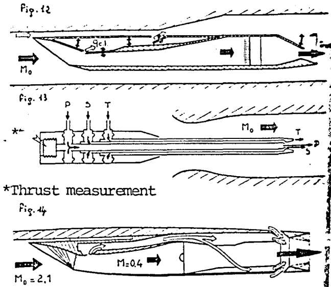
Fig. 13 - Scale for measuring in the windtunnel the thrust of multiple concentric nozzles (1964). Fig. 14 - Power nacelle sketched by the manufacturers (B.A.C. - Sud-Aviation - S.N.E.C.M.A).
