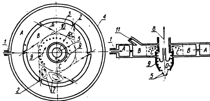
Ill. 1 A simplified schema of the pulverization process in the grinding chamber with the air-jet fluid: A--compressed gas, B--grinding zone, C--classification zone, D--separation zone: 1--compressed air lead, 2--nozzle, 3--rings, 4--external ring of the grinding chamber, 5--product collection, 6. directions of the operation of the work jets, 7--rotation in the grinding zone on the nozzle's surface, 8--outlet for the decompressed gas, 9--direction of the movement of the particles in the separation zone, 10--particles' rotating movement on the edge of the grinding and classification zones, 11--the mill's feed
