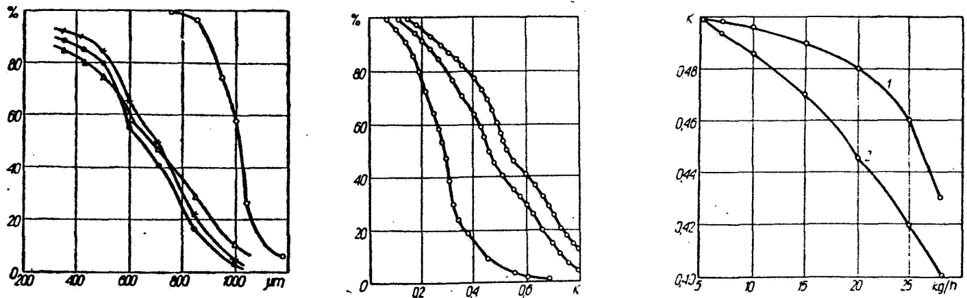
Ill. 11 The granulation of the feed and product of the pulverization of abrasive materials in a jet mill: O--feed, ●--rare electrocorundum, x--common electrocorundum, Δ--silicon carbide
