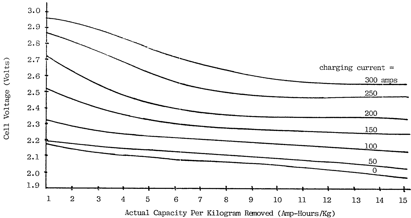
Figure F-3. Battery Cell Charging Characteristic
