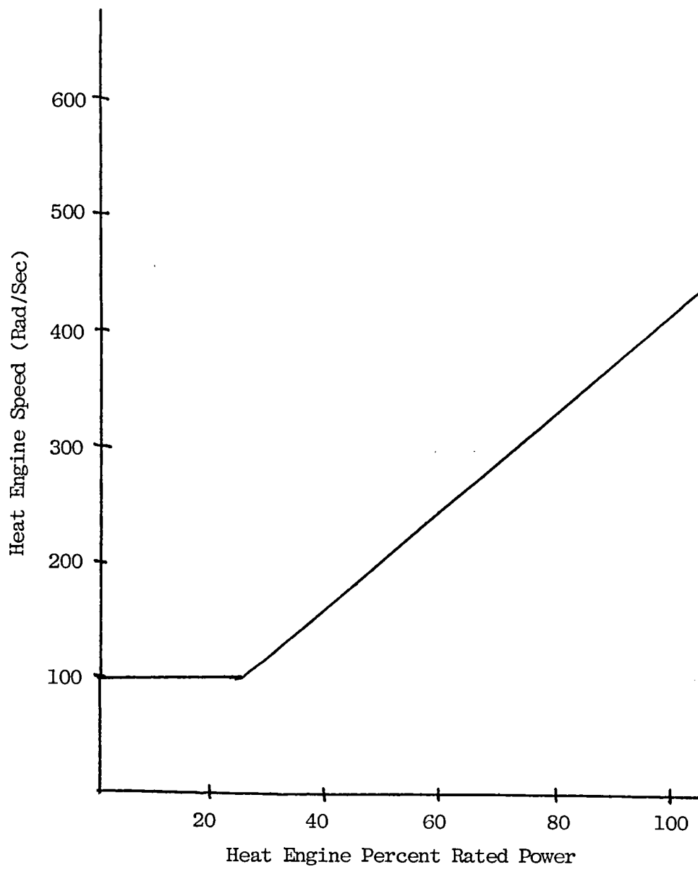
Figure G-2 Most Fuel-Efficient Engine Speed vs. Engine Output Power
