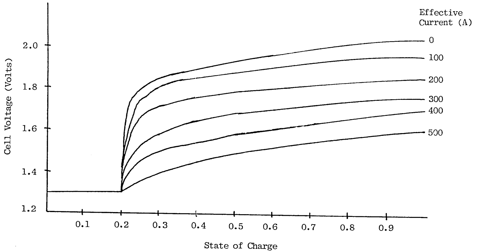
Figure F-2 Battery Discharge Characteristic
