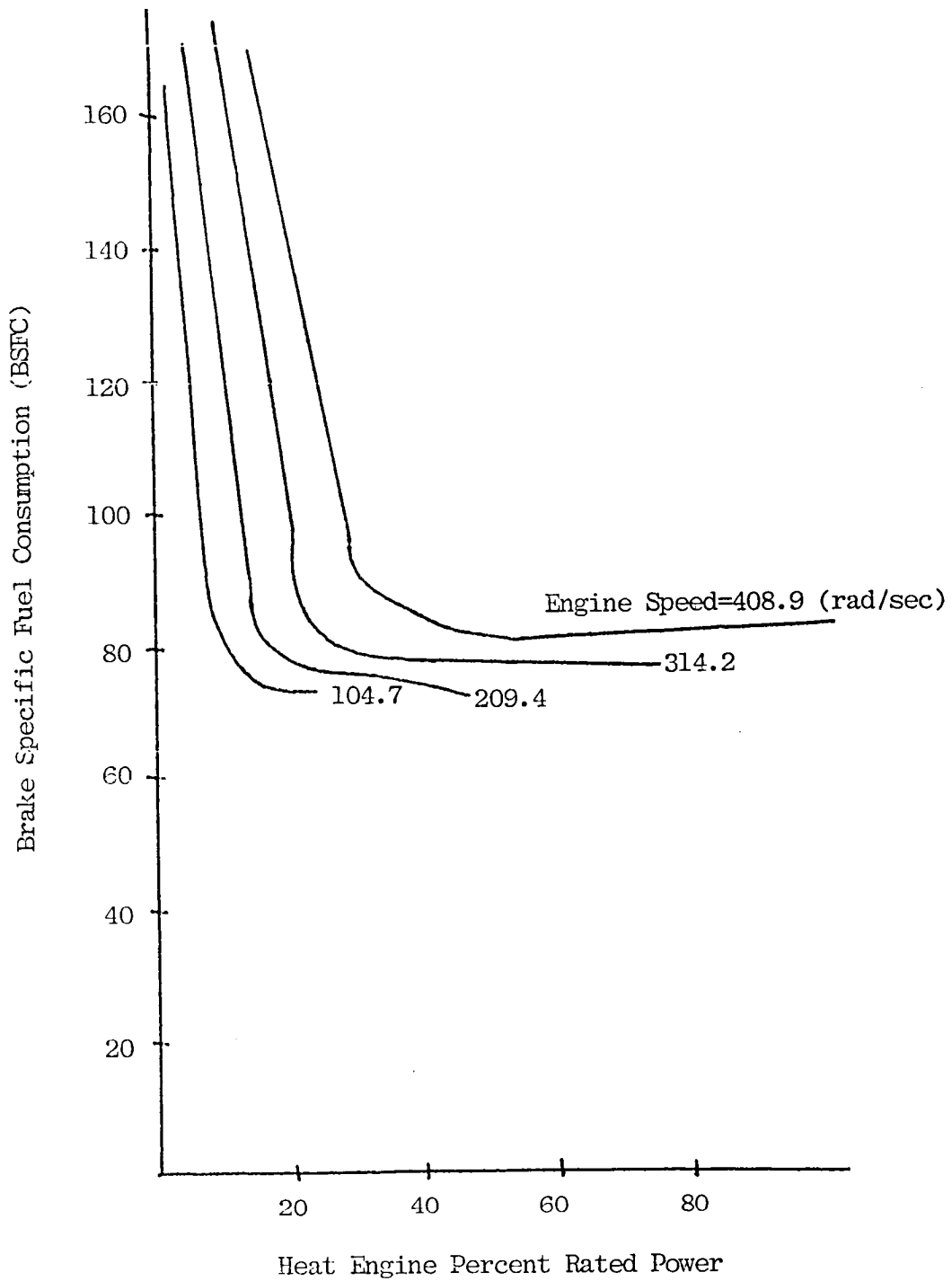
Figure G-1 Brake Specific Fuel Consumption (BSFC) Map for a 75 Kilowatt Engine
