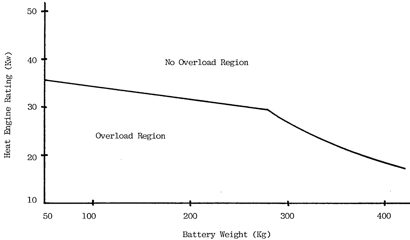
Figure 6-1. Overload Constraint Boundary
