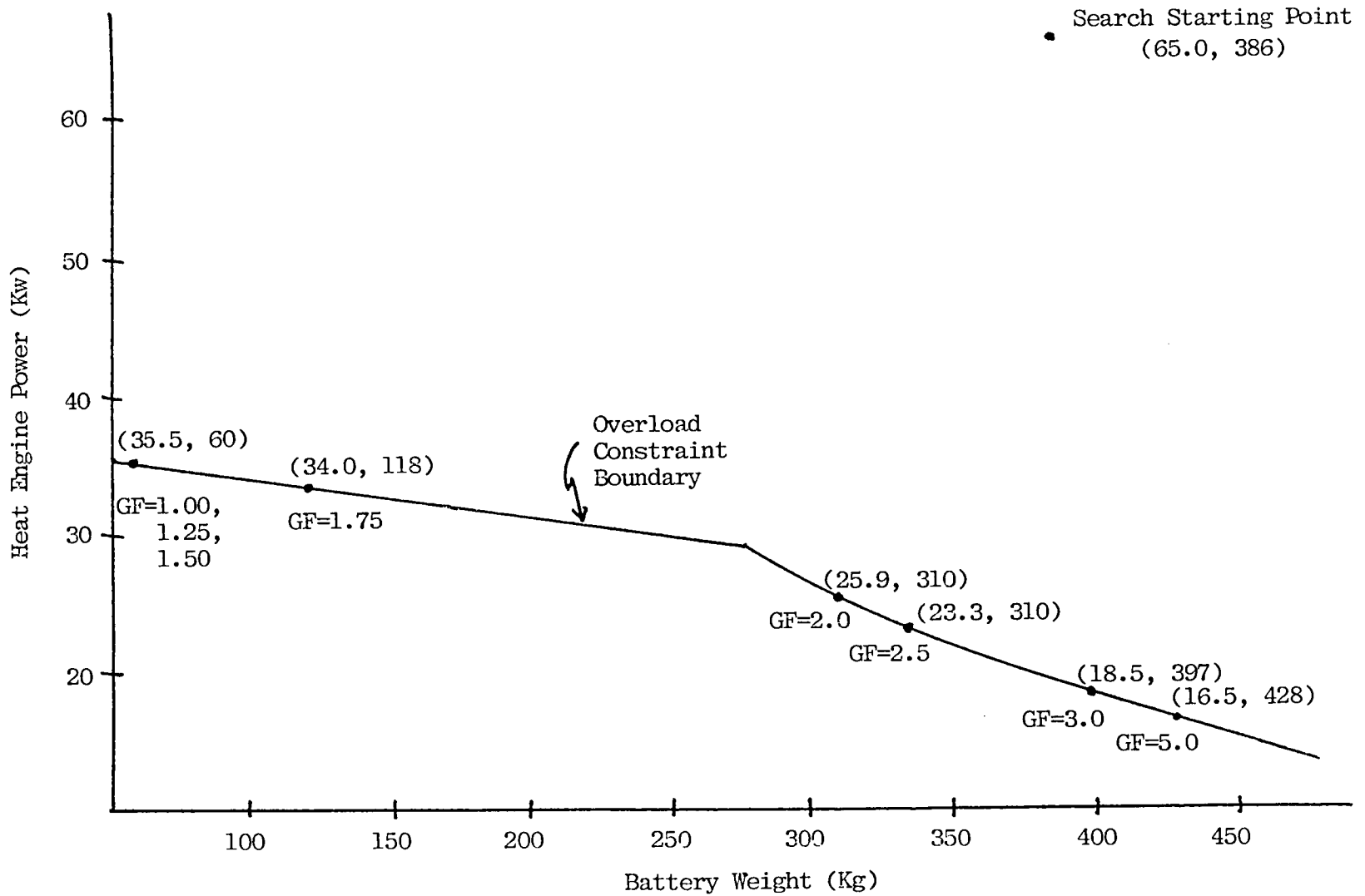
Figure 11-3 Power Source Sizing for Optimum Life Cycle Cost (Various Petroleum Costs)
