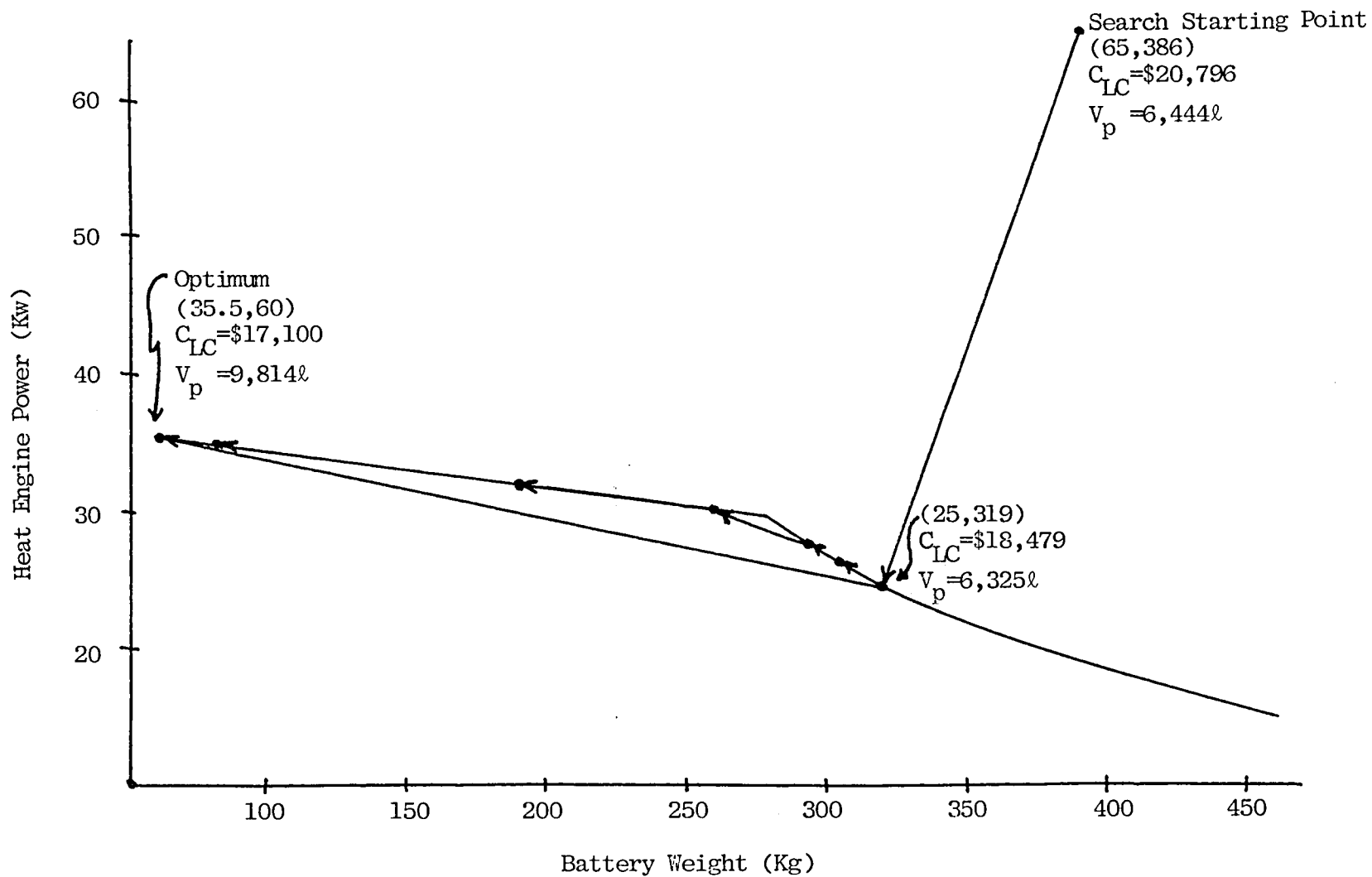
Figure 11-1 Power Source Sizing for Optimum Life Cycle Cost (Petroleum Usage Unconstrained)
