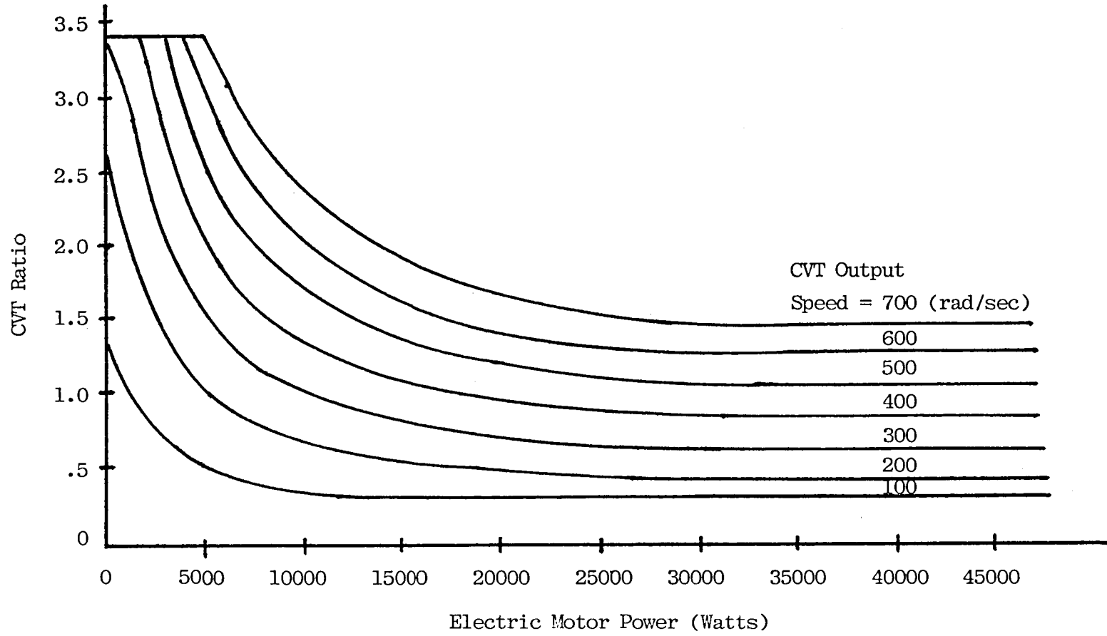
Figure G-3. CVT Ratio for Most Efficient Electric Motor Speed
