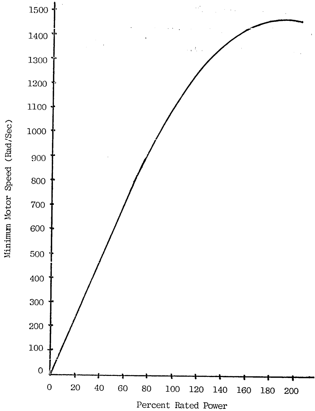
Figure G-4. Traction Motor Stall-Out Curve
