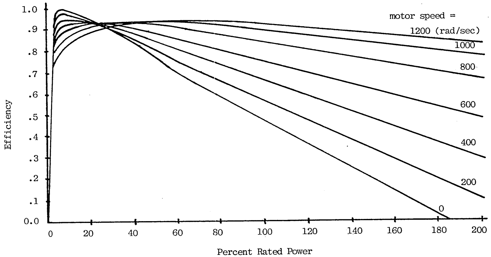
Figure E-2. Electric Motor Efficiency Map
