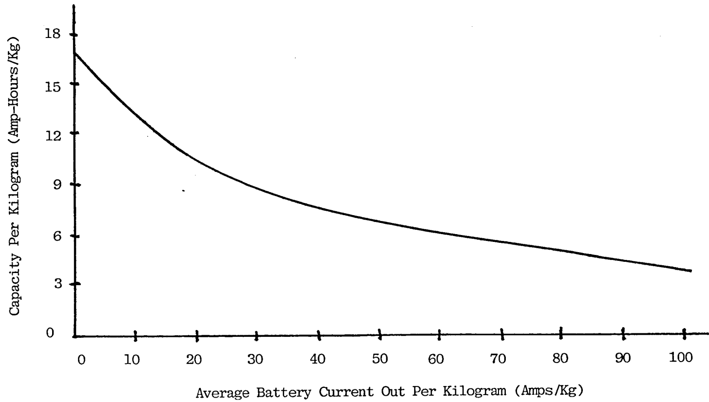
Figure F-1. Scaled Peukert Curve
