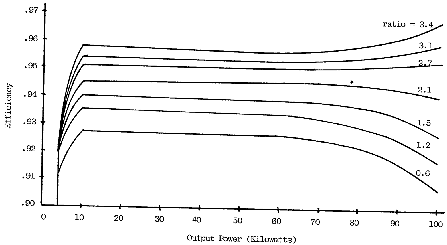
Figure E-3. CVT Efficiency Map
