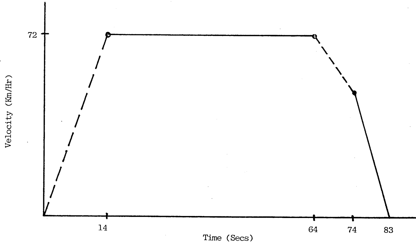
Figure 4-1. Special Test Cycle
