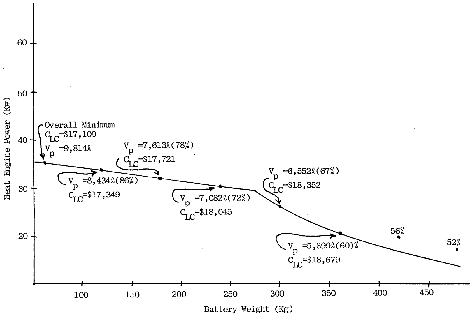
Figure 11-2 Power Source Sizing for Optimum Life Cycle Cost (Petroleum Usage Constrained)
