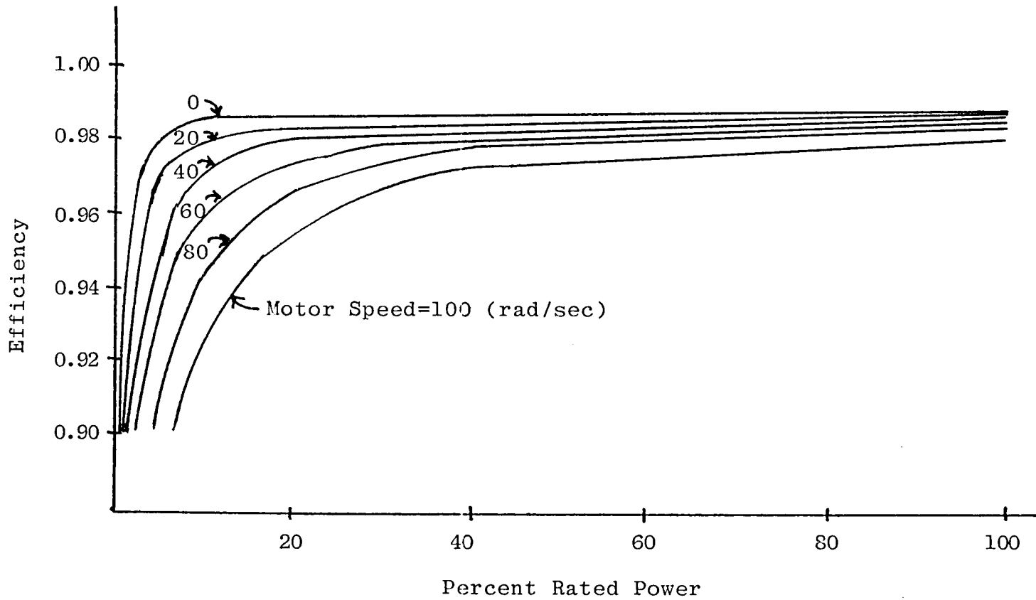
Figure E-4 Gear Efficiency Map
