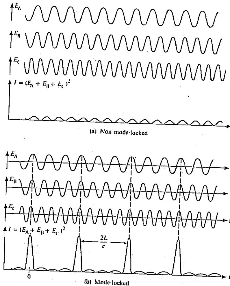
FIGURE 2-5: Comparison of non-mode-locked and mode-locked outputs. In part (a), the phases are random and the instantaneous power is never large. In part (b), all the cosine waves have the same phase at t = 0 . The narrow pulses are spaced 2L/c in time, the round-trip time for light in the cavity.
