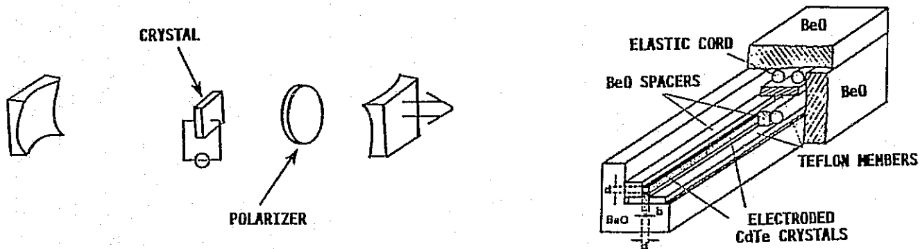
(b) INTERNAL MODULATOR USING A BIREFRINGENT CRYSTAL AND A POLARIZER.
