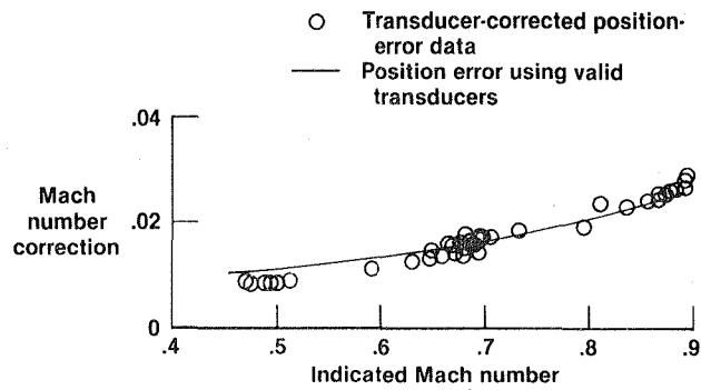
Figure 16. Comparison of corrected position error with position error determined using valid transducers.
