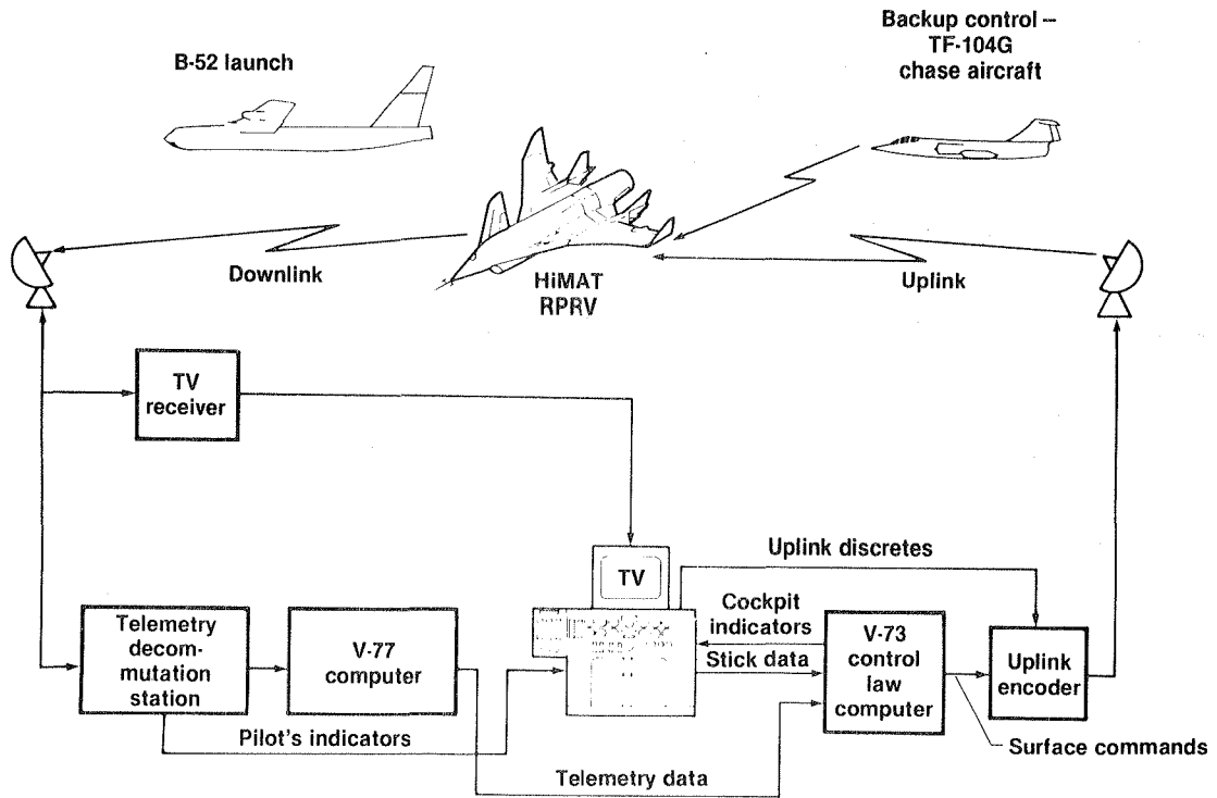
Figure 3. HiMAT RPRV control system.
