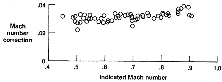
Figure 15. Original HiMAT position-error correction.
