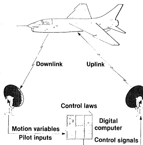
Figure 7. F-8 RAV flight test technique.
