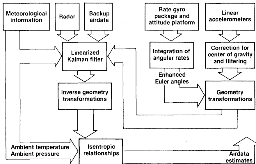
Figure 14. LKF computational scheme.
