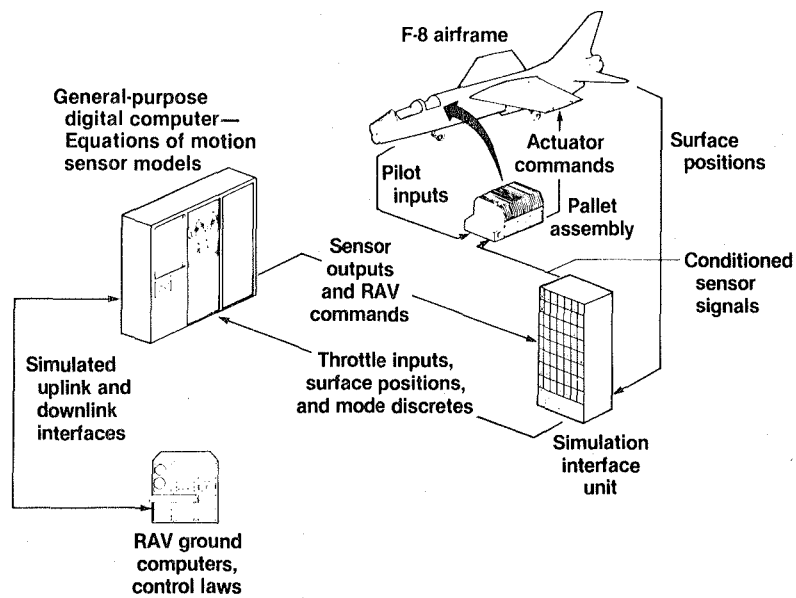
Figure 11. F-8 DFBW iron bird simulation facility configured for RAV system testing.
