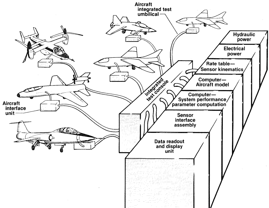
Figure 12. Integrated Test Facility.
