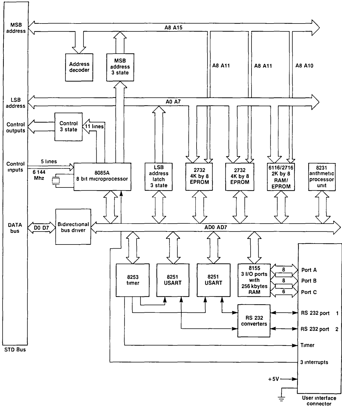
Figure 3. Simplified block diagram of a single-board microcomputer.
