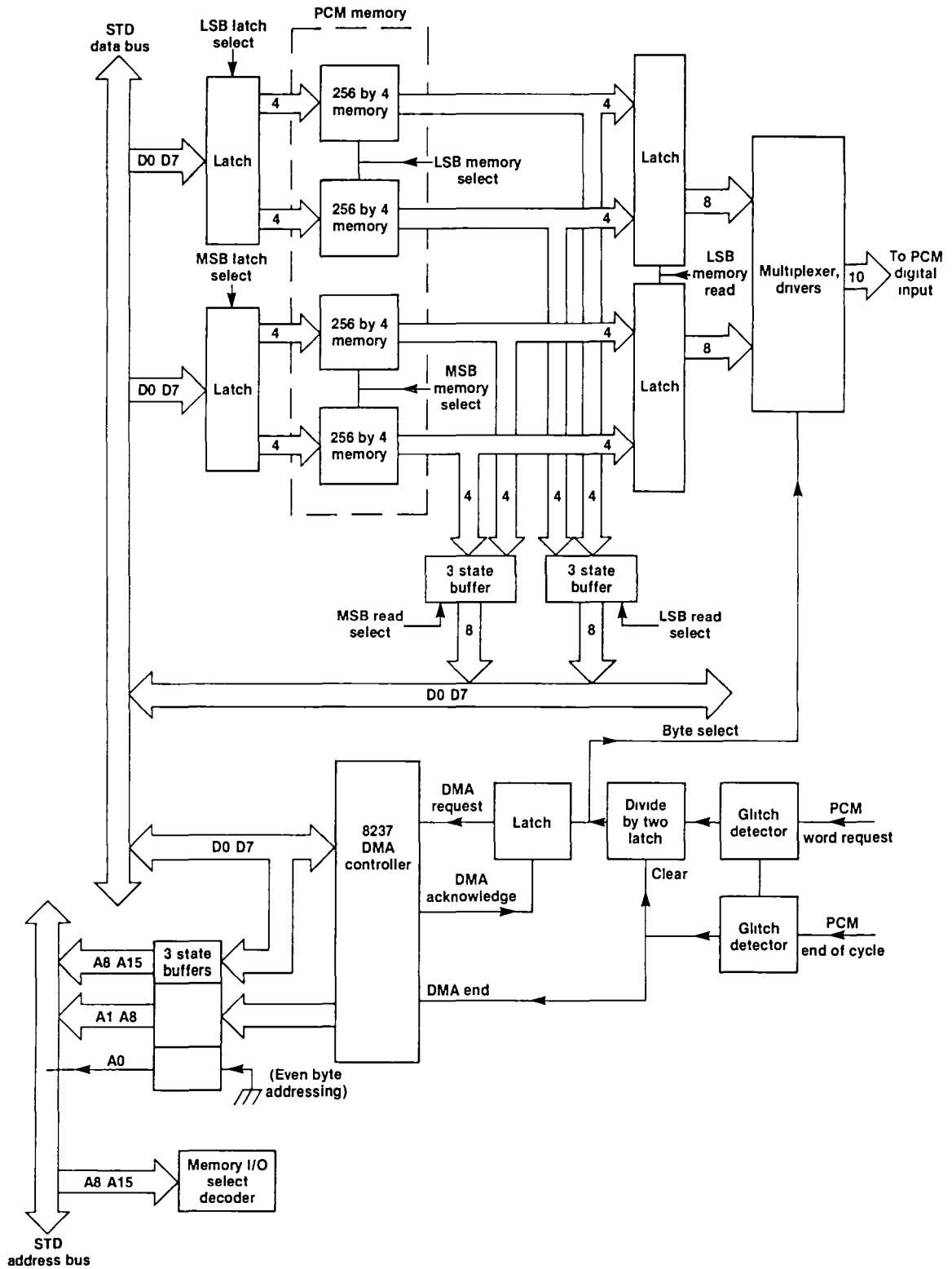
Figure 5. Simplified block diagram of a PCM interface.
