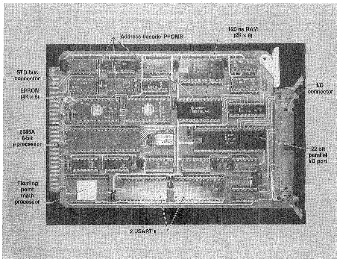
Figure 4. Single-board microcomputer.
