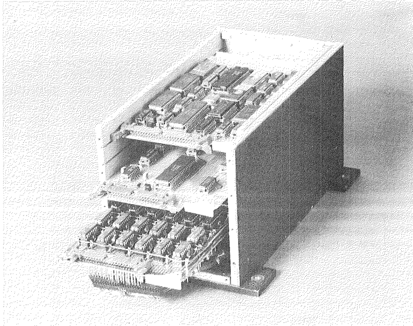
Figure 1. AICS box (DEEC prototype configuration).
