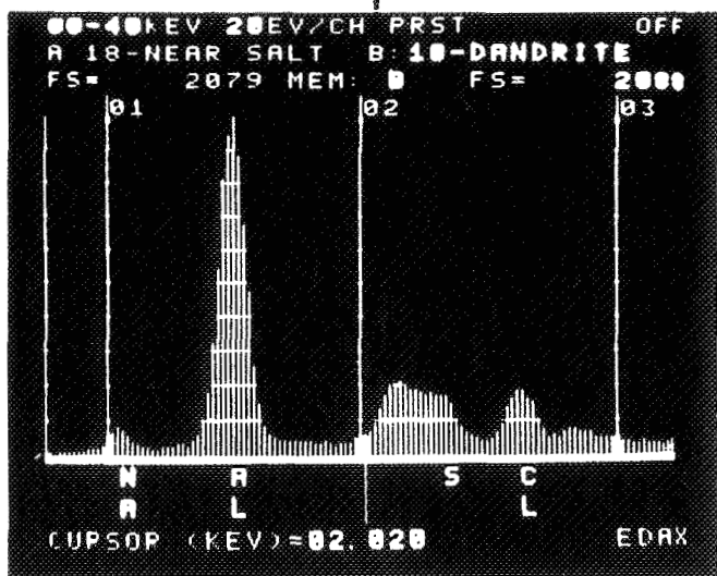
EDAX OF Al_2O_3 SUBSTRATE IN THE DENDRITE AREA; HIGH AL PEAKS.
