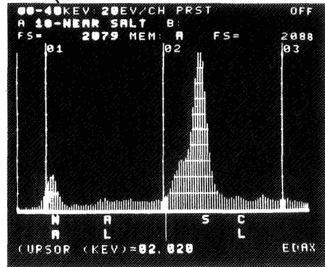
EDAX OF Al_2O_3 SUBSTRATE NEAR THE NaCl PARTICLE; HIGH SULFUR CONTENT NOTED.
