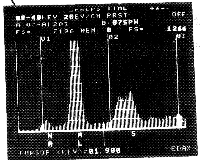
EDAX OF SULFUR-RICH GLOBULES.
