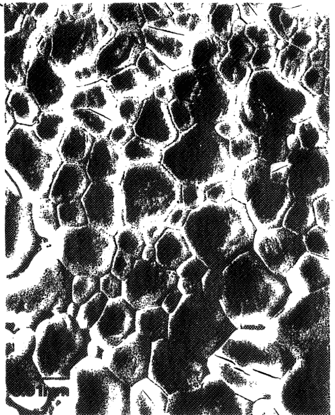
Al_2O_3 SUBSTRATE EXPOSED TO AIR AND 0.9% SO_2 AT 650^{\circ}C . FOR FOUR HOURS.
