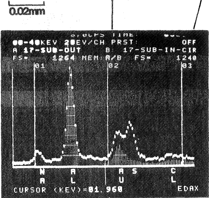
EDAX OF Al_2O_3 SUBSTRATE; COMPARES ELEMENTAL COM- PONENTS OF THE INNER AND OUTER RINGS.
