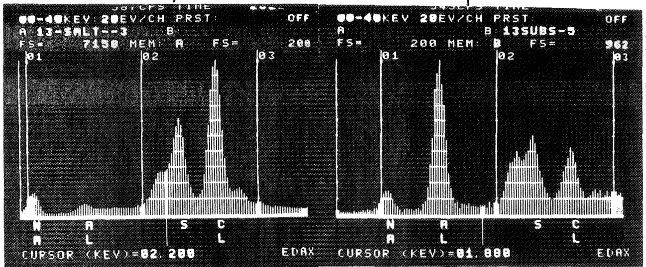
NaCl PARTICLE EXPOSED TO AIR PLUS 0.99% SO 2 AT 600 0 C. FOR 10 MINUTES.
