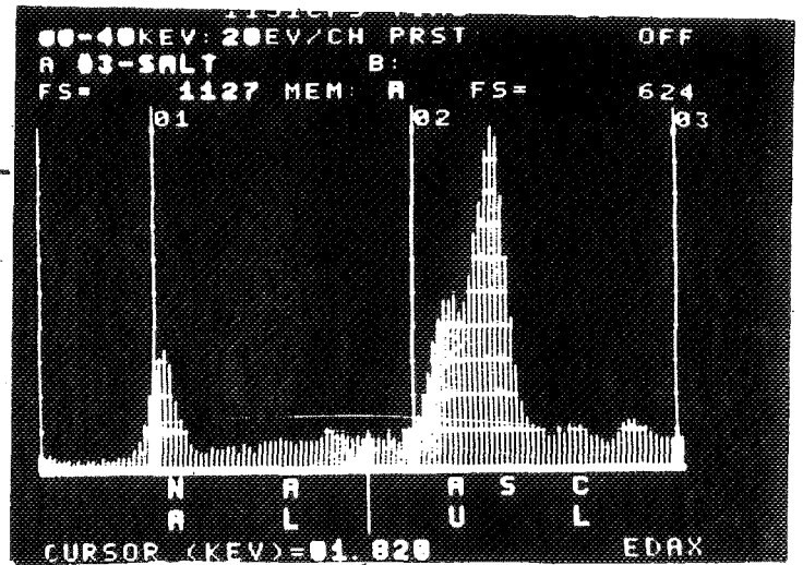
NaCl PARTICLE EXPOSED TO AIR AND 0.2% SO 2 AT 600° C. FOR TWO HOURS.
