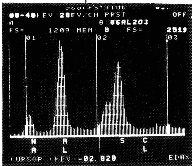
EDAX OF Al_2O_3 SUBSTRATE; NO CHLORINE 3 PEAK.
