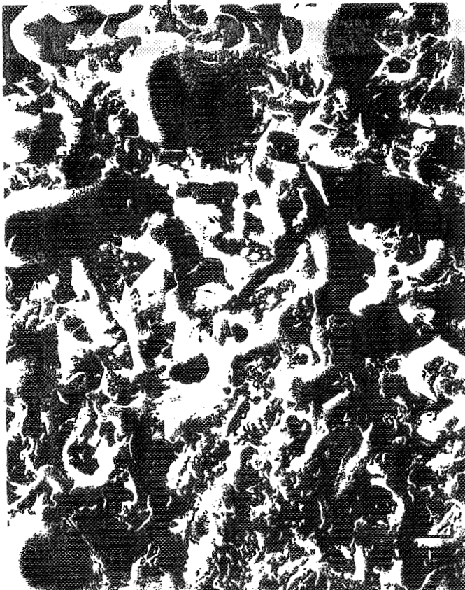
Al_2O_3 SUBSTRATE EXPOSED TO AIR AND 0.9% SO_2 AT 650^{\circ}C . FOR FOUR HOURS.
