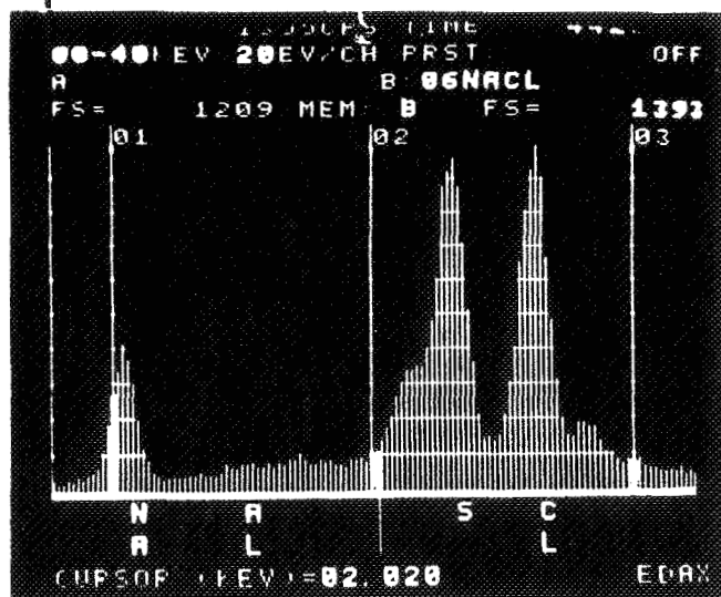
EDAX OF NA 2 CL PARTICLE; SULFUR AND CHLORINE PRESENT.
