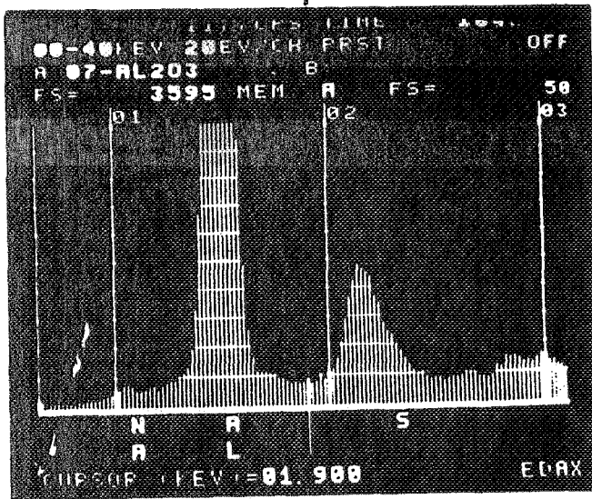
EDAX OF Al_2O_3 SUBSTRATE.
