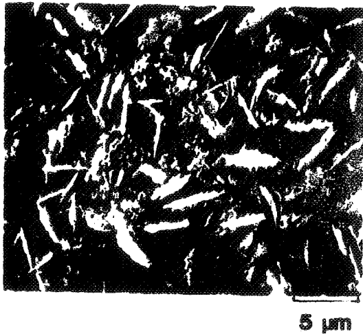
FIGURE 41 \text{Al}_2\text{O}_3 surface after removal of water soluble salts shows evidence of attack by the liquid eutectic at temperature, but no attack below the solid deposits.
