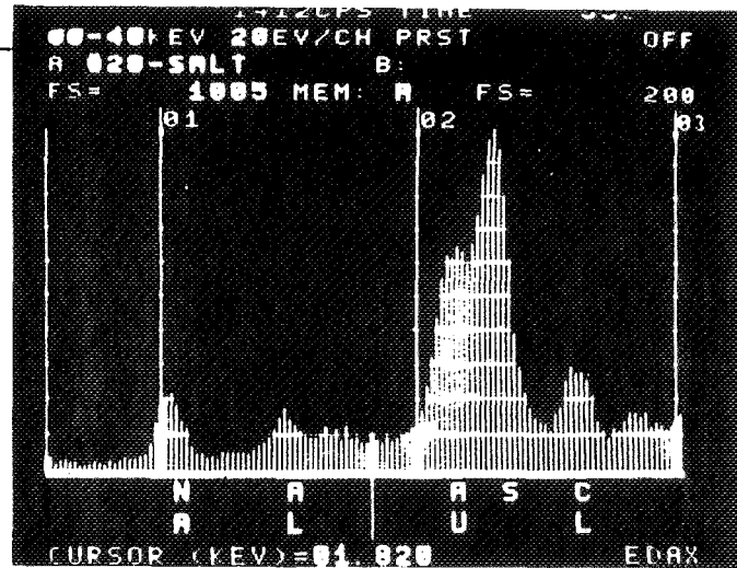
NaCl PARTICLE EXPOSED TO AIR, 0.2% SO 2 AND 1.0% H 2 O AT 500 0 C. FOR FOUR HOURS.
