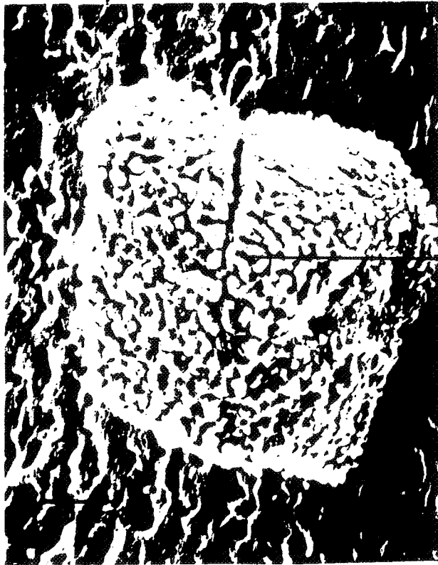
FIGURE 16 NaCl particle exposed to air + 1%SO 2 at 600°C for 30 min.
