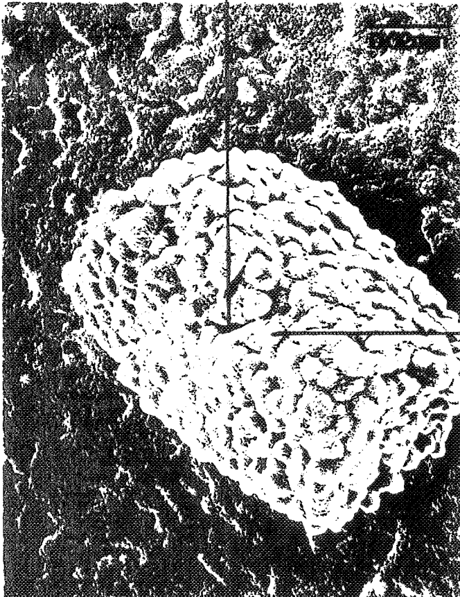
NaCl PARTICLE EXPOSED TO AIR AND 0.2% SO 2 AT 600° C. FOR TWO HOURS.
