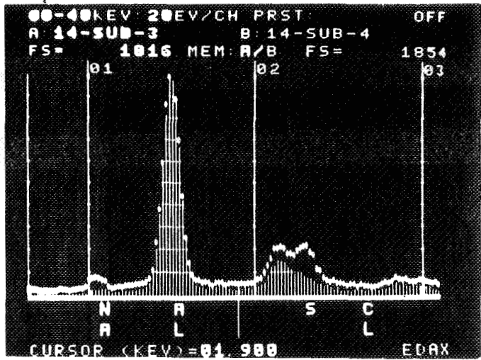
EDAX OF AL 2 O 3 SUBSTRATE; SULFUR CONTENT PRESENT.
