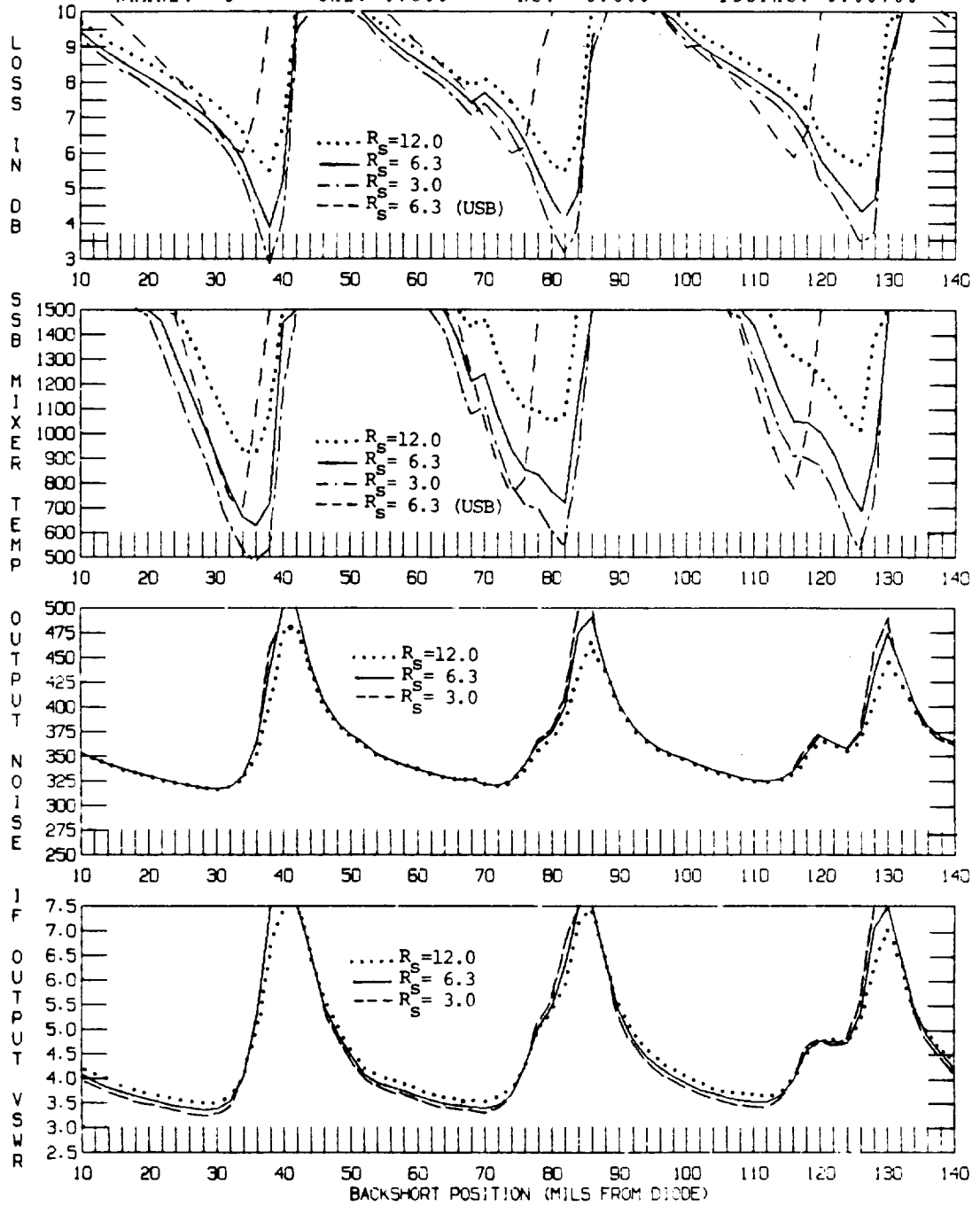
Fig. 5-4 Computed mixer performance at 180 GHz when R_s(\text{dc}) = 3, 6.3 and 12 ohms. In the top two graphs only the lower sidebands are compared (except for the plain dashed line which represents the upper sideband performance for R_s(\text{dc}) = 6.3 , our standard value).
