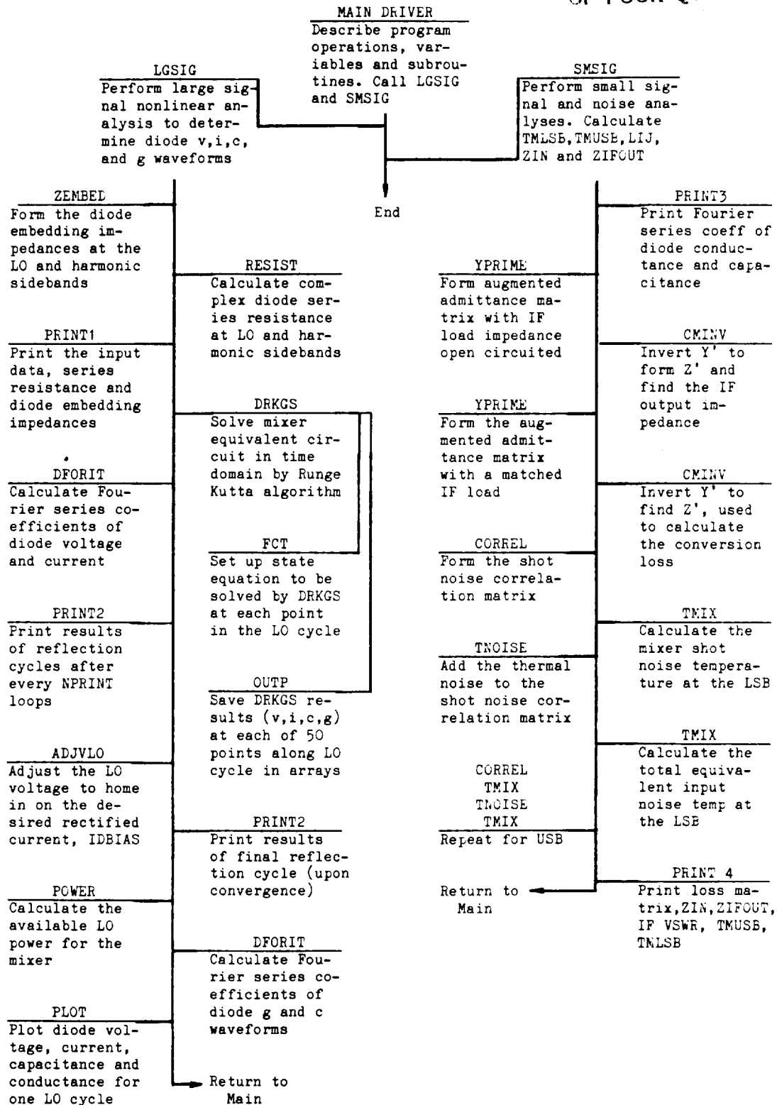
Fig. 2-10 Flow diagram of the mixer analysis program.
