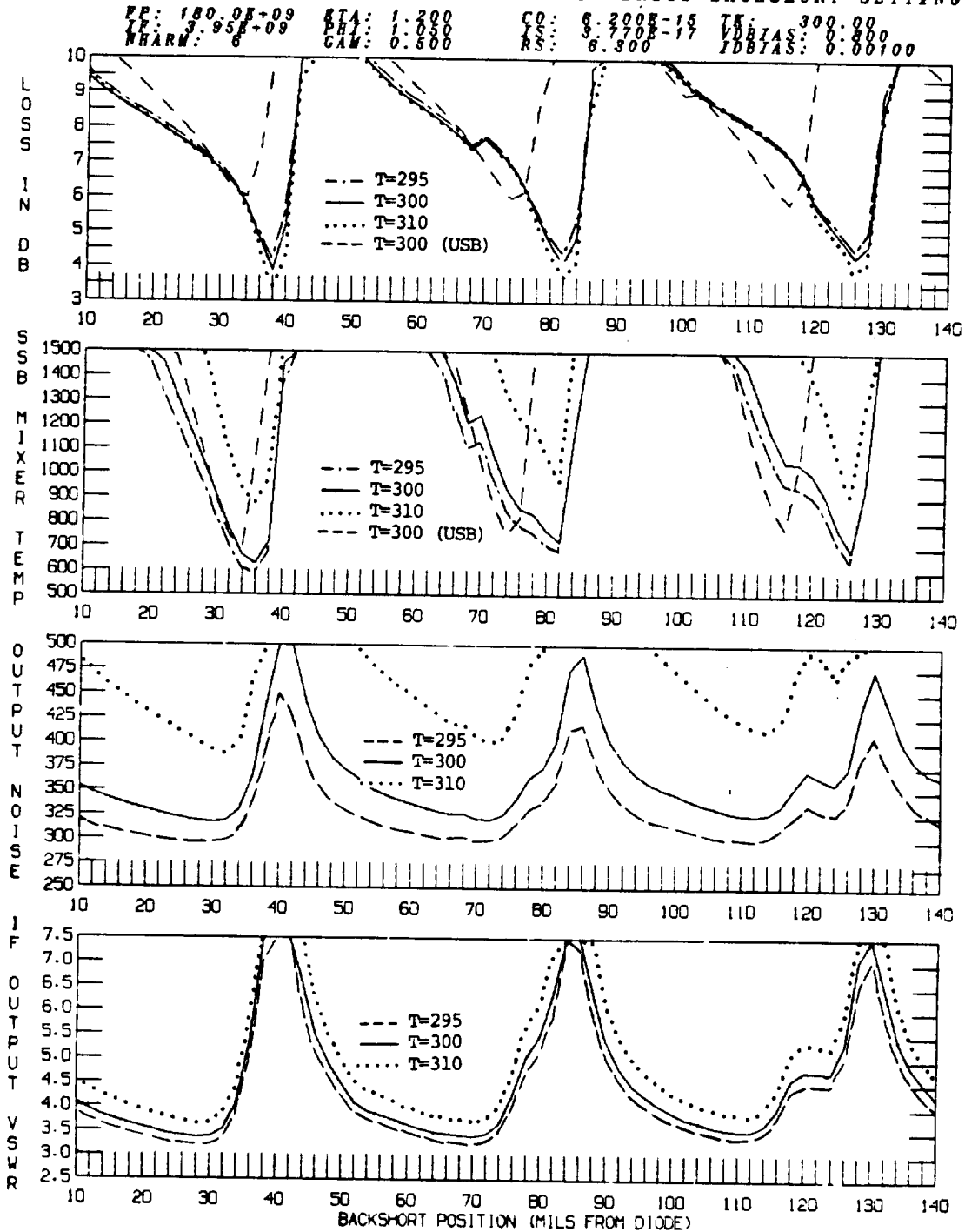
Fig. 5-5 Computed mixer performance at 180 GHz when T = 295, 300 and 310 K. In the top two graphs only the lower sidebands are compared (except for the plain dashed line which represents the upper sideband performance for T = 300 K, our standard value).
