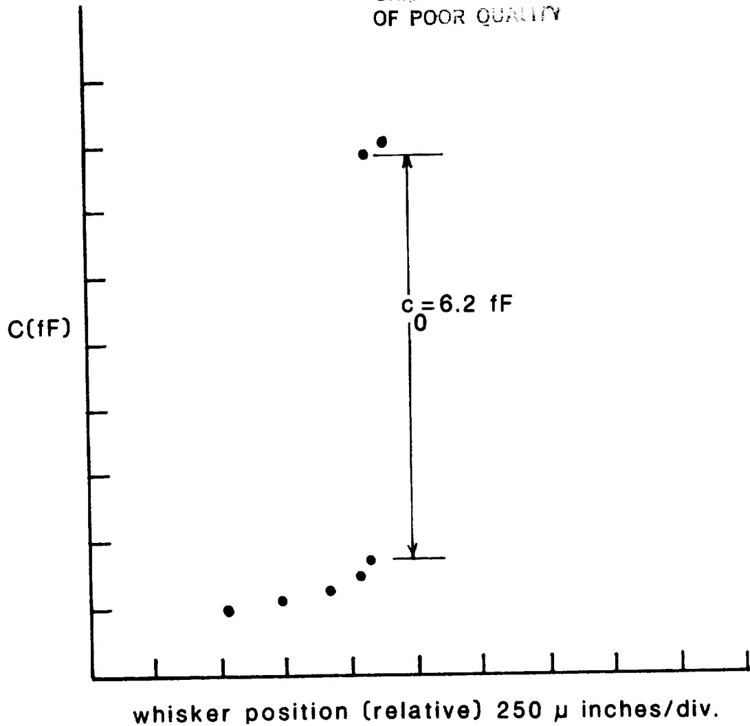
Fig. 4-8 A plot of the relative capacitance versus whisker position during the diode contacting procedure. As the whisker is advanced towards the diode the capacitance between the body of the diode chip and the whisker and mixer block (grounded) increases. At contact, the diode junction capacitance is added in parallel with the fringing capacitance and the measured value jumps by c_0 . A Boonton model 75D 1 MHz capacitance bridge with a resolution of 0.05 fF is used for the measurement.
