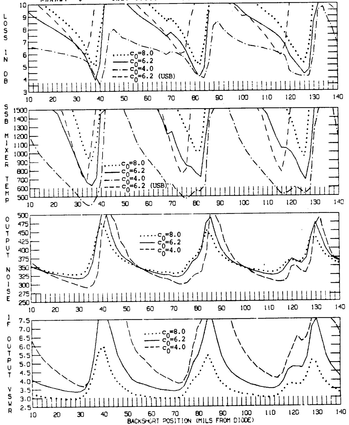
Fig. 5-6 Computed mixer performance at 180 GHz when c_0 = 4, 6.2 and 8 fF. In the top two graphs only the lower sidebands are compared (except for the plain dashed line which represents the upper sideband performance for c_0 = 6.2 fF, our standard value).
