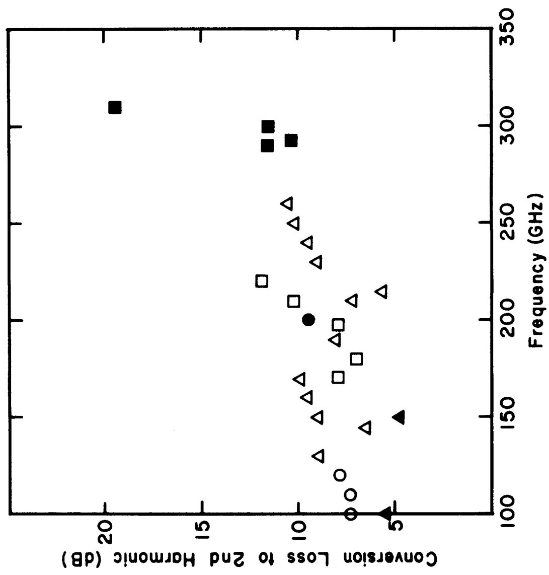
Fig. 6-3 Reported conversion efficiencies for varactor diode doublers with outputs between 100 and 350 GHz.
