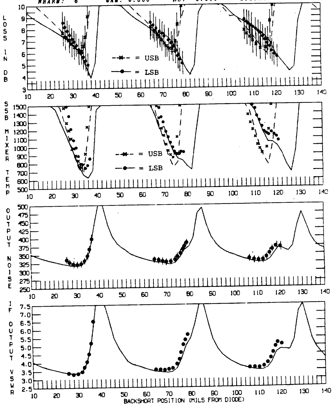
Fig. 4-10 A comparison of the measured (points) and computed (lines) mixer performance at 180 GHz. Error bars reflect uncertainties in the input signal power level and in the IF readings (error bars for the input noise temperature are typically +400,-200K and are not shown).
