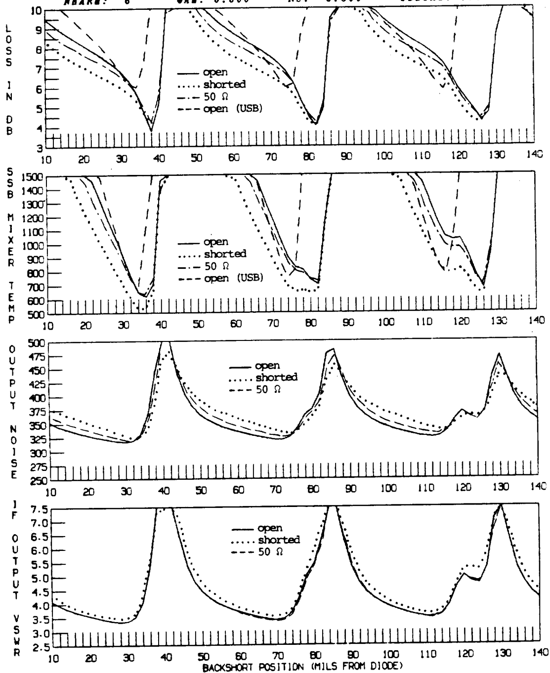
Fig. 5-11 Computed mixer performance at 180 GHz when the embedding impedances are (a) open circuited, (b) short circuited and (c) set to 50 ohms above the upper sideband. Curves (a) are indistinguishable from the standard run (Fig. 4-11). In the top two graphs only the lower sidebands are compared (except for the plain dashed line which represents the upper sideband performance for Z_e open circuited).
