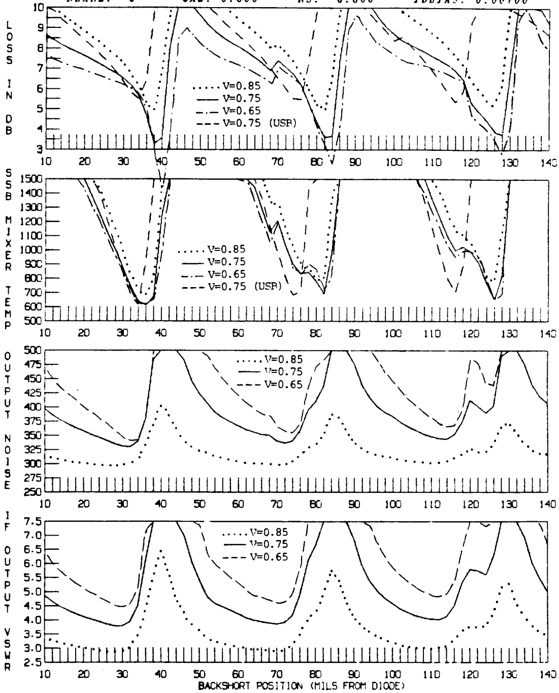
Fig. 5-9 Computed mixer performance at 180 GHz when VDBIAS = .65, .75 and .85 V. In the top two graphs only the lower sidebands are compared (except for the plain dashed line which represents the upper sideband performance for VDBIAS = 0.75).
