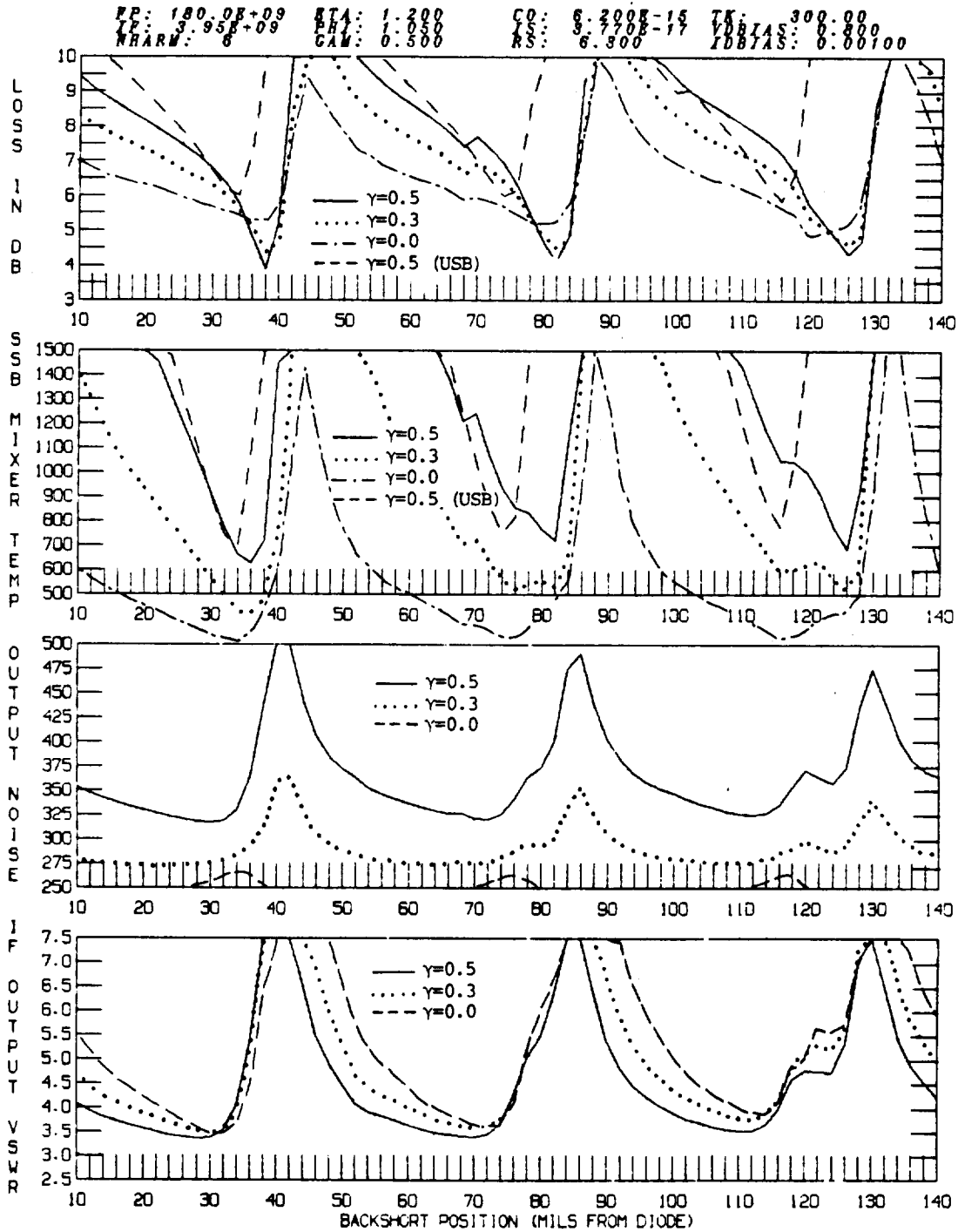
Fig. 5-3 Computed mixer performance at 180 GHz when \gamma = 0.0, 0.3 and 0.5 . In the top two graphs only the lower sidebands are compared (except for the plain dashed line which represents the upper sideband performance for \gamma = 0.5 , our standard value).
