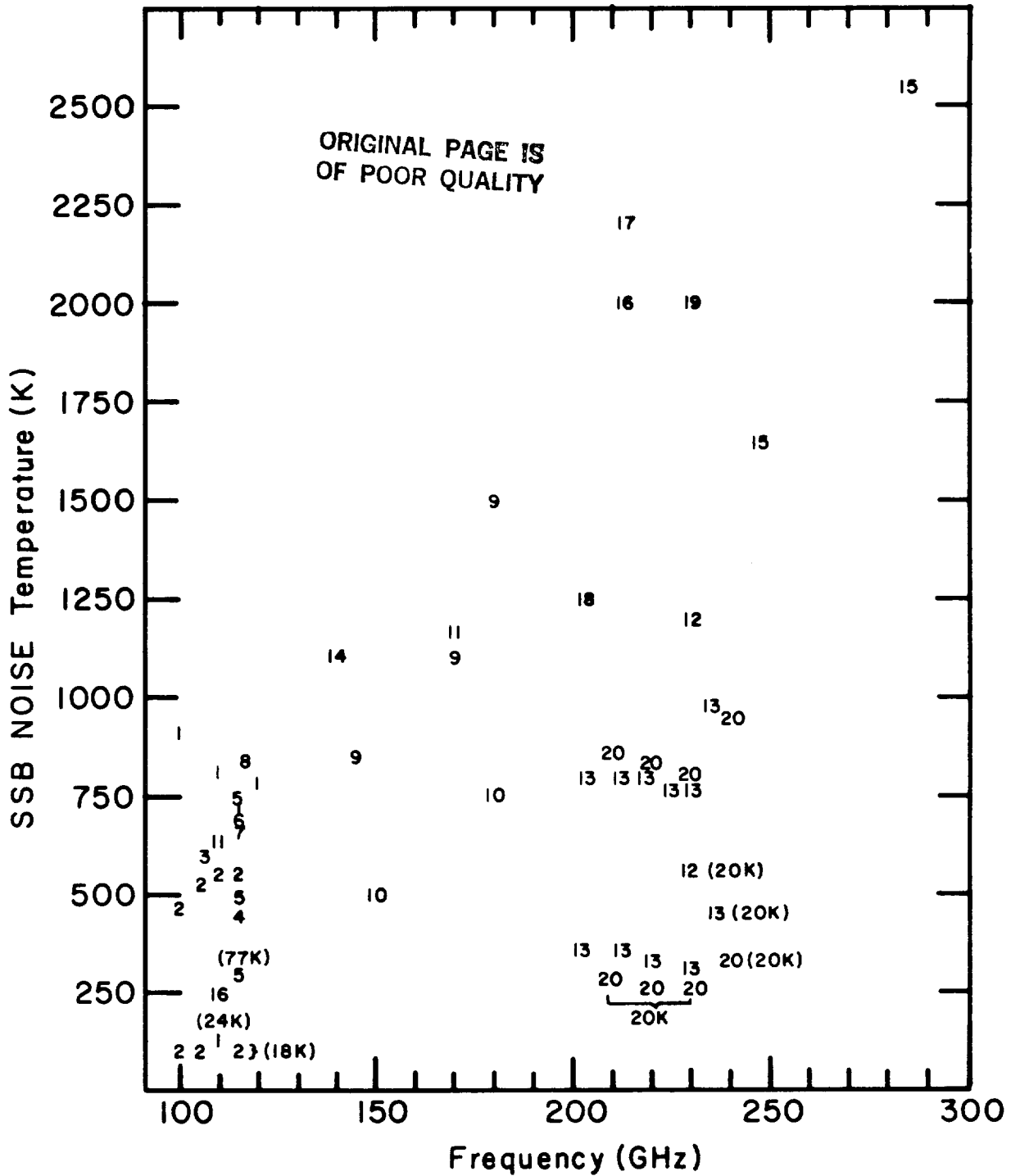
Fig. 1-2 Reported single sideband noise temperatures of fundamental Schottky barrier diode mixers in the 100-300 GHz region. References for the plotted points are given in the list in Fig. 1-1. All results are for room temperature unless otherwise indicated.
