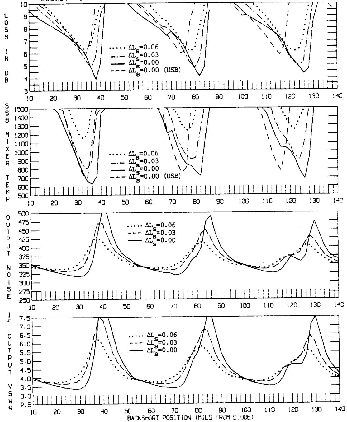
Fig. 5-12 Computed mixer performance at 180 GHz when the diode contact whisker length is increased ( \Delta L_s = 0.0, 0.03 and 0.06 nH). In the top two graphs only the lower sidebands are compared (except for the plain dashed line which represents the upper sideband performance for our standard diode).
