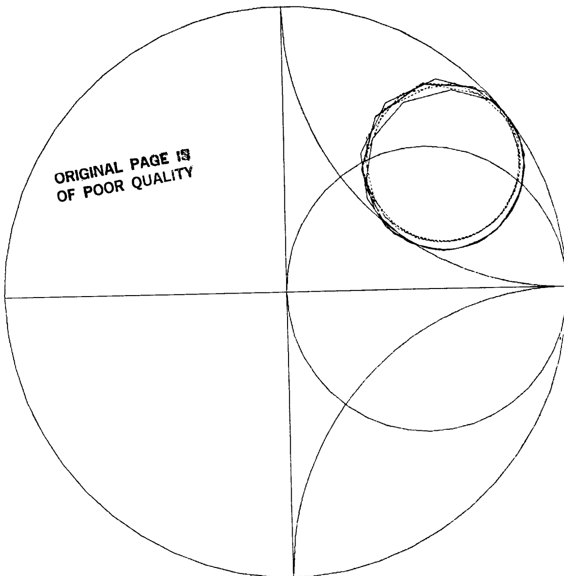
Fig. 3-8 The measured (solid line) and corrected (dashed line) diode embedding impedances as a function of backshort position at an LO frequency of 180 GHz. The dashed line shows the impedances corrected for waveguide loss and for capacitive and inductive differences between the mixer and the scale model.
