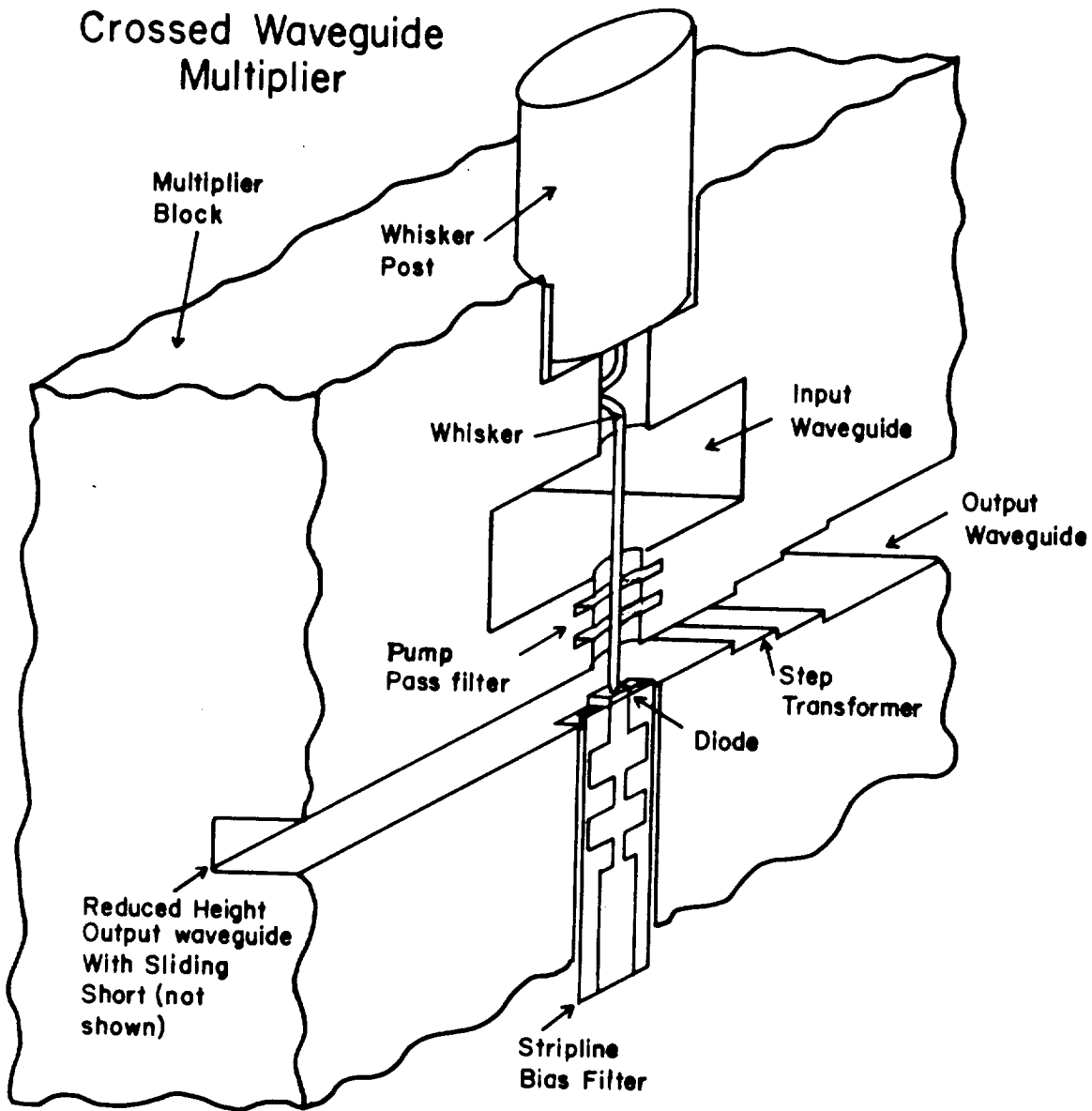
Fig. 6-1 Isometric view of a hypothetical crossed waveguide multiplier in the region near the diode. Only one half of a split-block structure is shown. The region between the input and output waveguides contains a coaxial pump-pass filter. The diode is bonded to a low pass stripline filter which allows DC biasing of the diode. Sliding shorts in each waveguide (not illustrated) can be used for tuning. A step transformer is included in the output waveguide for reducing the guide impedance to a value which more closely matches the input impedance of the diode.
