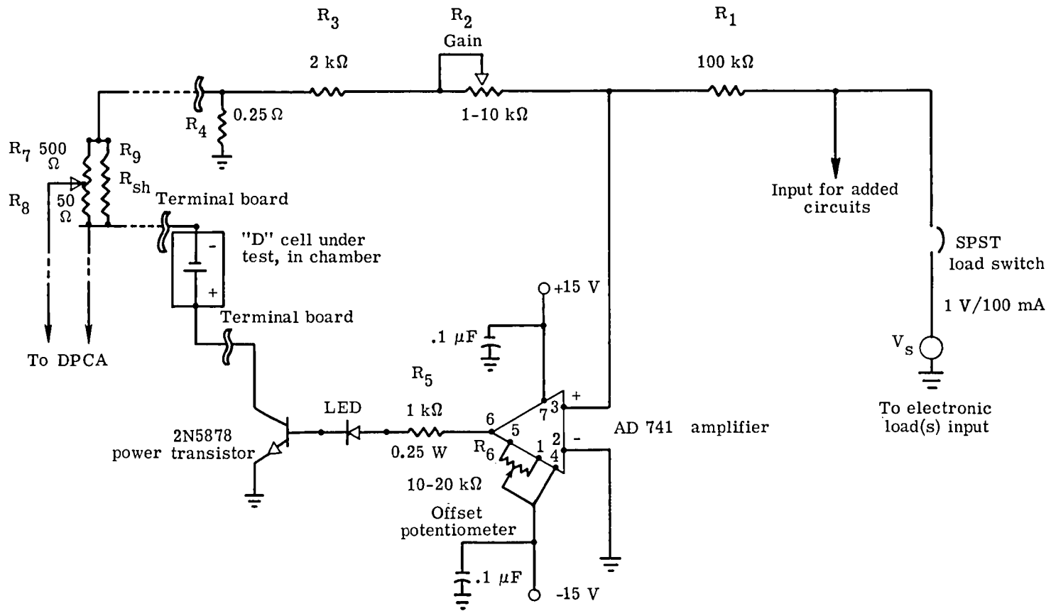
Figure A1.- ELT alkaline battery cell constant-current load circuit.
