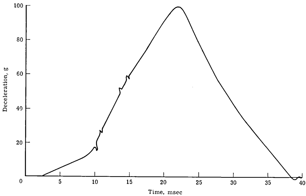
Figure 20.- Shock spectrum to which alkaline cells were exposed.
