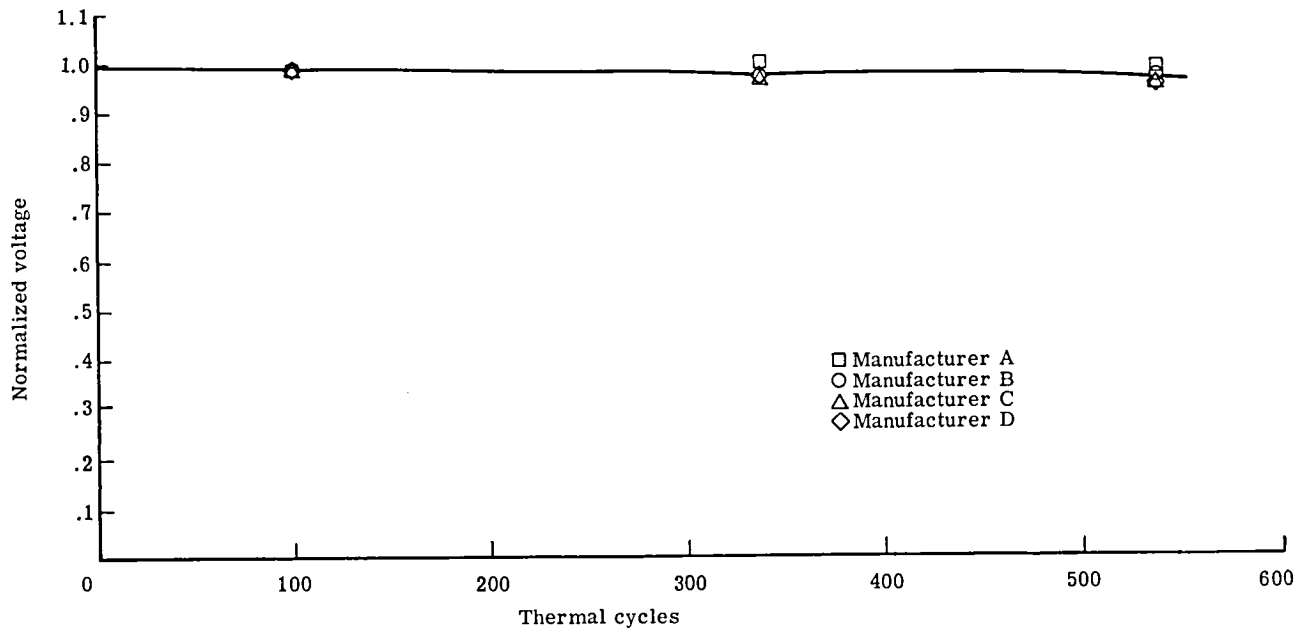
Figure 17.- Effect of thermal cycling on open-circuit voltage of alkaline cells.
