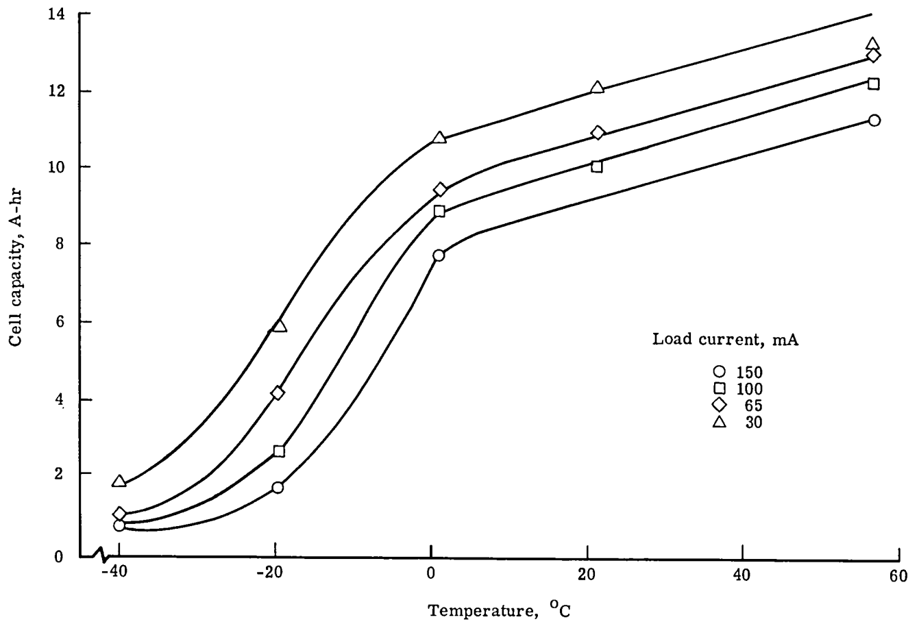
Figure 6.- Effect of temperature on capacity (0.9-V cutoff voltage) for cells from manufacturer A.
