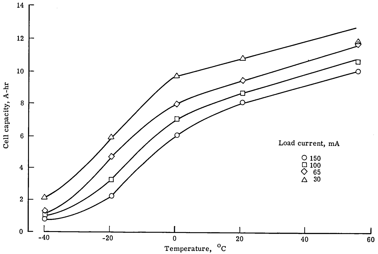
Figure 12.- Effect of temperature on capacity (0.9-V cutoff voltage) for cells from manufacturer C.
