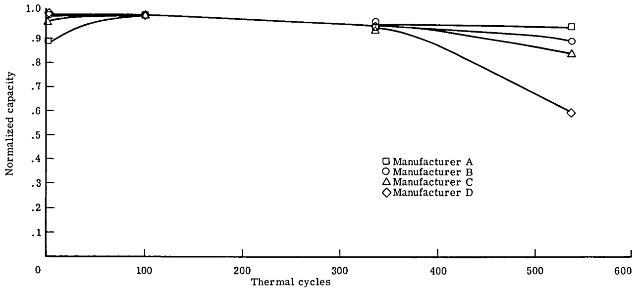
Figure 18.- Effect of thermal cycling on capacity of alkaline cells.
