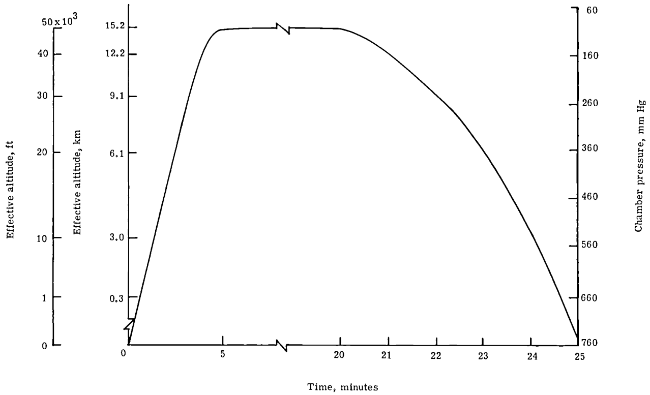
Figure 19.- Test chamber pressure profile for high-altitude exposure tests on alkaline battery cells.
