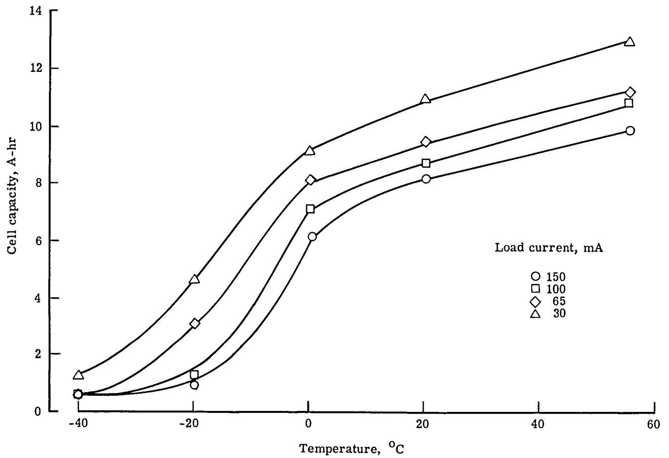
Figure 9.- Effect of temperature on capacity (0.9-V cutoff voltage) for cells from manufacturer B.
