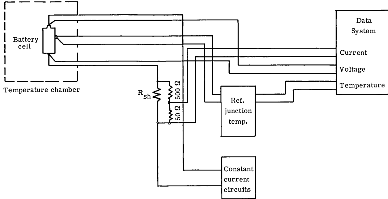
Figure 1.- Block diagram of basic test setup.
