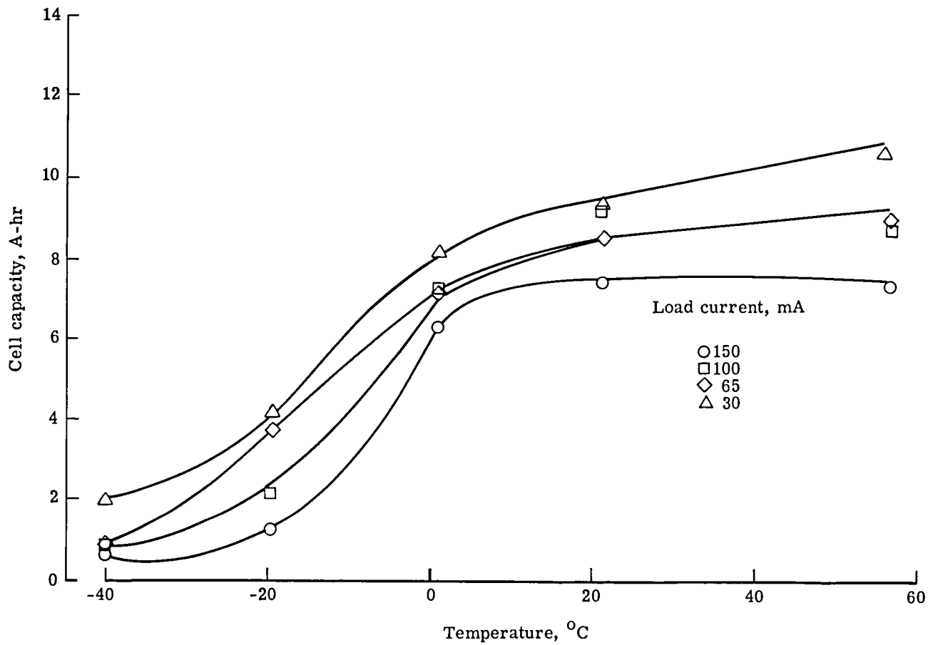
Figure 15.- Effect of temperature on capacity (0.9-V cutoff voltage) for cells from manufacturer D.
