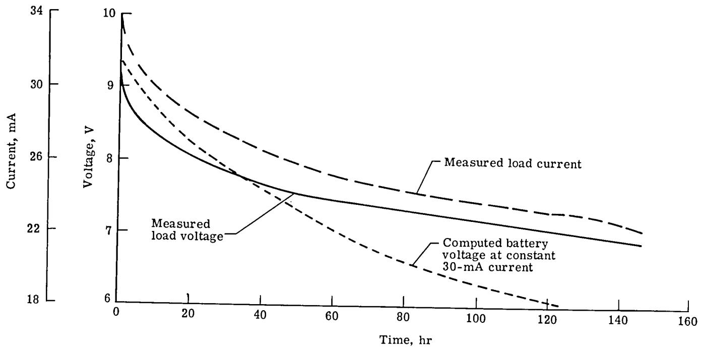
Figure 22.- Measured and computed voltage curves and measured current curve for an ELT powered by a battery made of cells from manufacturer B. T = -20^{\circ}\text{C} .
