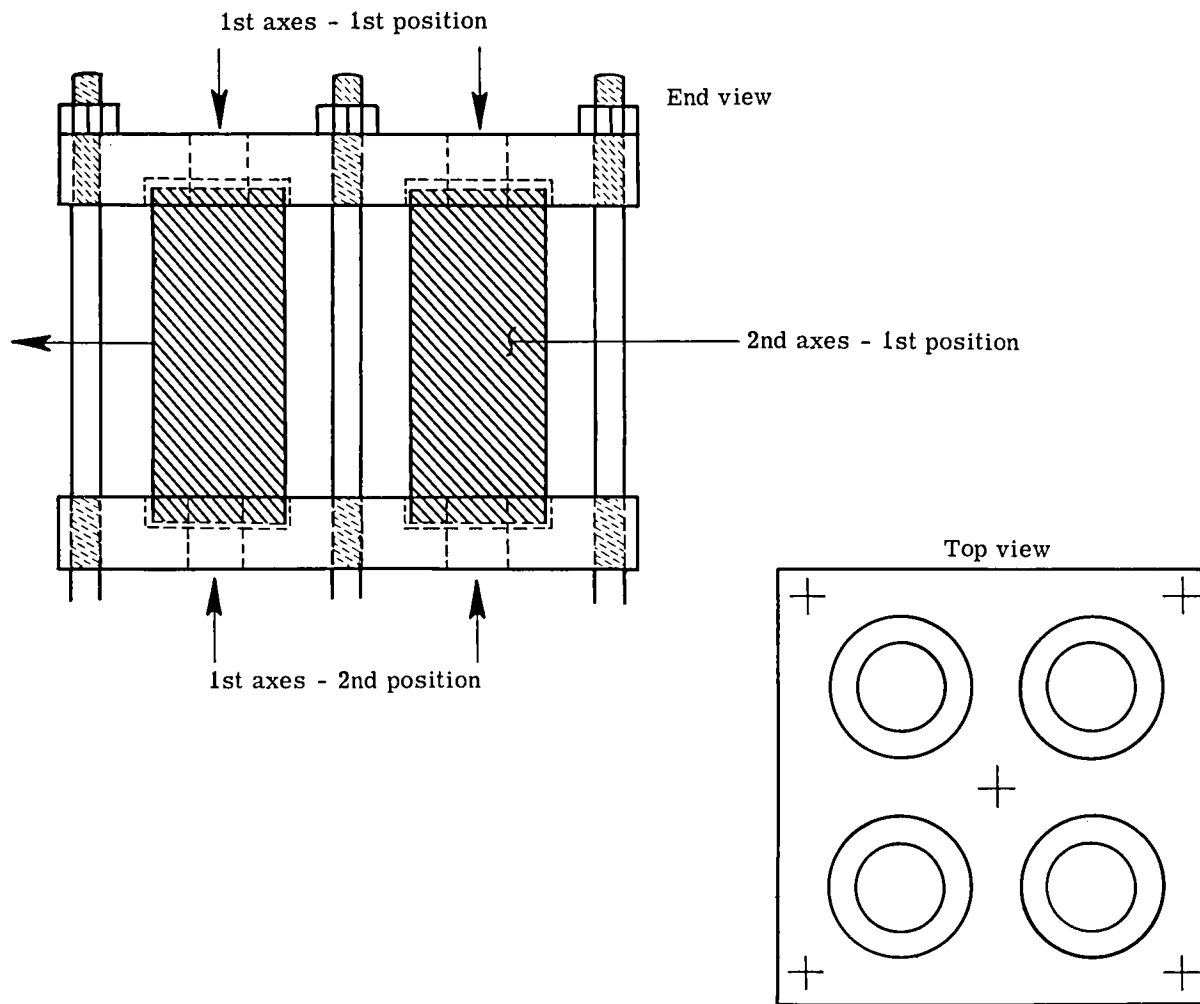
Figure 2.- Cells mounted in holders for shock tests.
