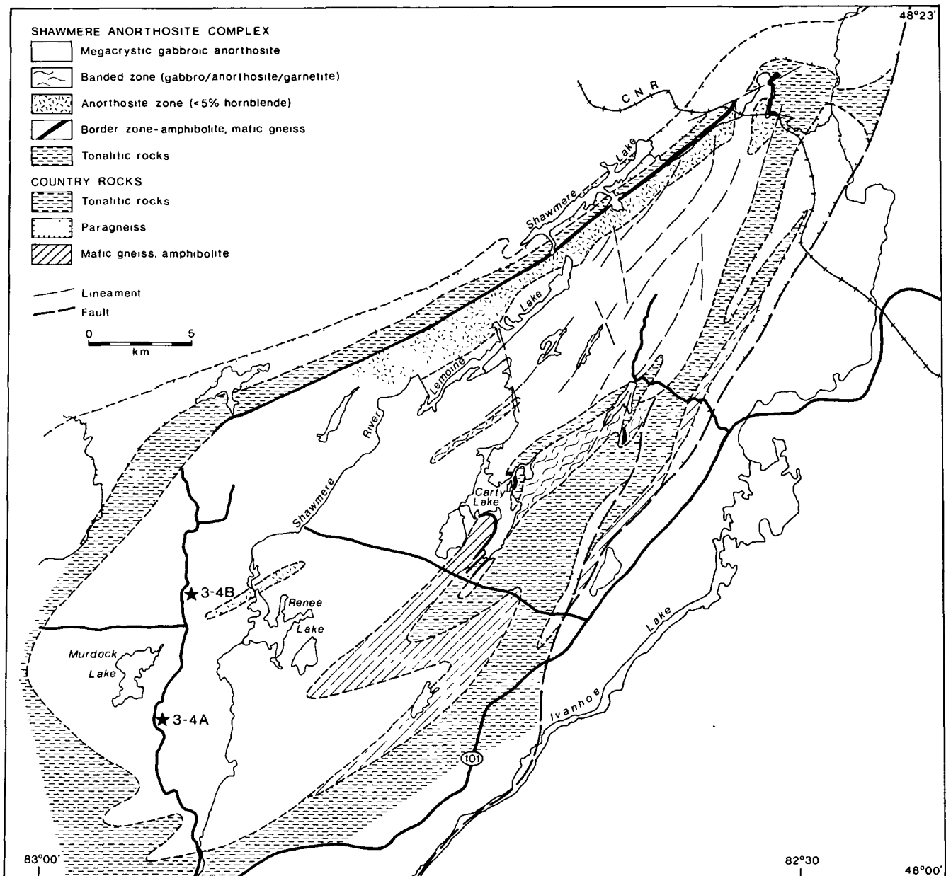
Fig. 6. Geology of the Shawmere anorthosite complex (after Riccio, 1980 and Percival, 1981).
