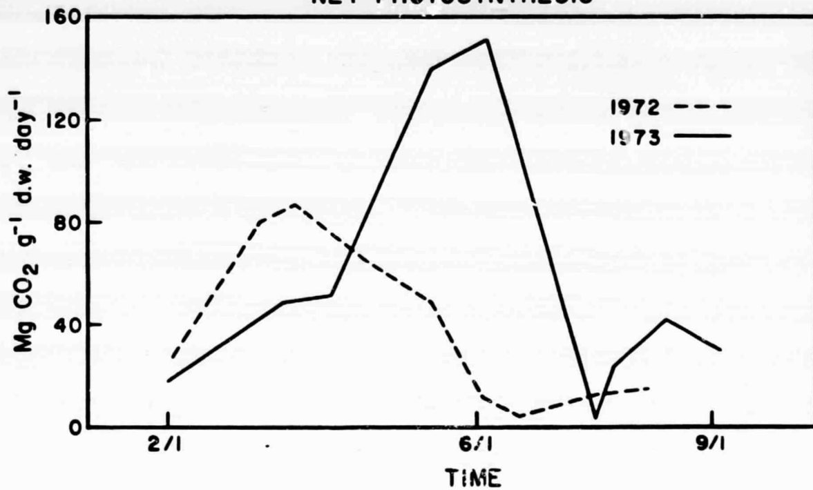
Figure 13. Net photosynthetic uptake of CO 2 by an evergreen shrub in the Mojave Desert for 1972 and 1973 (after Bamberg et al., 1976).
