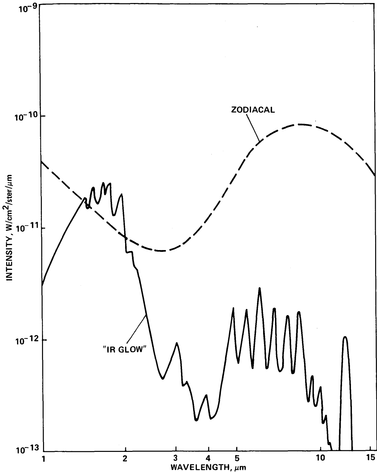
Figure 6.- The zodiacal light intensity, assuming observation 90° from sun on the ecliptic, is crudely plotted with the dashed line as a function of wavelength. (The intensity drops by a factor of ~3 for observations perpendicular to the ecliptic.) The expected IR glow intensity is schematically shown with the solid line marked "IR glow," calculated using the assumptions outlined in the text. The precise shape of the spectrum, sketched here assuming the OH spectrum from figure 5, is quite uncertain since OH may not be responsible for the Shuttle glow (see text).
