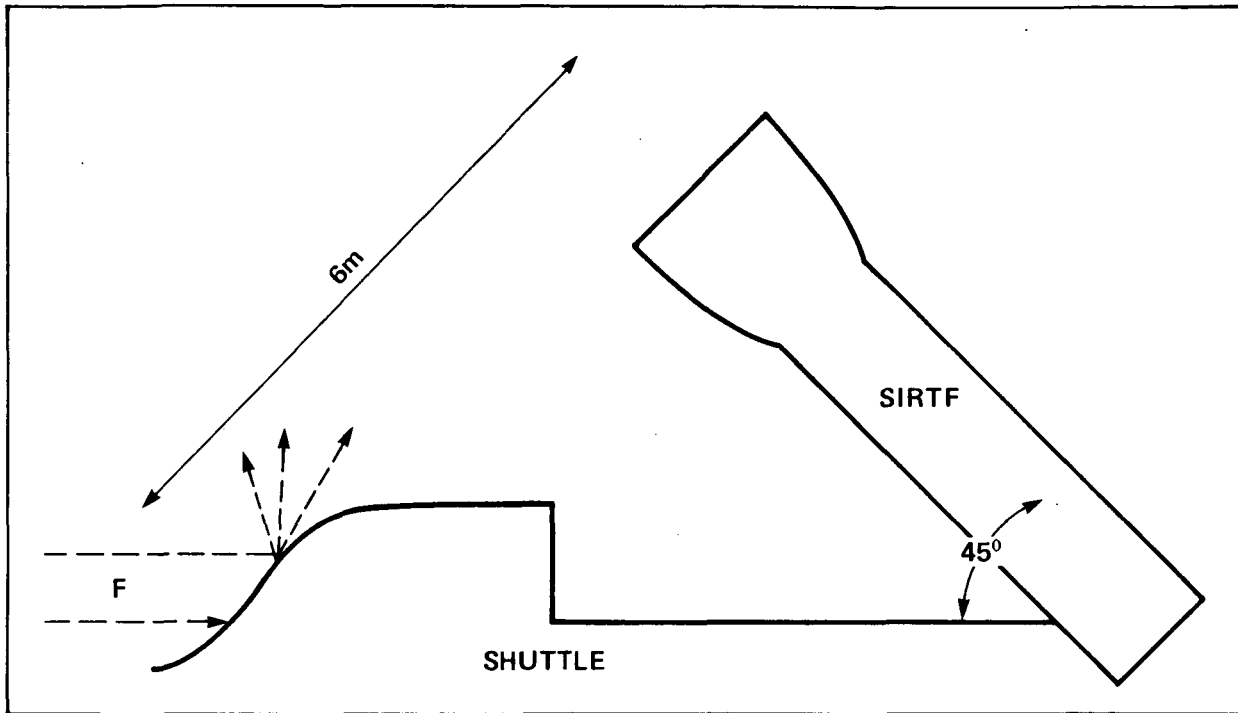
Figure 4.- The worst case configuration for SIRTIF observing the infrared glow associated with the observed optical glow is schematically shown. The atmospheric flux F impacts a minimum distance of about 6 m from the SIRTIF line-of-sight. This configuration can be modeled with figure 3b, using r_d \sim 6 m and r_o \sim 3 m.
