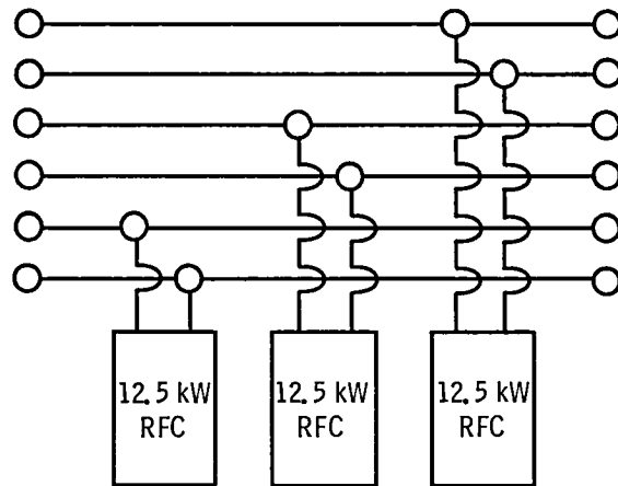
Figure 3. - 37.5 kW RFC energy storage system.
