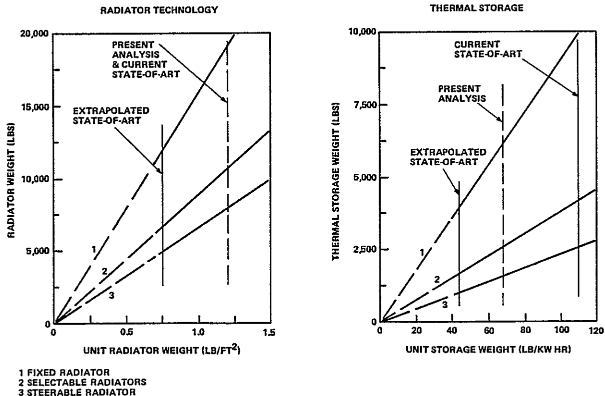
Figure 3.4-10. Benefits of Radiator and Thermal Storage Advances
