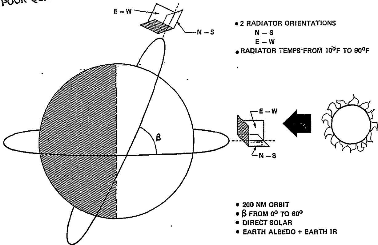
Figure 3.4-4. Radiator Analysis
