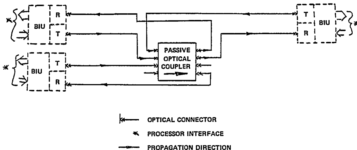
Figure 3.3-4. Passive Star Coupled Bus
