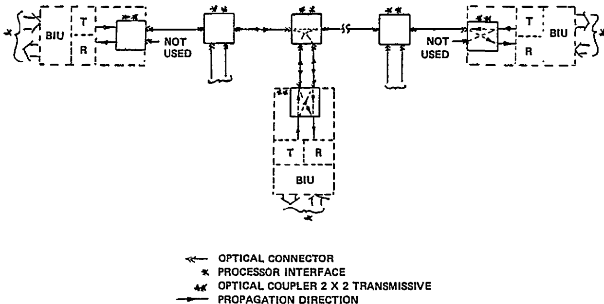
Figure 3.3-3. T-Coupled Optical Bus
