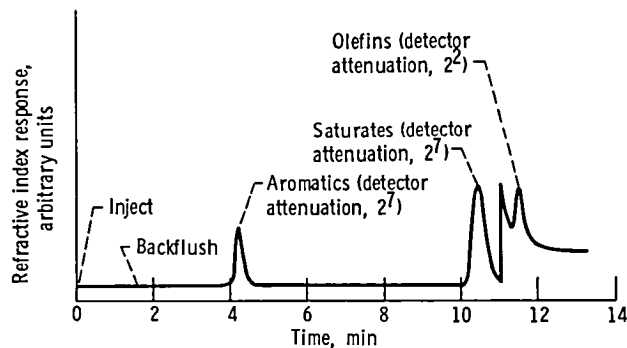
Figure 3. – Typical chromatogram for olefin determination (2 percent C_{12}H_{24} ).
