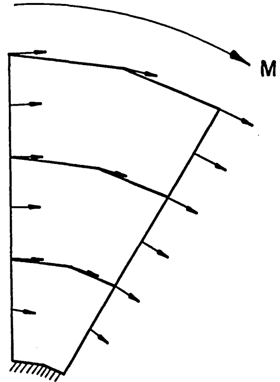
Fig. 12 - Qualitate Nodal Displacements from Numerical Solution of Hub Rotation Interior Problem. (Displacements not to scale.)
