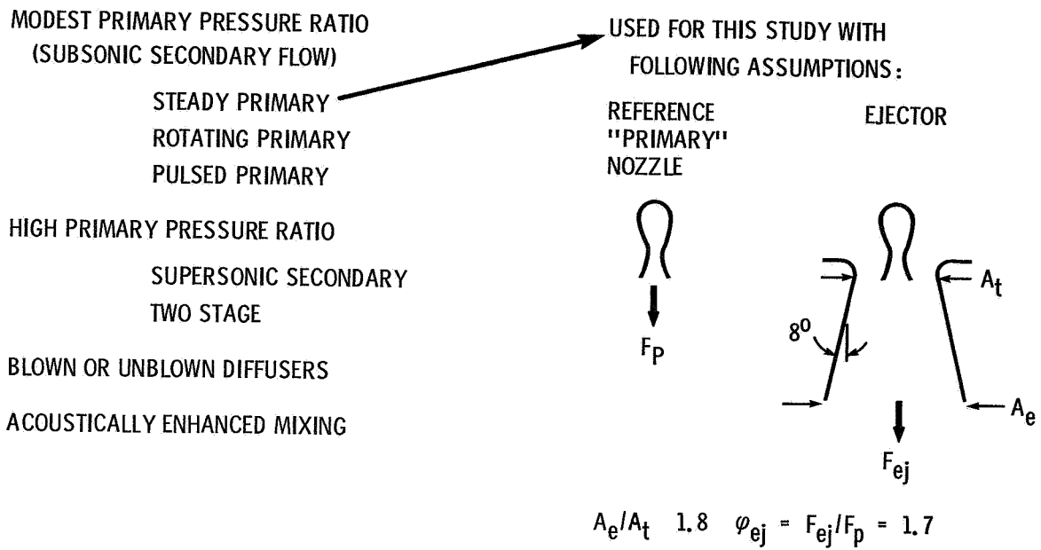
Figure 3. - Ejector types.
