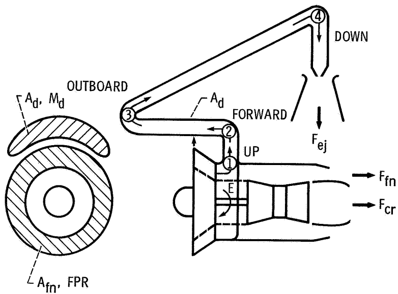
Figure 8. - Ejector propulsion system parameters.
