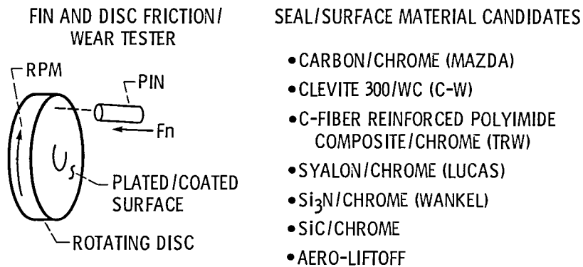
Figure 9. - Apex seal research.
