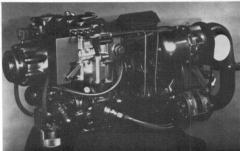
ROTARY ENGINE SFC = 0.35 lb/hp-hr SP. wt. = 0.80 lb/hp
