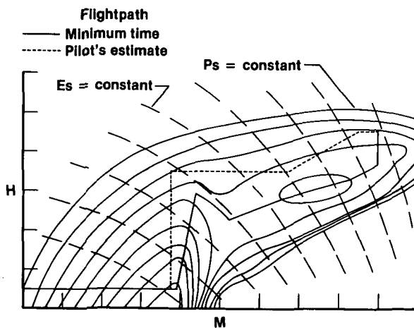
Fig. 12 Es and Ps contours and minimum time flightpaths for the F-15 HIDEDEC at maximum power without uptrim.
