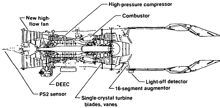
Fig. 3 Features of the F100 EMD engine for the HIDEC program.
