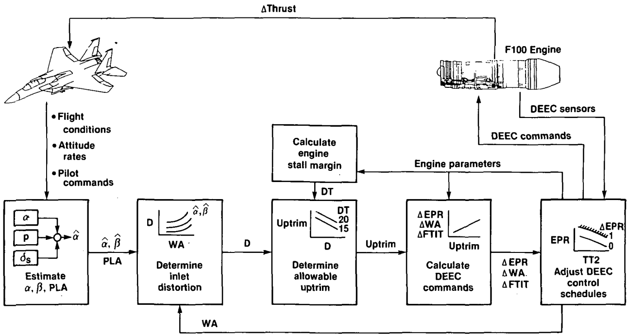
Fig. 4 Block diagram of the HIDEC adaptive stall margin mode.
