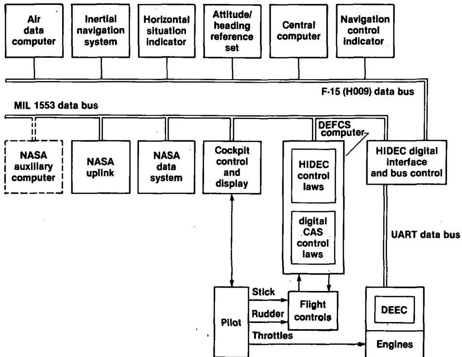
Fig. 2 Block diagram of the HIDEC system.
