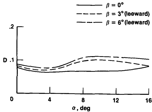
Fig. 5 Effect of \alpha and \beta on D for the F-15; M = 1.6 .
