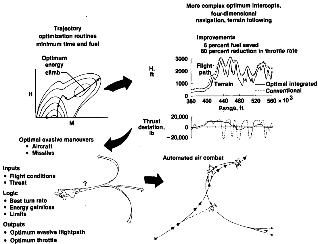
Fig. 11 Integrated flightpath management modes for the HIDEDEC program.
