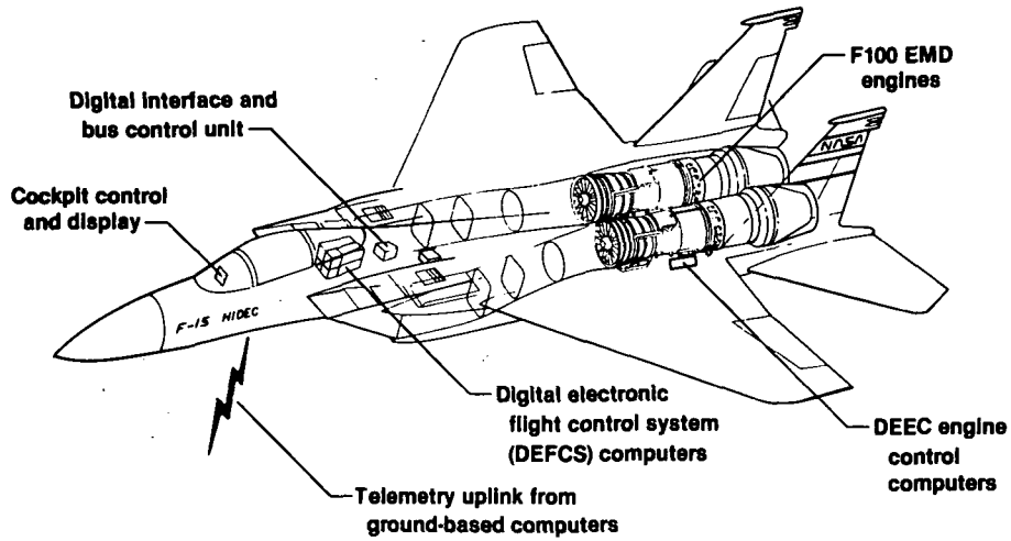
Fig. 1 Features of the F-15 HIDEC research airplane.
