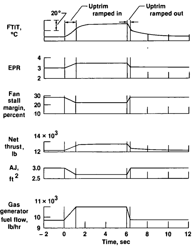
Fig. 9 Evaluation of HIDECA ASM uptrim using the F100 EMD linear state-variable dynamic simulation at intermediate power and at low-altitude, low-speed conditions.
