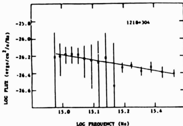
Figure 1. IUE Spectrum of 1218+304
