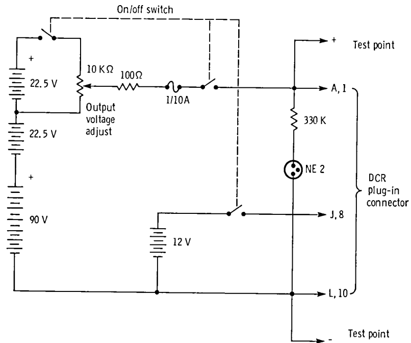
Figure 13. - High voltage duty cycle regulator calibrator.
