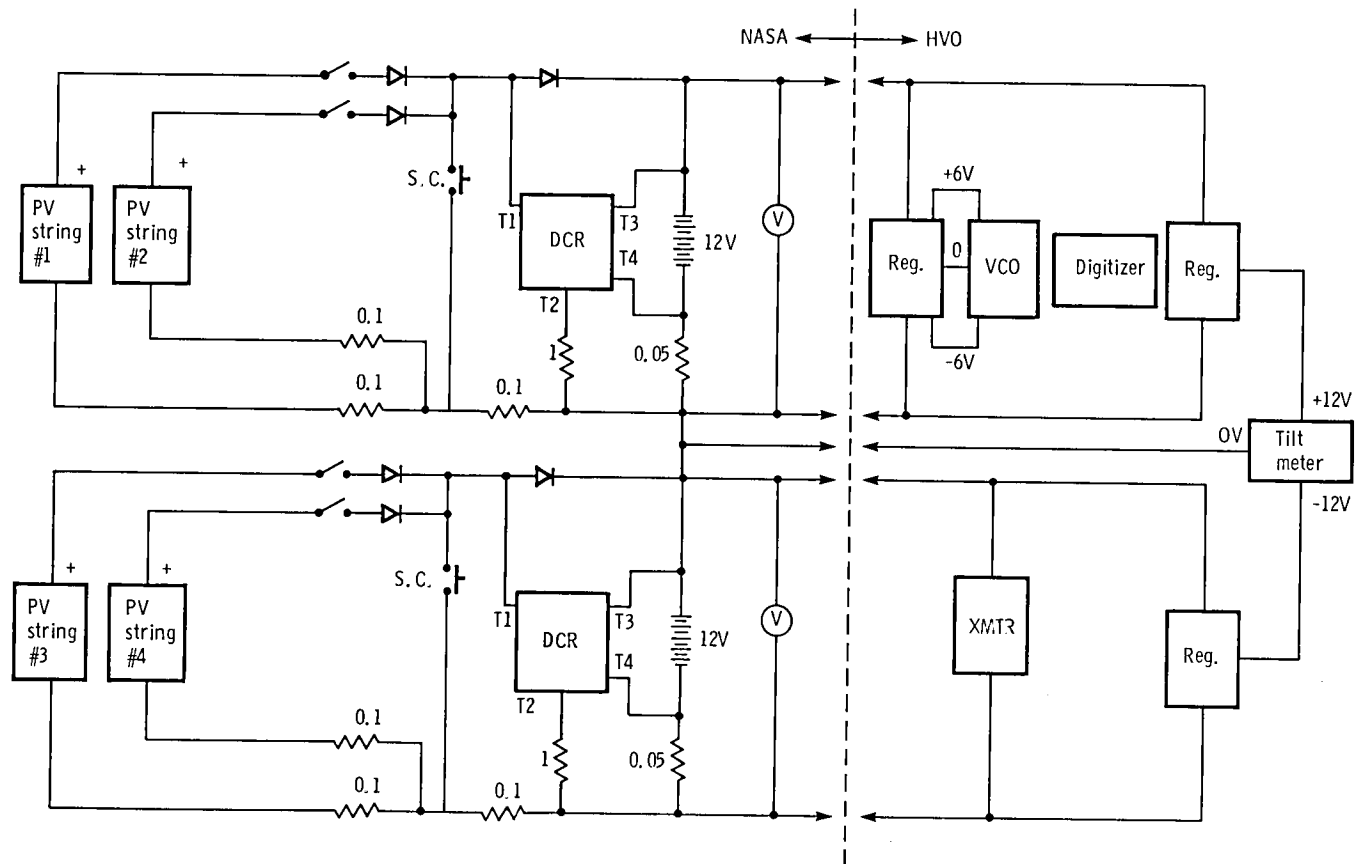
Figure 18. - Hawaii volcano observatory system schematic diagram (simplified).
