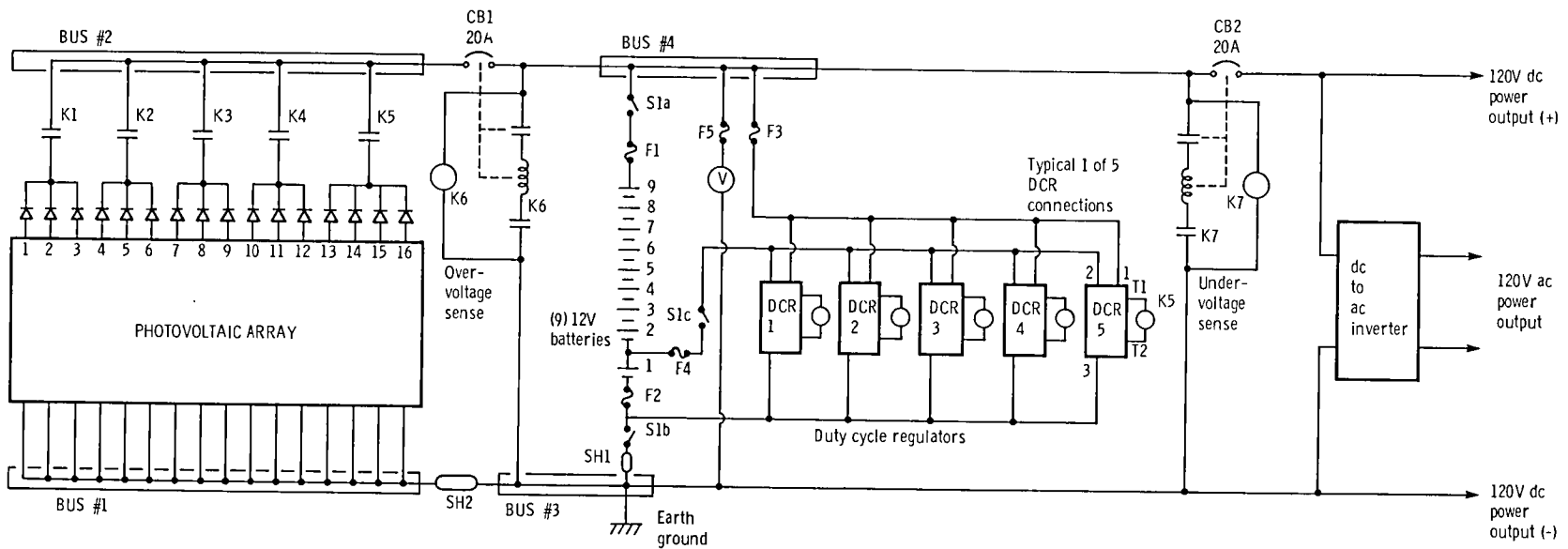
Figure 17. - Unispace 82 system schematic diagram.
