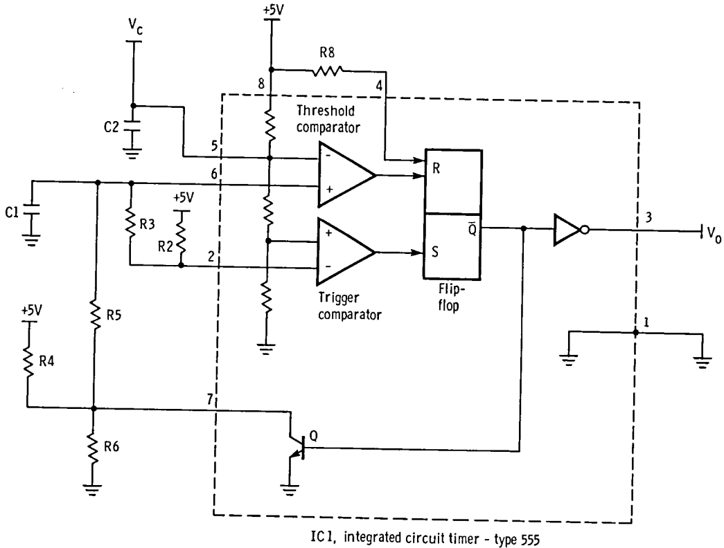
Figure 7. - High voltage duty cycle regulator circuit diagram (details).
