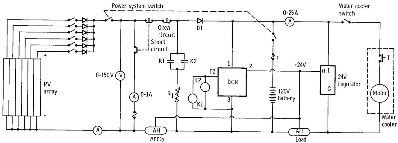
Figure 16. - Lone pine system schematic diagram (simplified).
