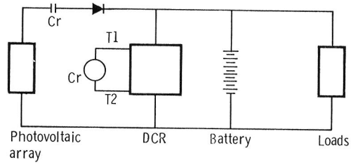
(a) Series control.
