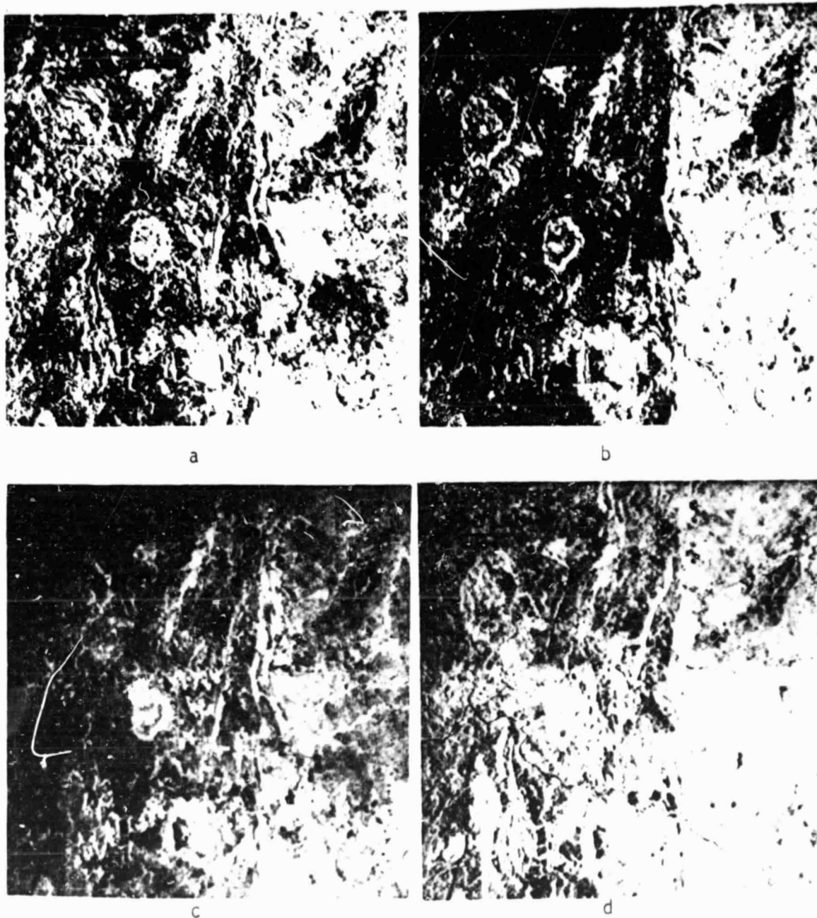
Fig. 7 - Example of Band Ratioing (a and b) and Principal Components (c and d) of the same images as in Figure 5: a) R_{7/5} of the dry season (June, 77) b) R_{7/5} of the rainy season (February, 77) c) Second Component of the dry season (June, 77) d) Second Component of the rainy season (February, 77). All these images have been contrast stretched after ratioing, and Principal Component Transformation.
