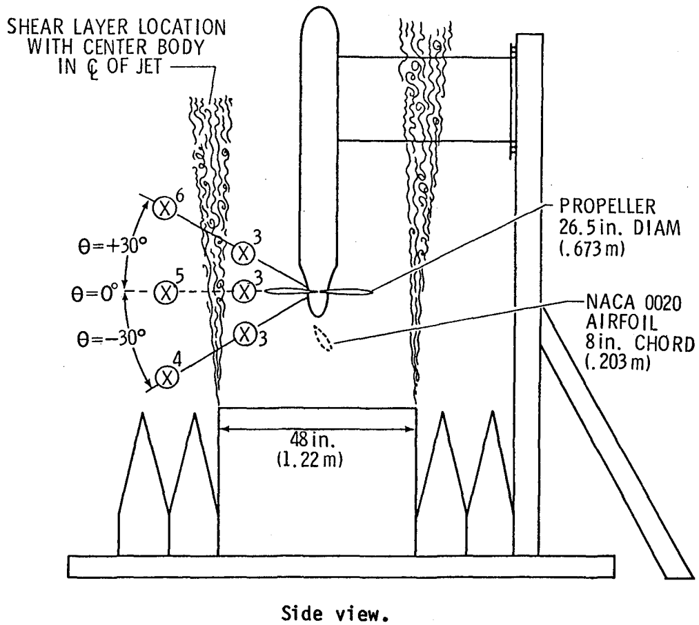
Figure 6.- Schematic of the test setup.
