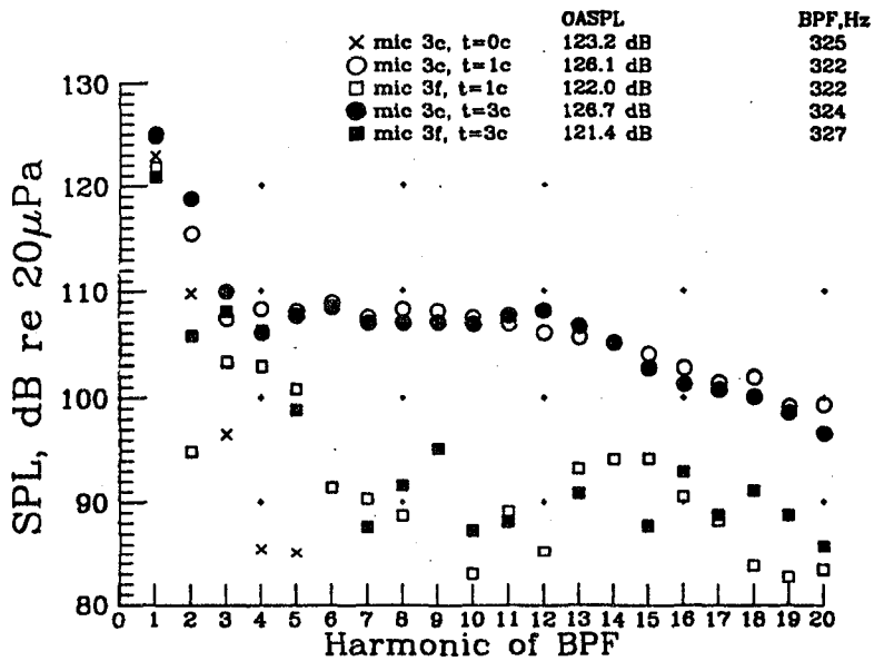
(e) 30° downstream ( \theta = 30^\circ ), microphone 3.
