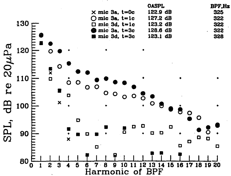
(a) 30° upstream ( \theta = -30^\circ ), microphone 3.
