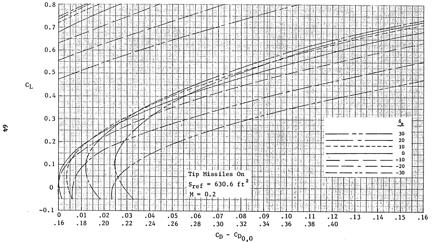
Figure 4-8 Variation of Low-Speed Drag Due to Lift and Camber with Lift Coefficient and Elevon Deflection in Free Air
