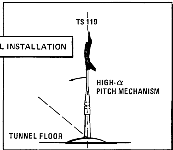
Figure 8-3 Installation Sketches for the Unitary and 12-Foot Wind Tunnels
