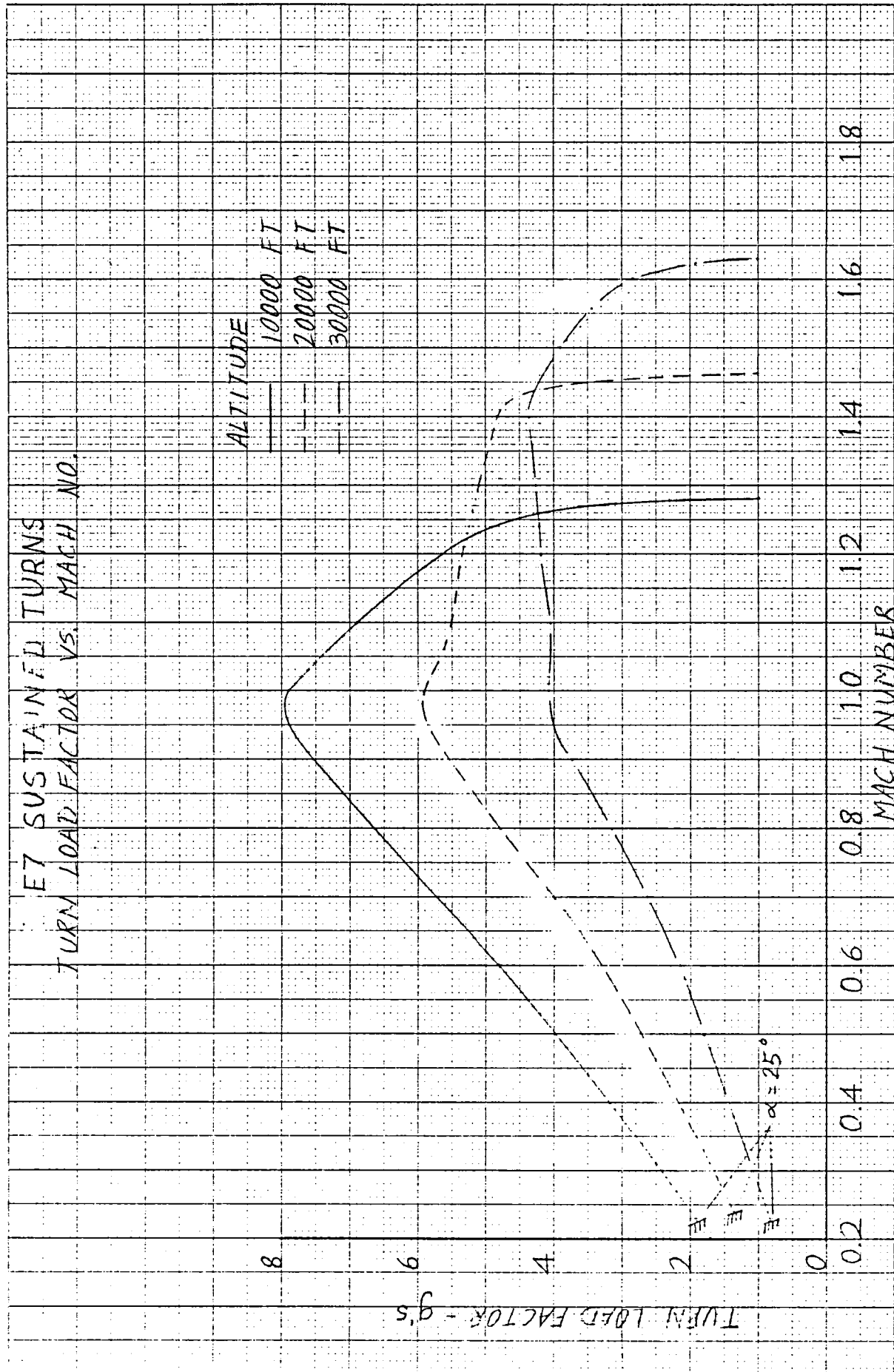
Figure 6-3 Sustained Turn Load Factor versus Mach Number
