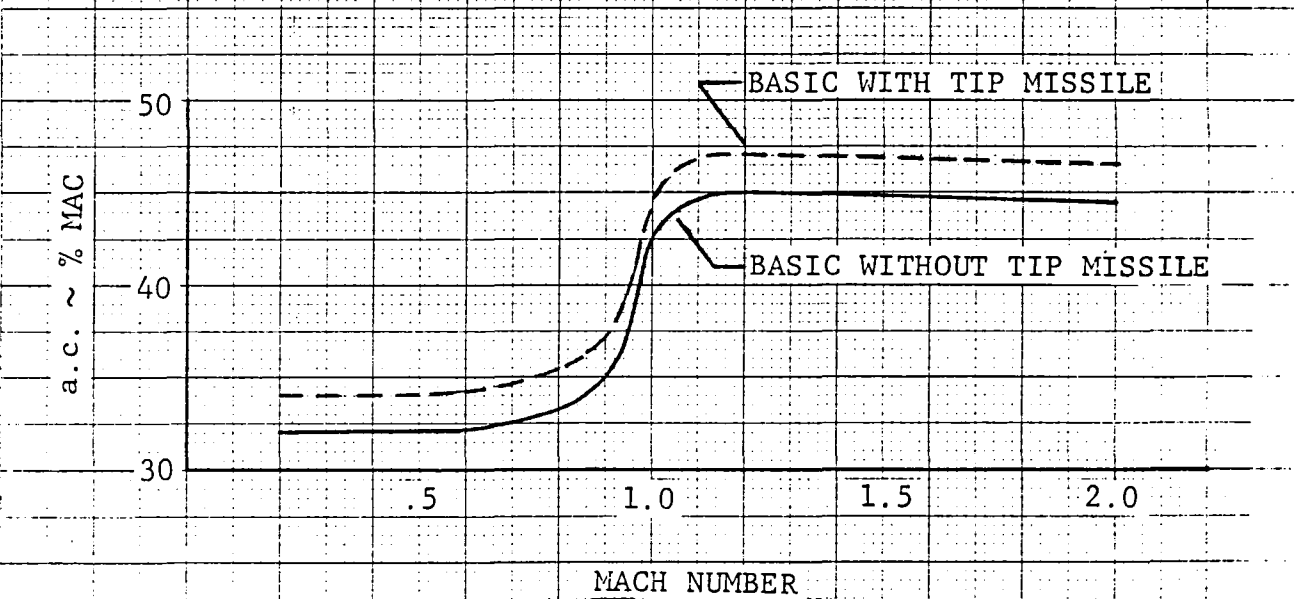
Figure 4-12 Aerodynamic Center Location Versus Mach Number
