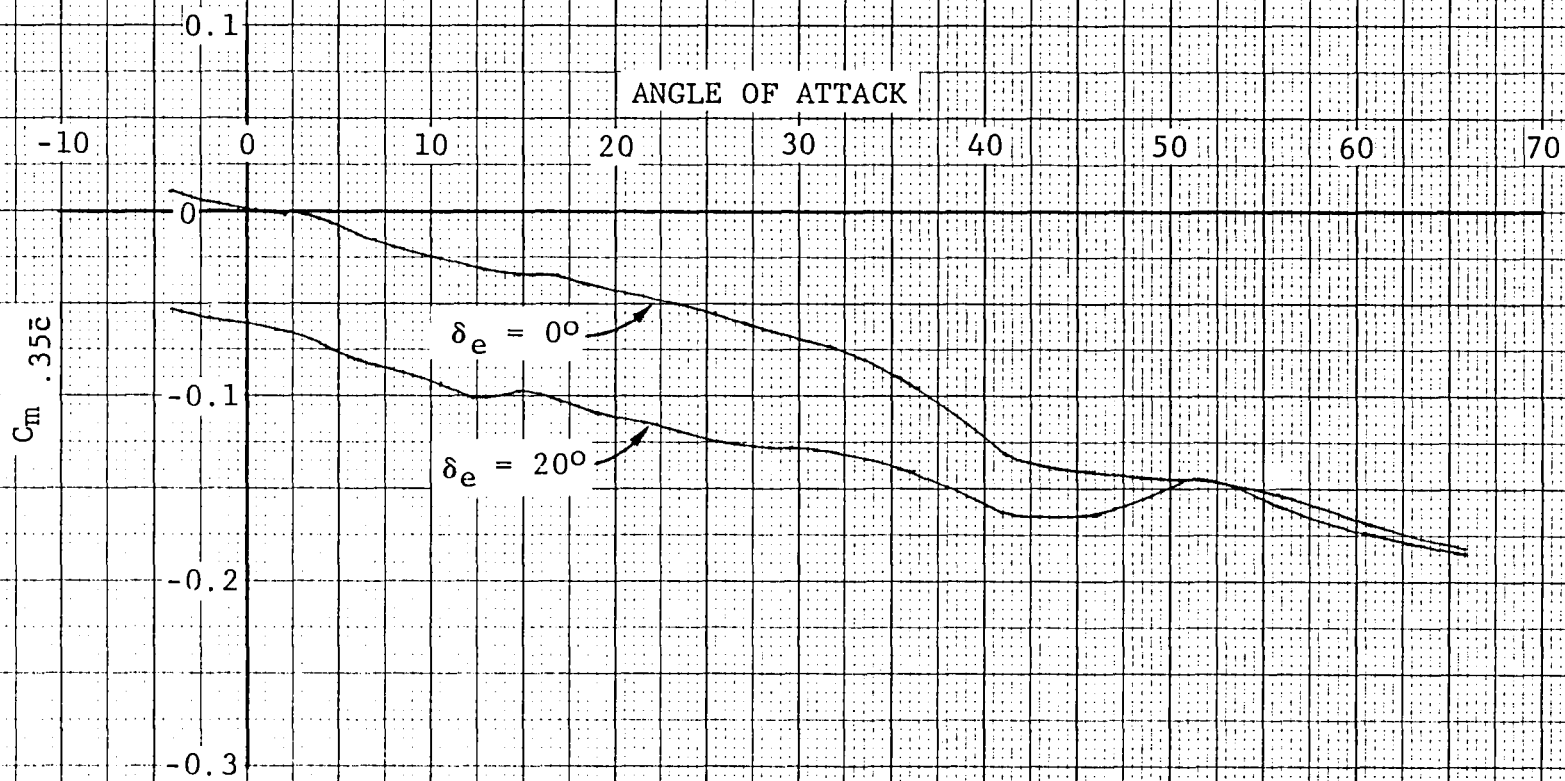
Figure 4-30 Pitching Moment Versus Angle of Attack to Very High \alpha 's
