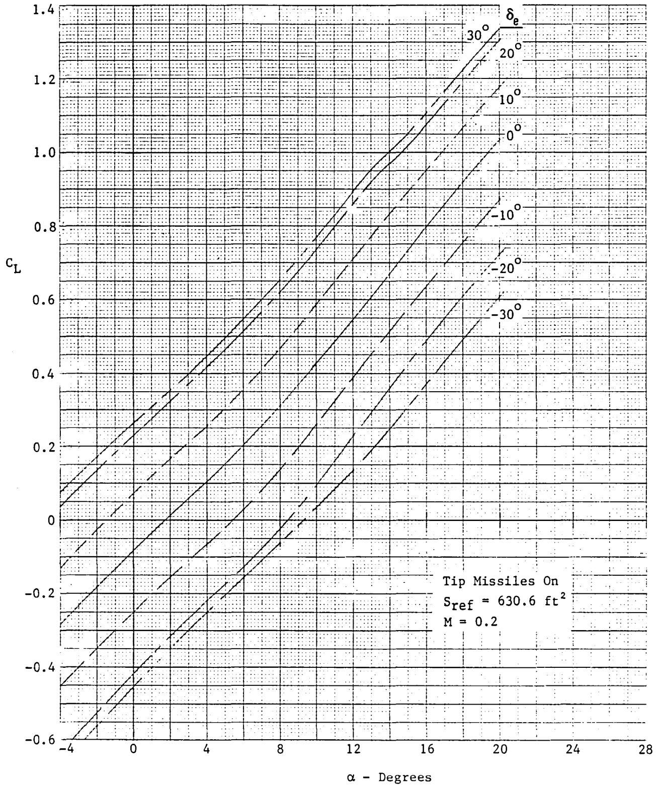
Figure 4-9 Variation of Low-Speed Lift Coefficient with Angle of Attack and Elevon Deflection in Ground Effect
