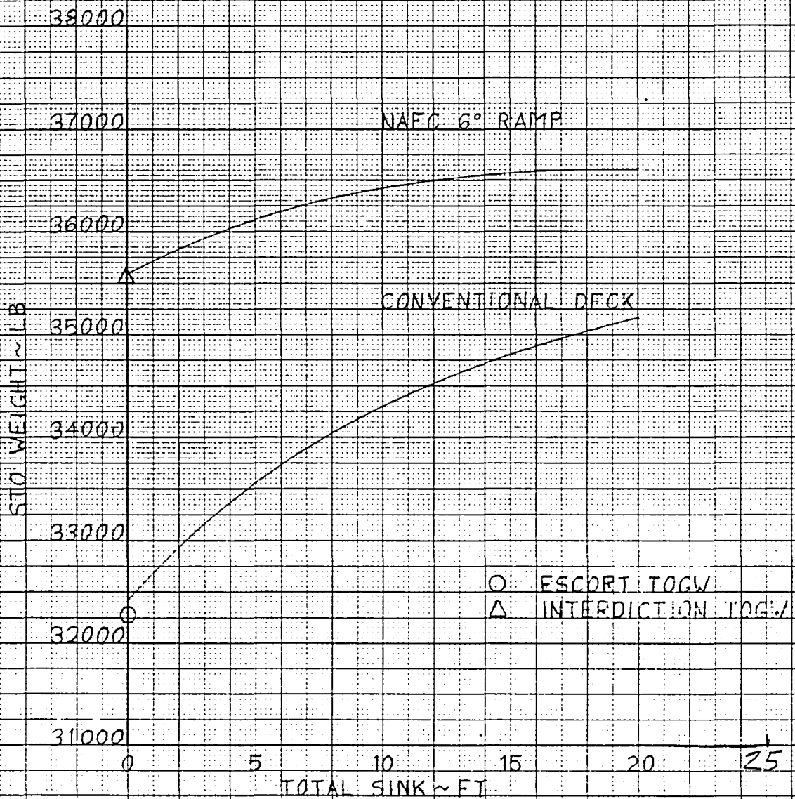
Figure 6-5 STO Weight versus Sink Over Bow
