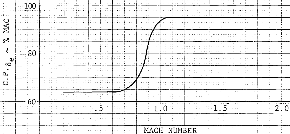
Figure 4-16 Center of Pressure of Lift due to Elevator Deflection Versus Mach Number
