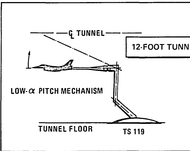
Figure 8-3 Installation Sketches for the Unitary and 12-Foot Wind Tunnels
