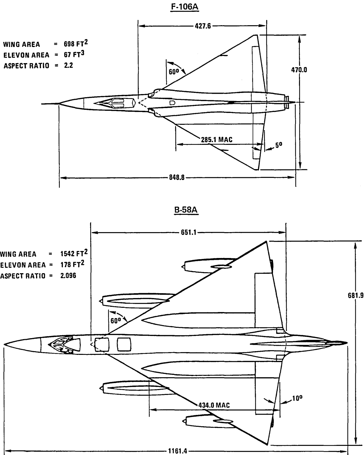
Figure 4-2 F-106A and B-58A Planform Comparison
