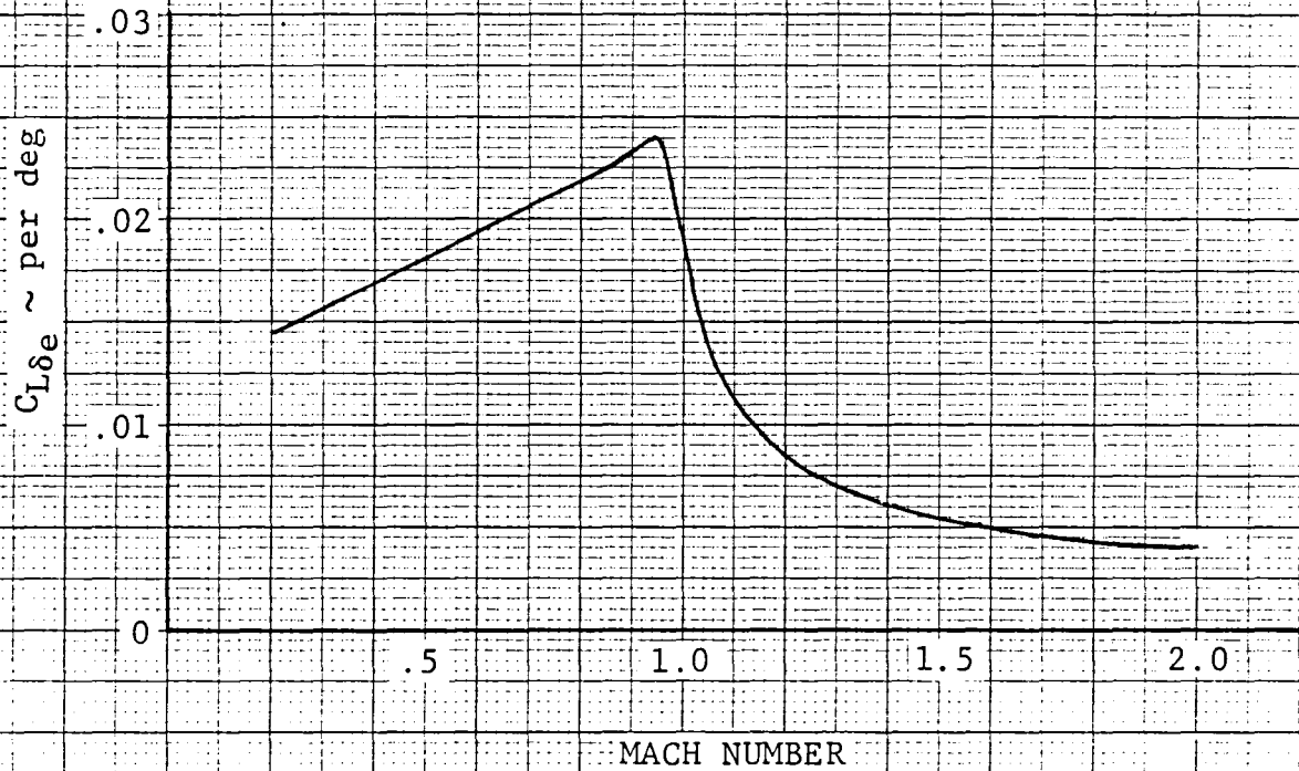
Figure 4-15 Change in Lift with Elevator Deflection Versus Mach Number
