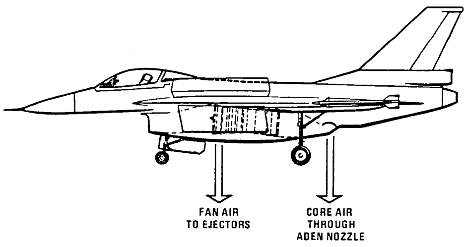
Figure 1-2 Propulsion System — Hover Configuration
