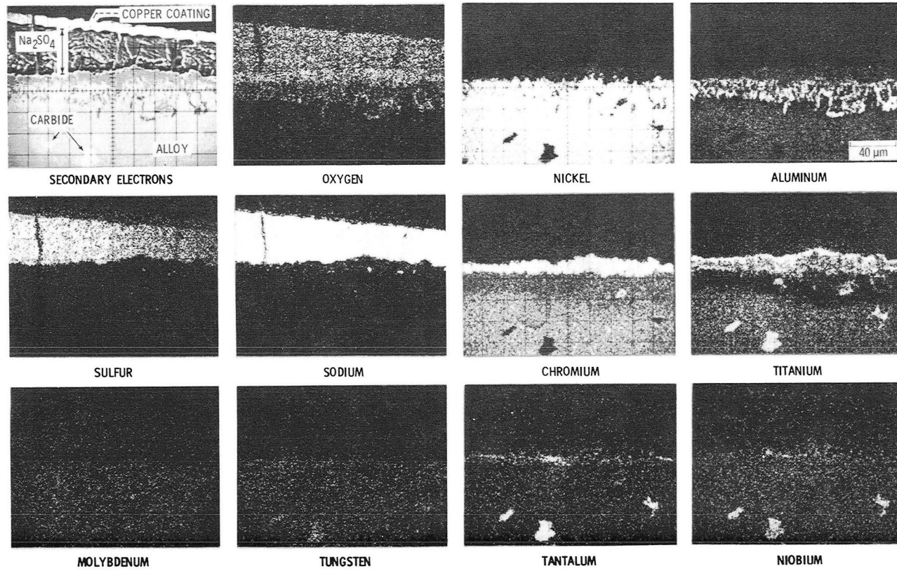
Figure 7.—Secondary electron and X-ray micrographs of preoxidized IN-738 specimen corroded for 5 min at 975° C with 3 mg cm -2 Na 2 SO 4 .
