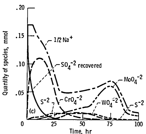
(a) Typical specific weight change. (b) Concentration of SO 2 evolved. (c) Quantity of water-soluble species remaining.
