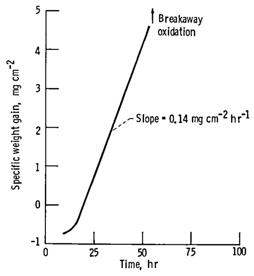
Figure 4.—Replot of weight change data of preoxidized IN-738 presented in figure 3(a) with the scale for the specific weight expanded to the same sensitivity as that of figure 1.
