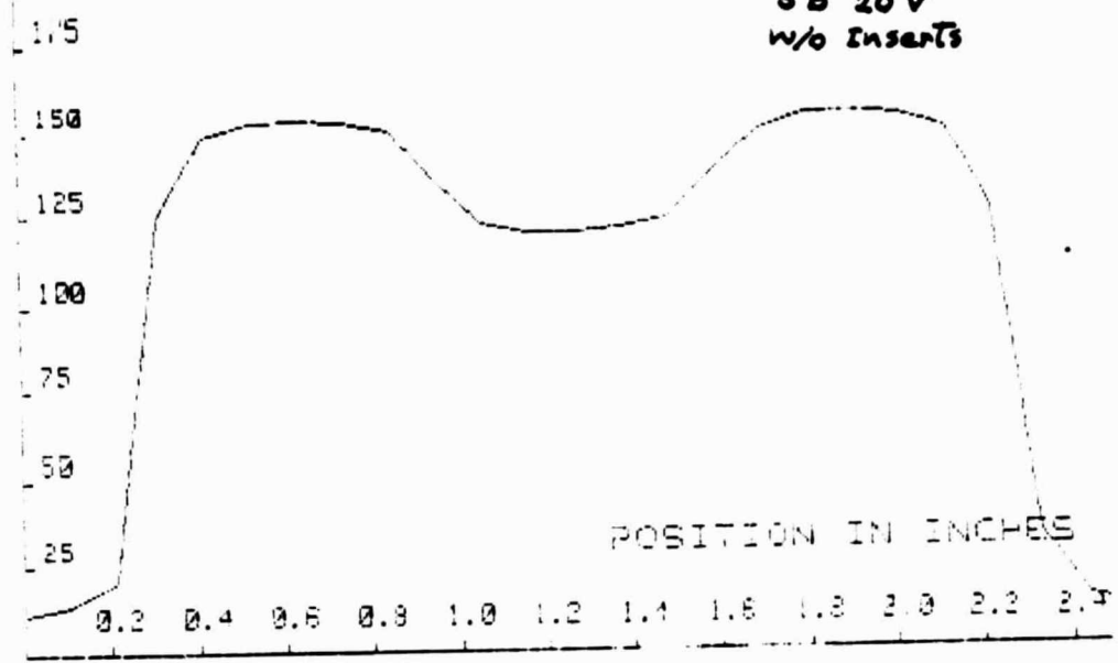
Fig. 2 - Typical Exit Velocity Profiles Obtainable with Modified Injector
