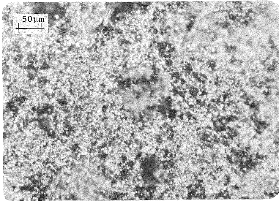
Fig. 4 Optical micrograph of S079A3 print (with eutectic dopant), fired at 500°C (two step) at 200X.
