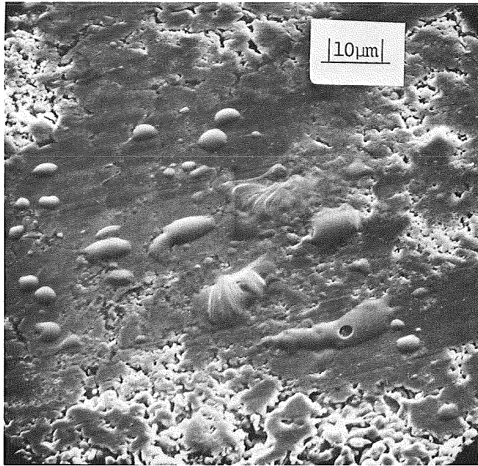
Figure 55. F30-584 o C CO with diamond scribed scratch at 1,000X magnification
