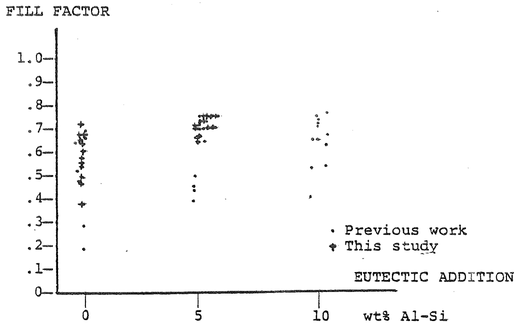
Figure 20 Fill factor versus amount of Al-Si eutectic addition to screened back electrode copper paste
