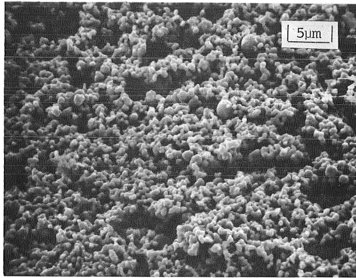
Figure 46. F 20 copper electrode sintered at 615°C taken at 2000X
