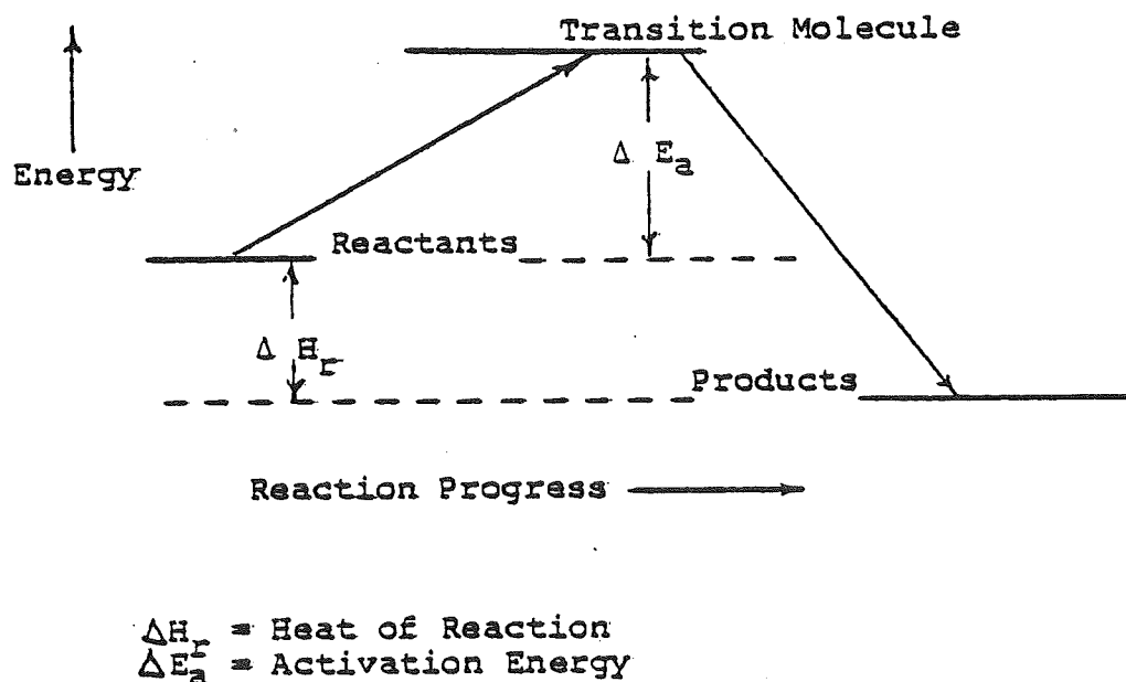
Figure 40 The Relation Between Heat of Reaction and Reaction Activation Energy
