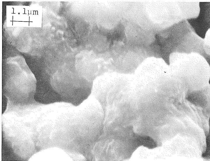
Figure 13 SEM micrograph of F12 electrode fired in nitrogen at 550°C, at 9000x.
