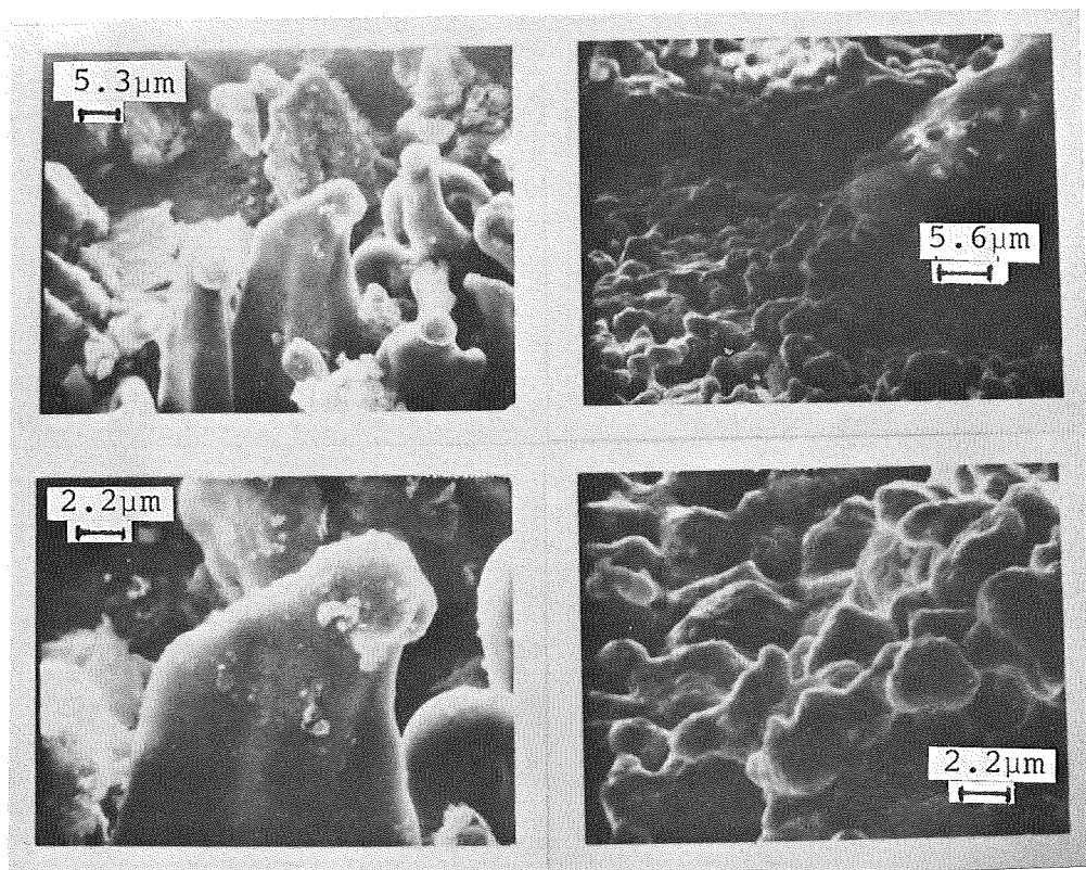
Figure 26 Composite of SEM micrographs of S080 successful screen print.
