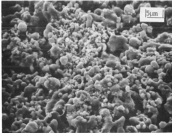
A. F27-650 o C, H 2 , Magnification 2,000X
