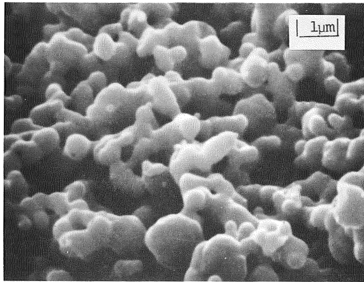
Figure 47. Same as above at 10,000X
