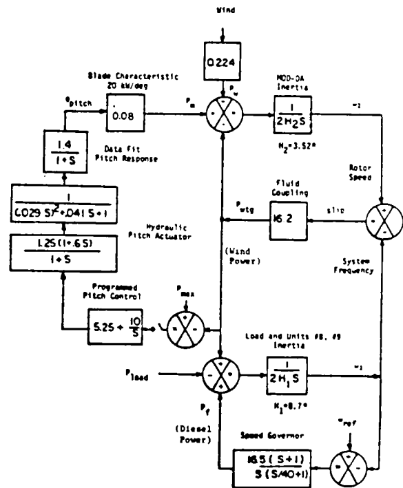
Figure 8 - MOD-OA and BIPCO Dynamic Model
