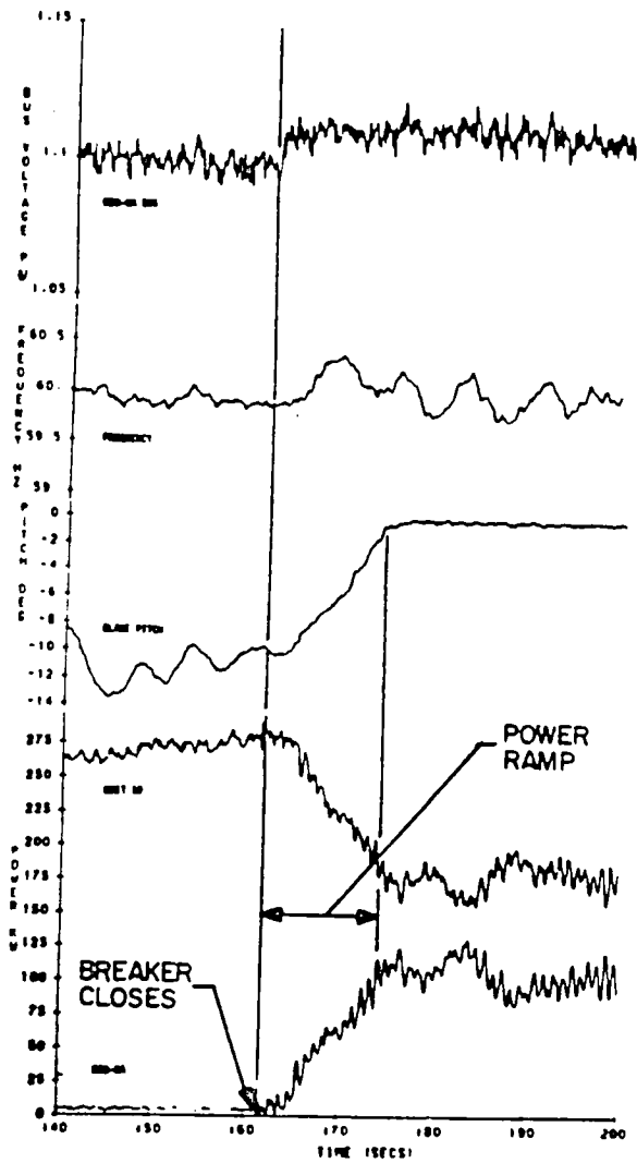
Figure 4 - Startup and Synchronization of the MOD-0A WTG
