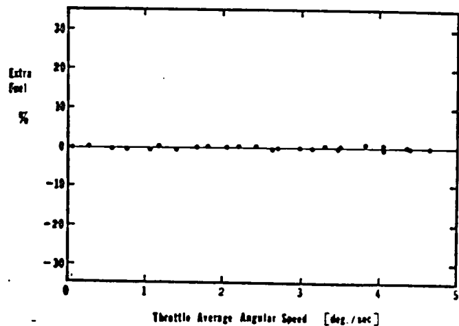
Figure 6 - Throttle Motion vs. Extra Fuel
