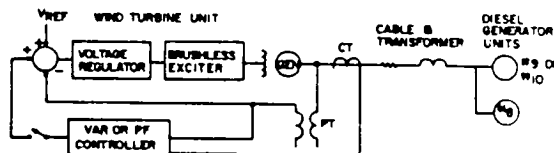
Figure 1 - Basic Configuration for Study of Excitation Control on MOD-0A WTG.
