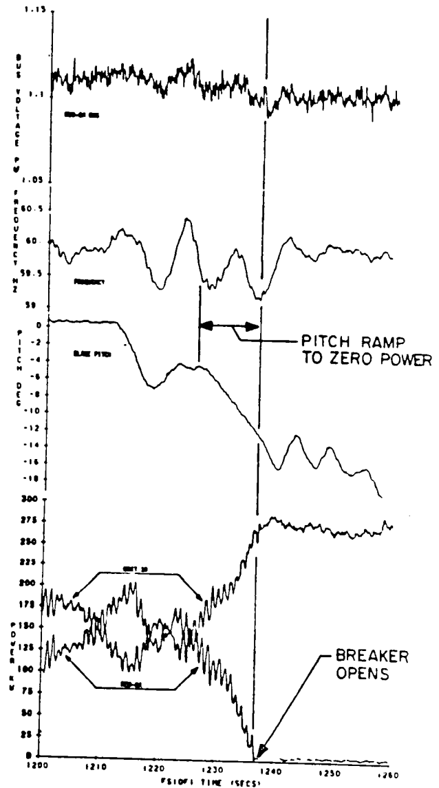
Figure 5 - Normal Shutdown and Cutout of the MOD-0A WTG
