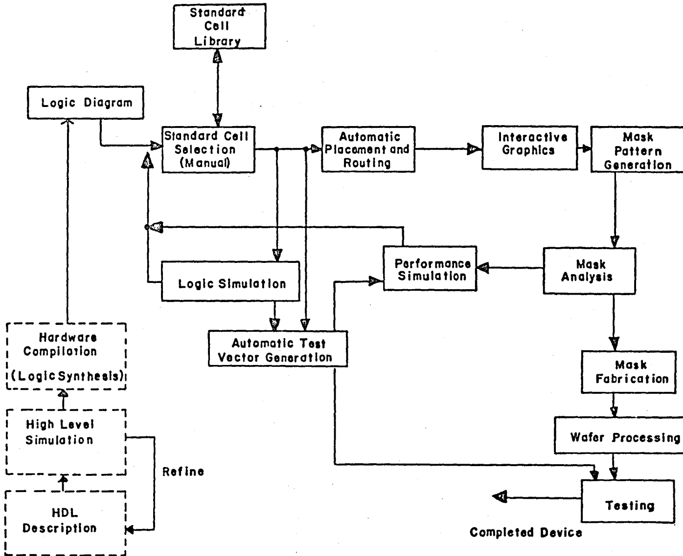
Figure 6 : CADAT System
