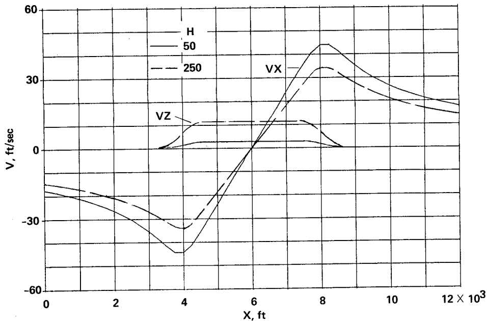
(a) Winds along paths through center of downburst.
