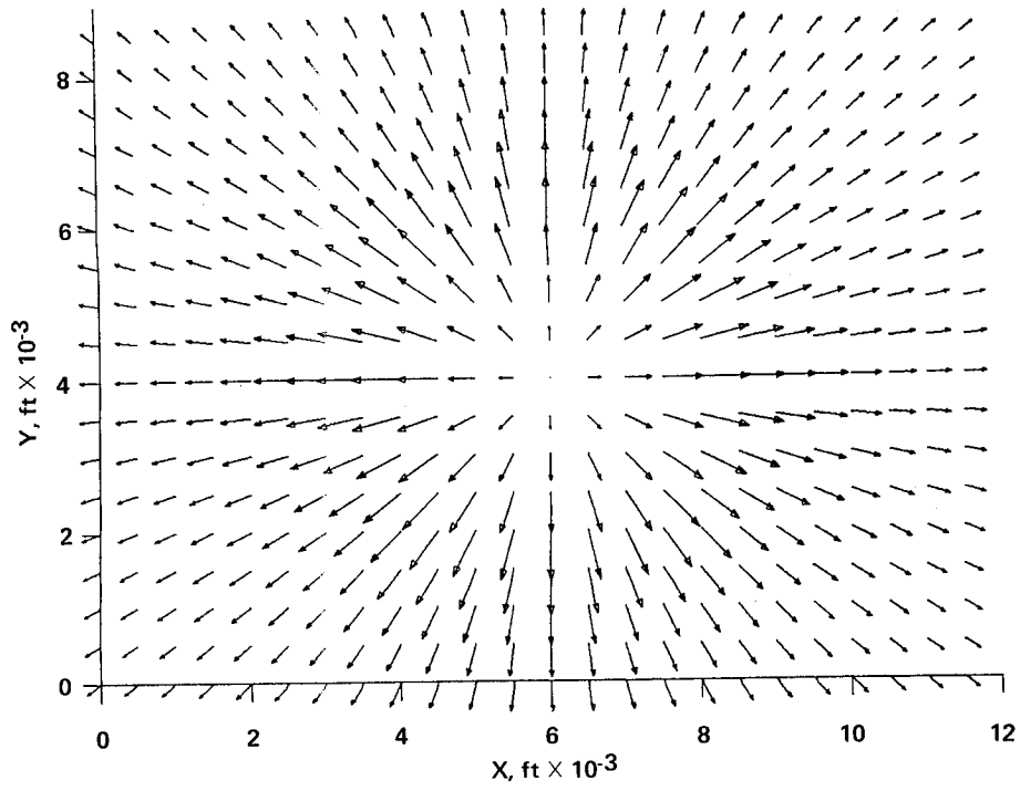
(b) Horizontal flow field at H = 50 ft.
