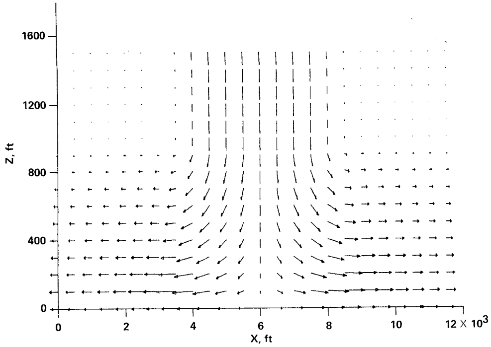
(c) Vertical cross section through center of down burst.
