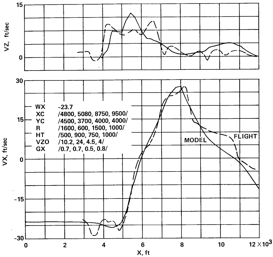
Figure 7.- Model of shear recorded in landing approach near-accident, 1975.
