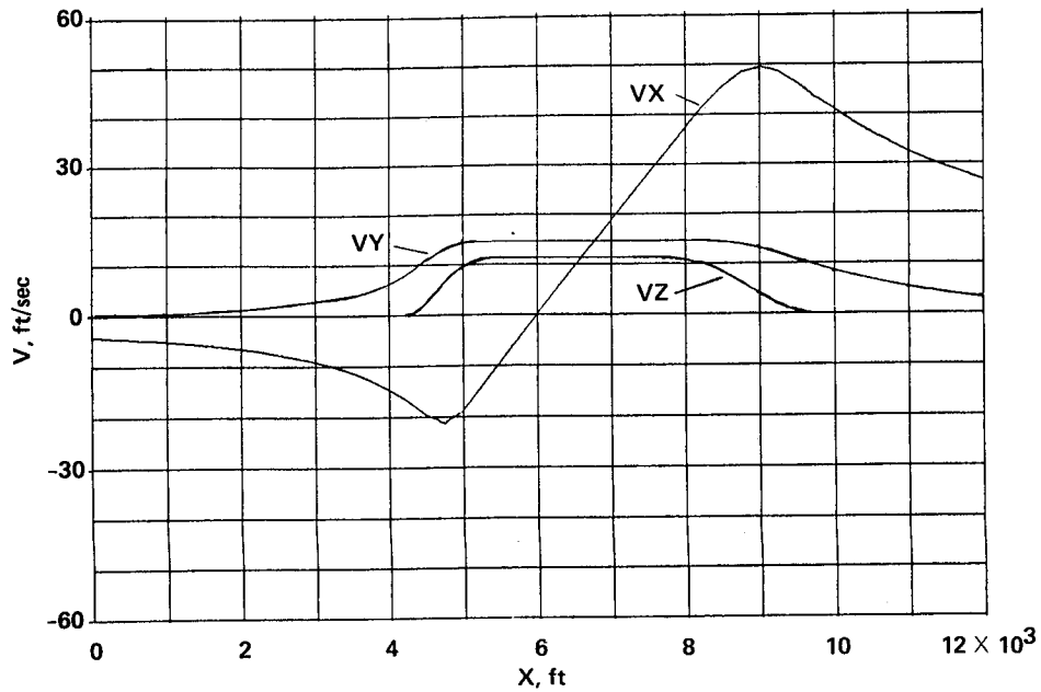
(a) Winds at 250 ft, G_X = G_Y = 0.4 .
