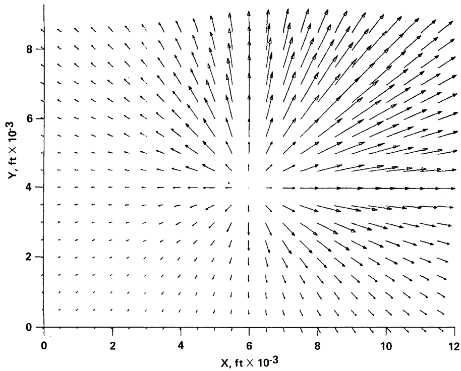
(b) Horizontal flow field, H = 50 ft.
