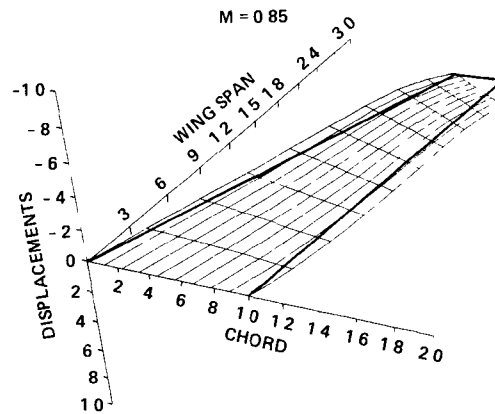
Fig 58 Shape of the swept wing at flutter is composed of the first bending and the first and second torsion modes
