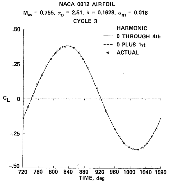
Fig. 29. Lift-coefficient variation during third cycle: NACA 0012, M_\infty = 0.755, k = 0.1628 .
