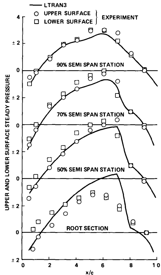
Fig 35 Comparison of steady pressure coefficients LTRAN3 and experiment
