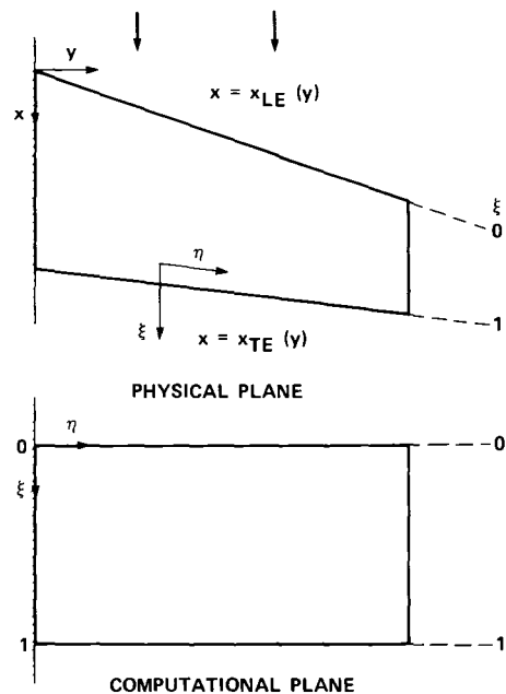
Fig 42. Sheared coordinate system \xi, \eta, \zeta used for swept and tapered wings
