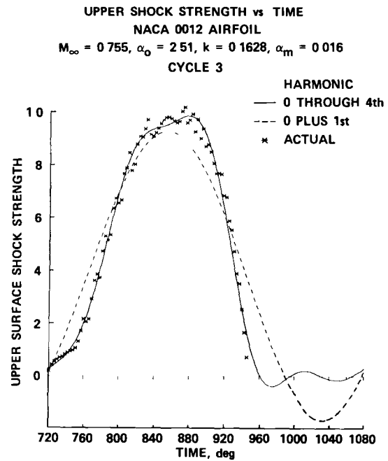
Fig 33 Upper-surface shock-strength variation NACA 0012, M_\infty = 0.755, k = 0.1628
