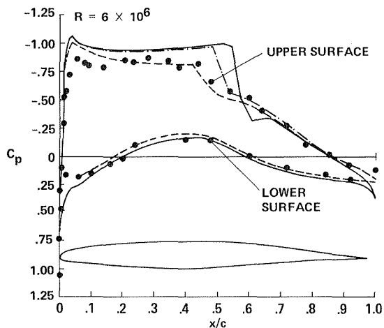
Fig. 12. Comparison of upper and lower surface steady-pressure distributions, theories and experiment.
