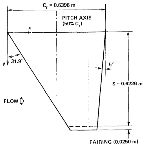
Fig. 43. Dimensions of the F-5 wing.
