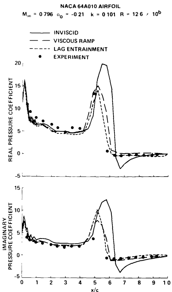
Fig 8 Real and imaginary parts of first Fourier component of unsteady lower-surface pressure coefficients k = 0.101
