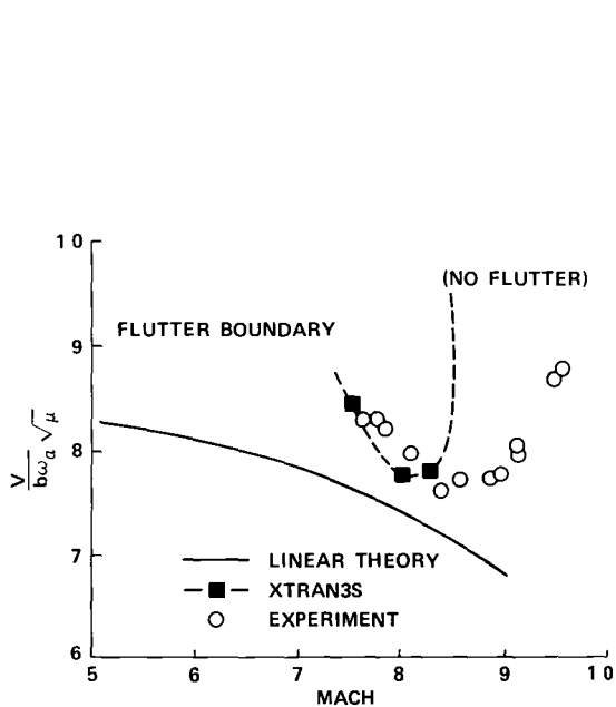
Fig 41 XTRAN3S flutter boundary for the Japanese transport wing
