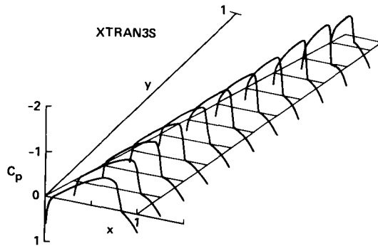
Fig 39. Steady-state initial conditions for Japanese transport wing M_\infty = 0.85
