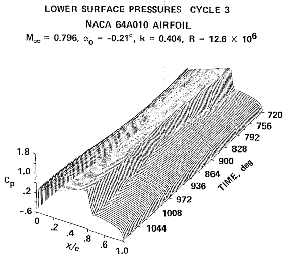
Fig. 11. Time-history of lower-surface pressure coefficients for third cycle of motion: NACA 64A010 airfoil, k = 0.404 .
