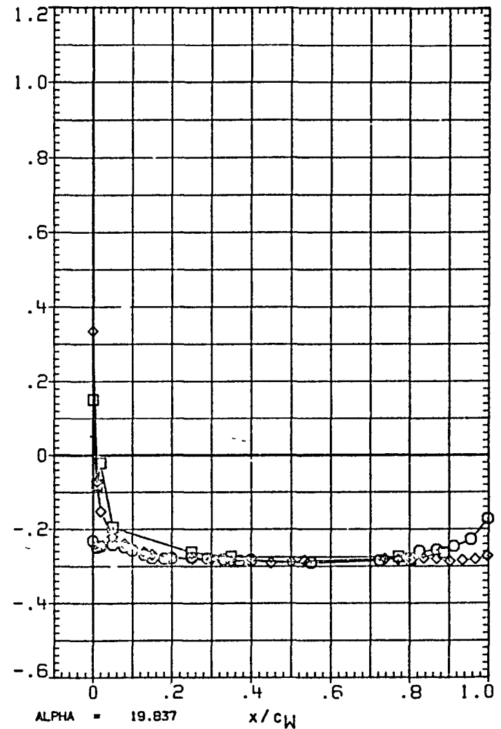
FIGURE 3G TYPICAL OA310C PRESSURE DISTRIBUTION - UPPER WING(LEFT)
