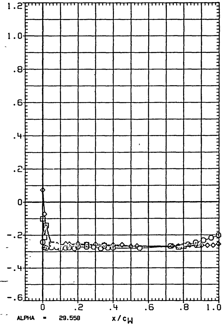
FIGURE 36 TYPICAL OA310C PRESSURE DISTRIBUTION - UPPER WING (LEFT)
