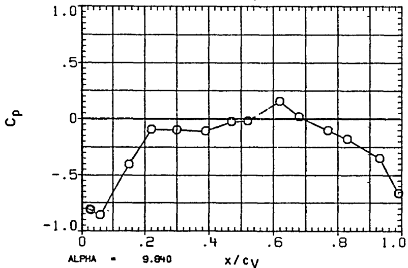
FIGURE 10 - TYPICAL OA310A PRESSURE DISTRIBUTION - VERTICAL TAIL (LEFT FACE)
