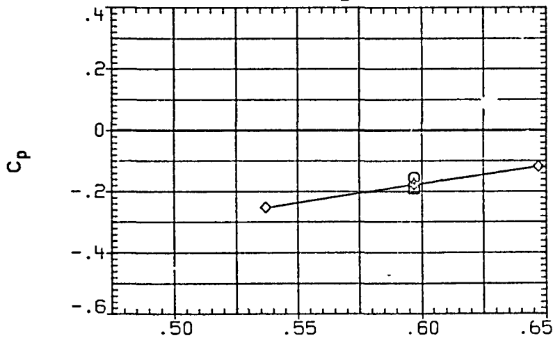
FIGURE 2C. TYPICAL OA310B PRESSURE DISTRIBUTION - MID-SIDE FUSELAGE
