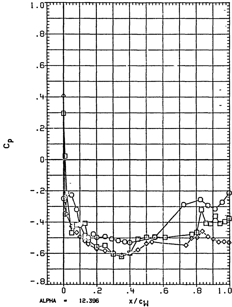
FIGURE 2G TYPICAL OA310B PRESSURE DISTRIBUTION - UPPER WING (LEFT)
