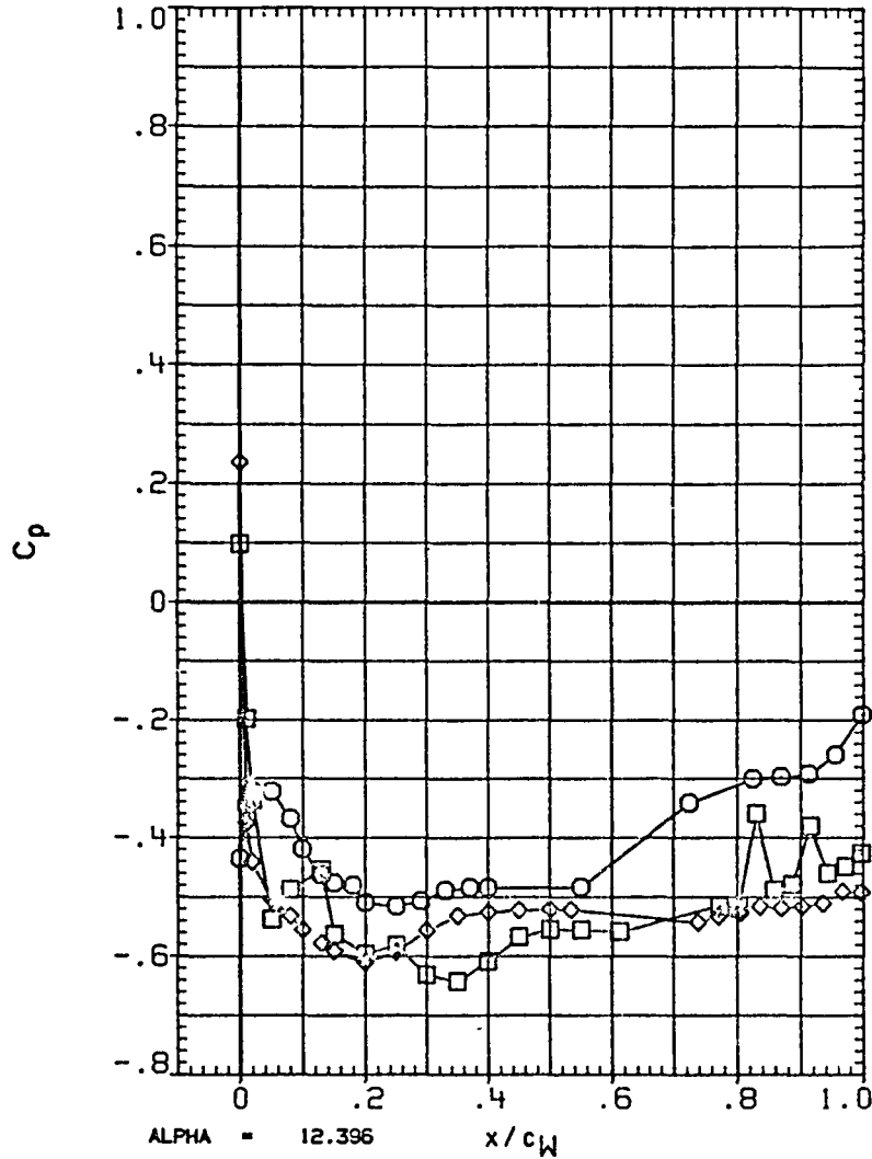
FIGURE 26 TYPICAL OA310B PRESSURE DISTRIBUTION - UPPER WING(LEFT)
