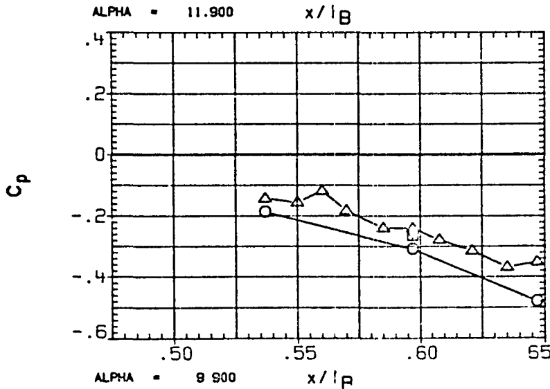
FIGURE 1C TYPICAL OA310A PRESSURE DISTRIBUTION - MID-SIDE FUSELAGE
