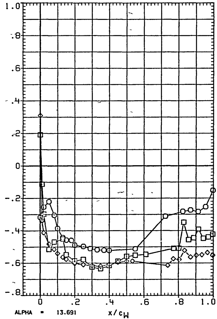
FIGURE 2G TYPICAL OA310B PRESSURE DISTRIBUTION - UPPER WING (LEFT)
