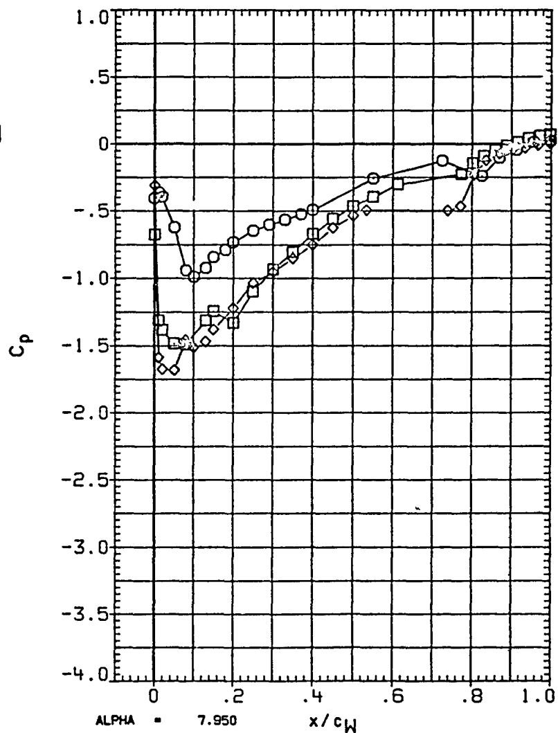
FIGURE 1G TYPICAL OA310A PRESSURE DISTRIBUTION - UPPER WING (LEFT)
