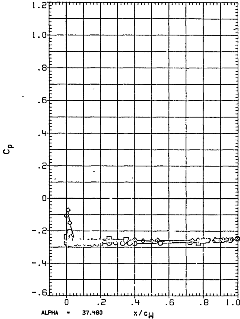
FIGURE 3G TYPICAL OA310C PRESSURE DISTRIBUTION - UPPER WING(LEFT)
