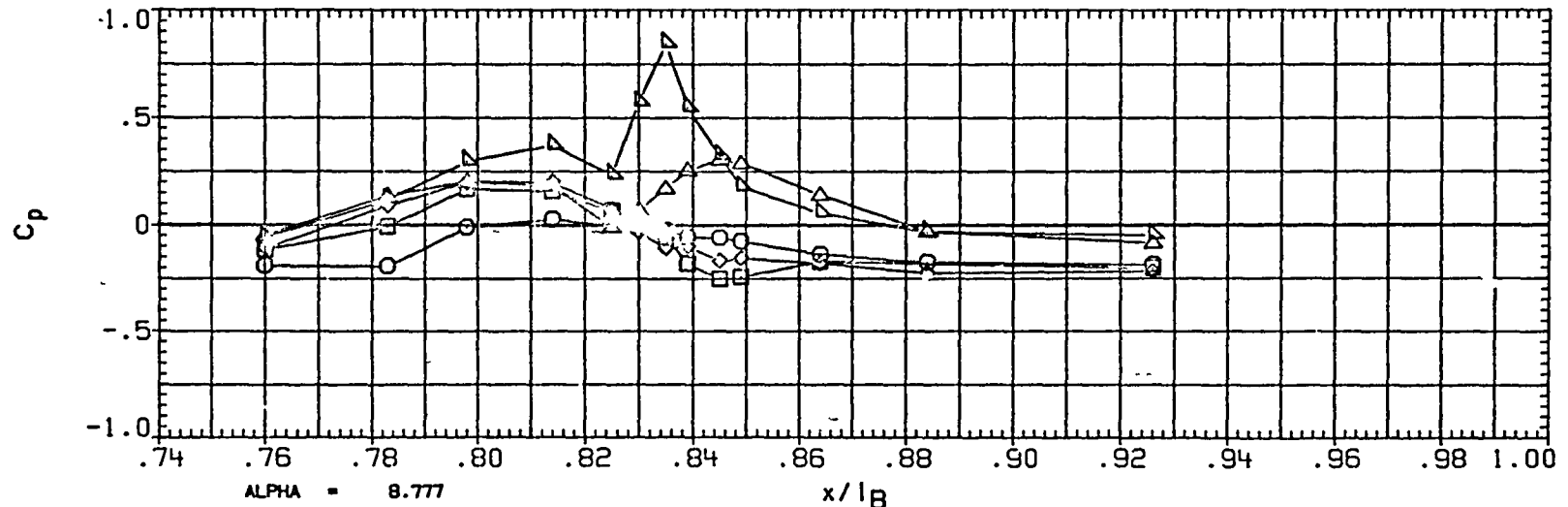
FIGURE 2D TYPICAL OA310B PRESSURE DISTRIBUTION - OMS P0D AND AFT FUSELAGE
