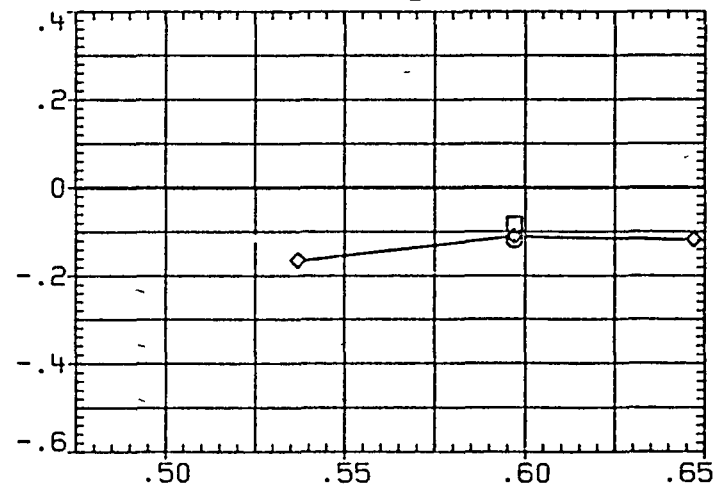
FIGURE 2C TYPICAL OA3103 PRESSURE DISTRIBUTION - MID-SIDE FUSELAGE
