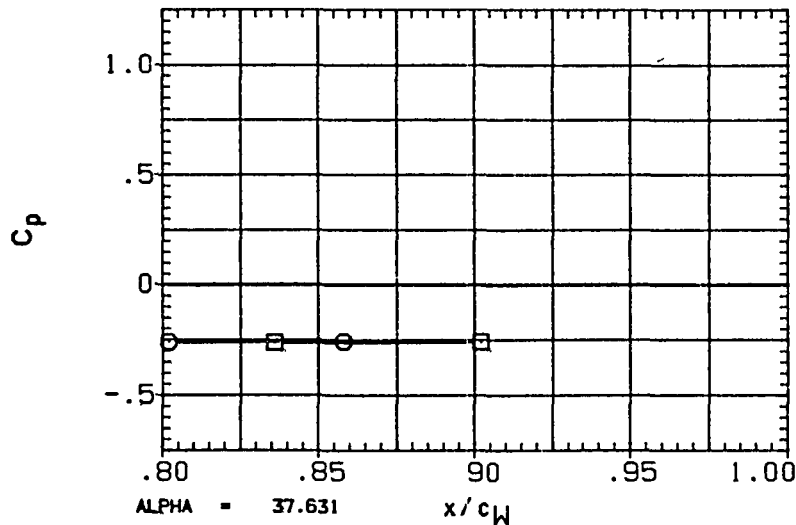
FIGURE 3H TYPICAL OA310C PRESSURE DISTRIBUTION - UPPER WING(RIGHT)
