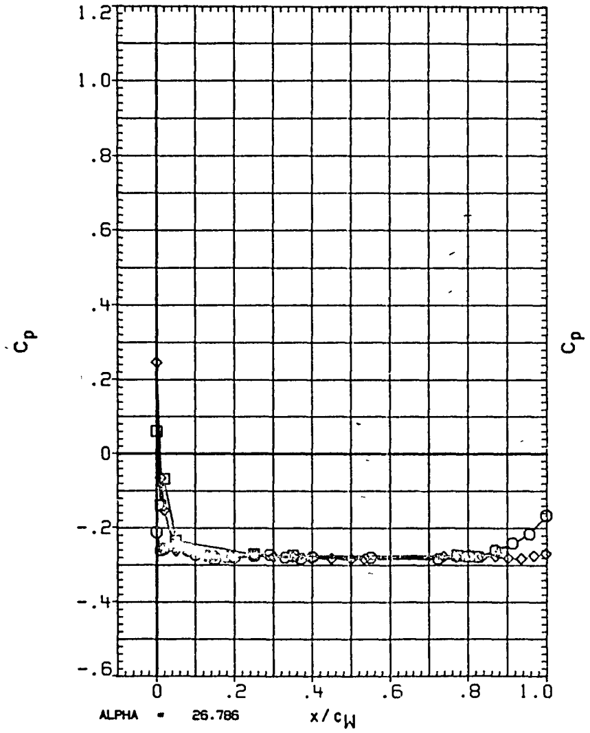
FIGURE 3G TYPICAL OA310C PRESSURE DISTRIBUTION - UPPER WING(LEFT)
