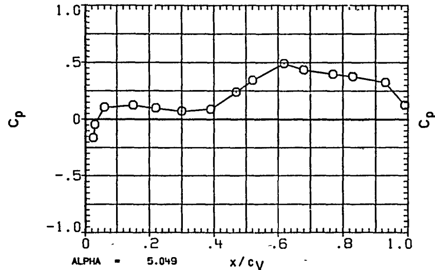
FIGURE 2E TYPICAL OA310B PRESSURE DISTRIBUTION - VERTICAL TAIL (LEFT FACE)
