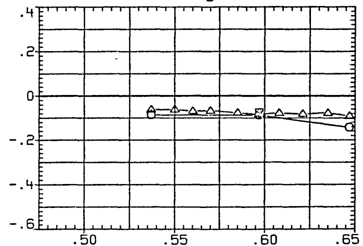
FIGURE 3C TYPICAL OA310C PRESSURE DISTRIBUTION - MID-SIDE FUSELAGE
