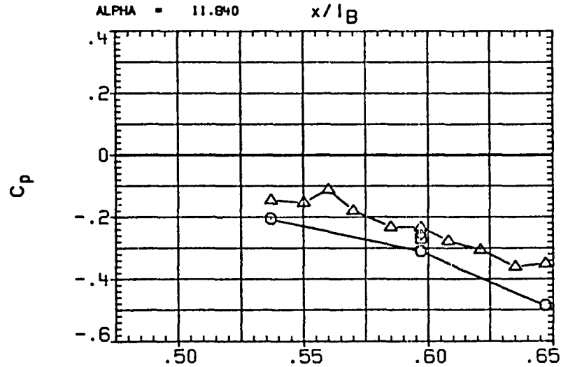
FIGURE 1C TYPICAL OA310A PRESSURE DISTRIBUTION - MID-SIDE FUSELAGE
