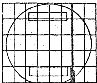
Figure 26 - Detector spacing variations; S= 25.4 mm
