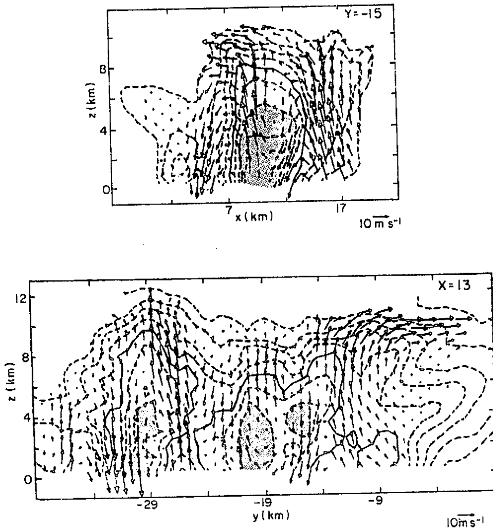
Fig. 5.6. Dual Doppler-derived velocity vectors (storm relative) in east-west and north-south planes at 1343 MDT. Echo contours and vector scales as in Fig. 5.1.
