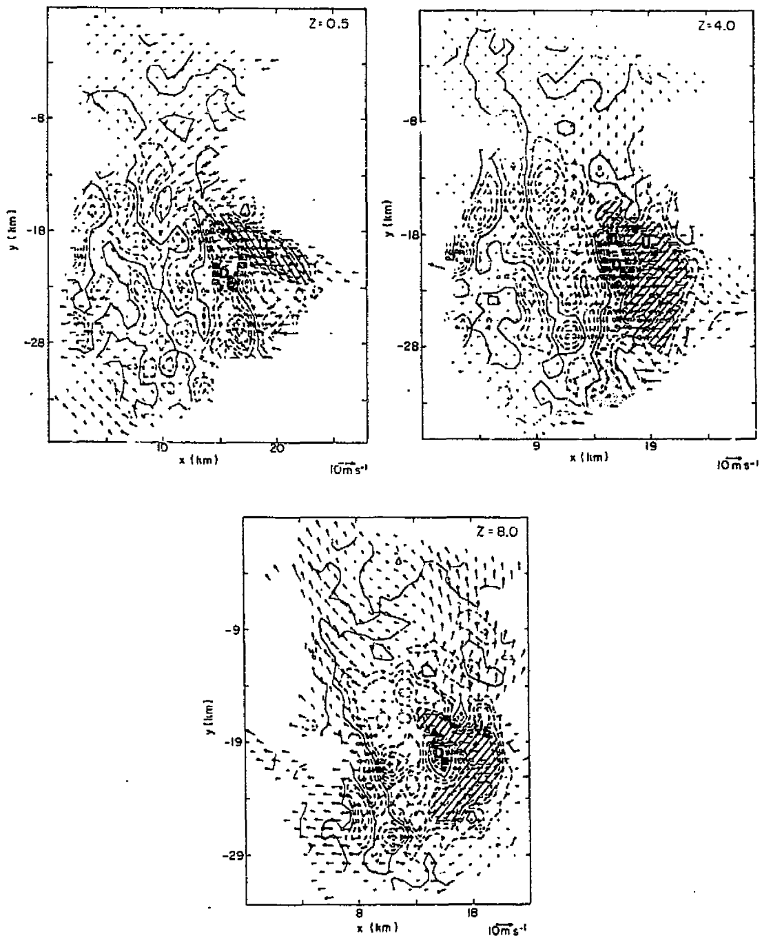
Fig. 5.9. Analyzed vertical motion for 1349 time period. Vertical velocity is in 4 \text{ m s}^{-1} intervals. Updraft U_3 is cross hatched; and downdraft D_5 is stippled.
