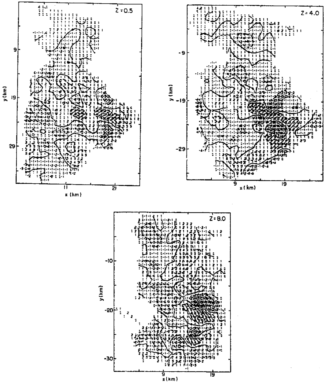
Fig. 5.17. Same as Fig. 5.15, for 1349 MDT.
