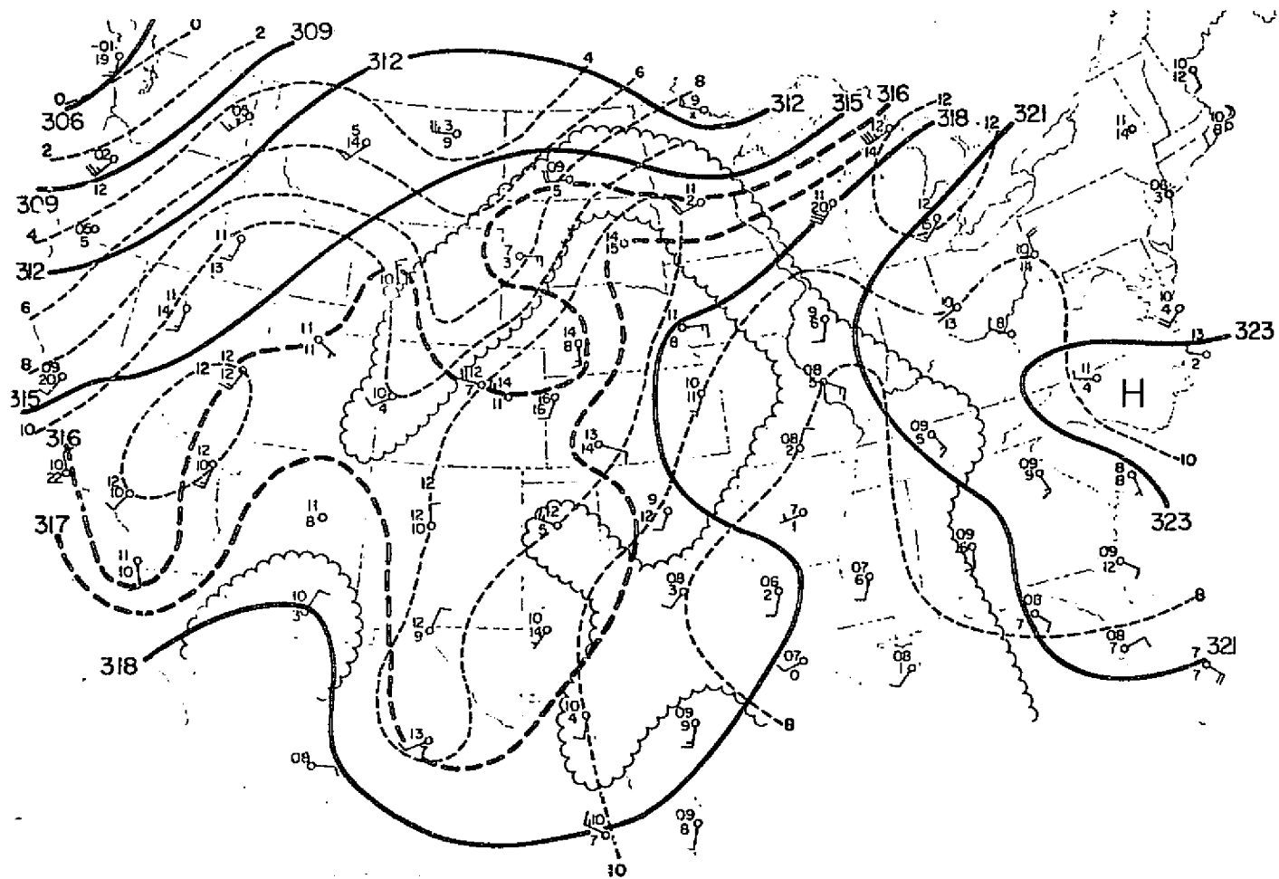
Fig. 4.3. 70 kpa analysis for 0600 MDT 20 July 1977. Areas with a dew-point depression ( T-T_d ) less than 6\text{ }^{\circ}\text{C} are marked. The primary contours (solid lines) are drawn at 30 m intervals, and secondary contours (heavy dashed lines) are drawn at 10 m intervals. Thin dashed lines depict isotherms.
