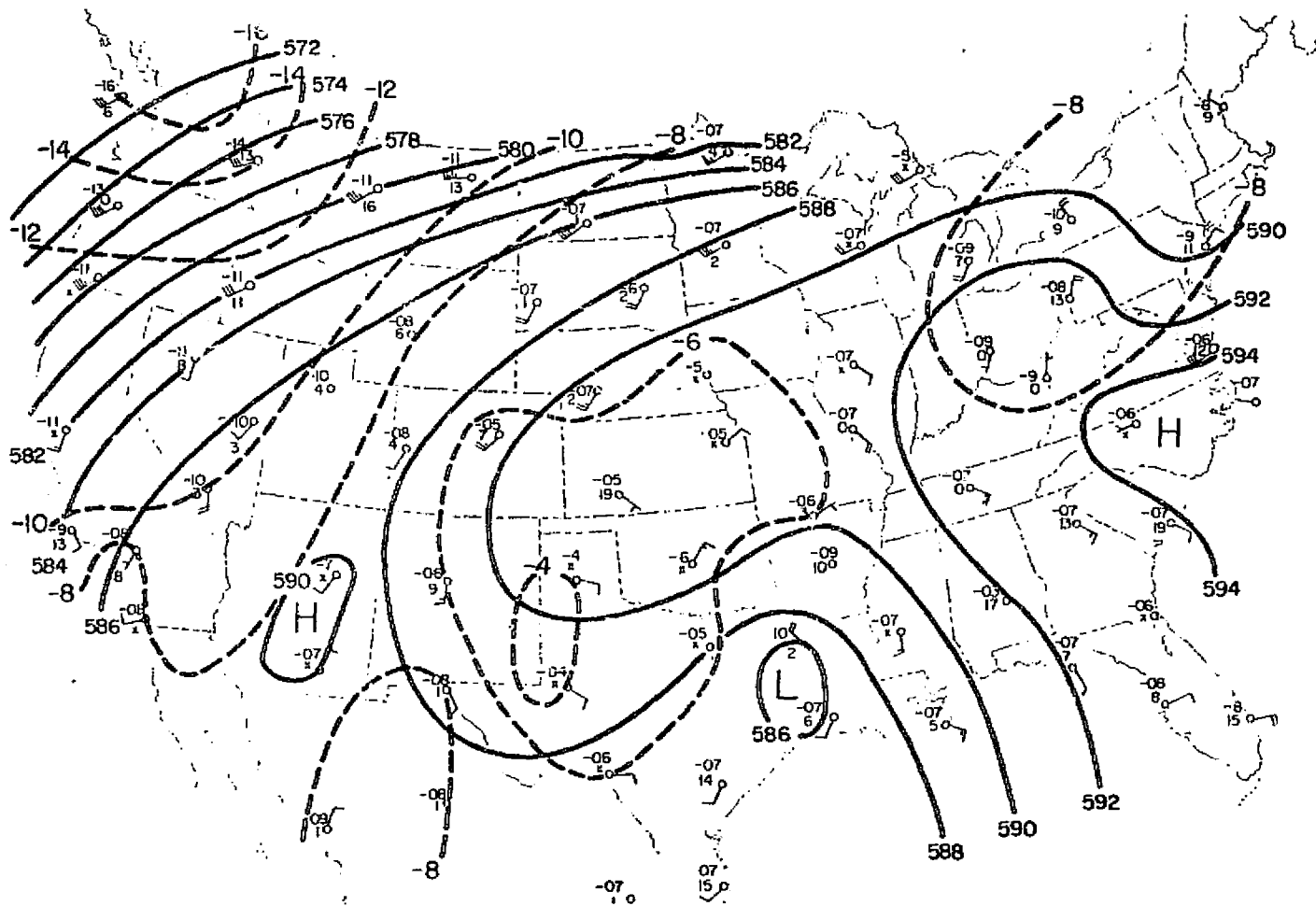
Fig. 4.4. 50 kpa analysis for 0600 MDT 20 July 1977. Height contours are labelled in decameters. Dashed lines depict isotherms.
