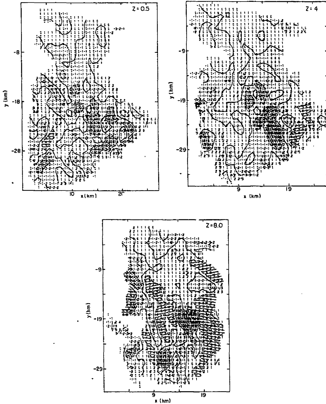
Fig. 5.11. Analyzed divergence patterns for 1349 time period. Contours are in 2.0 \times 10^{-3} intervals. Divergence > 2 \times 10^{-3} are cross hatched; and < -2.0 \times 10^{-3} are stippled.
