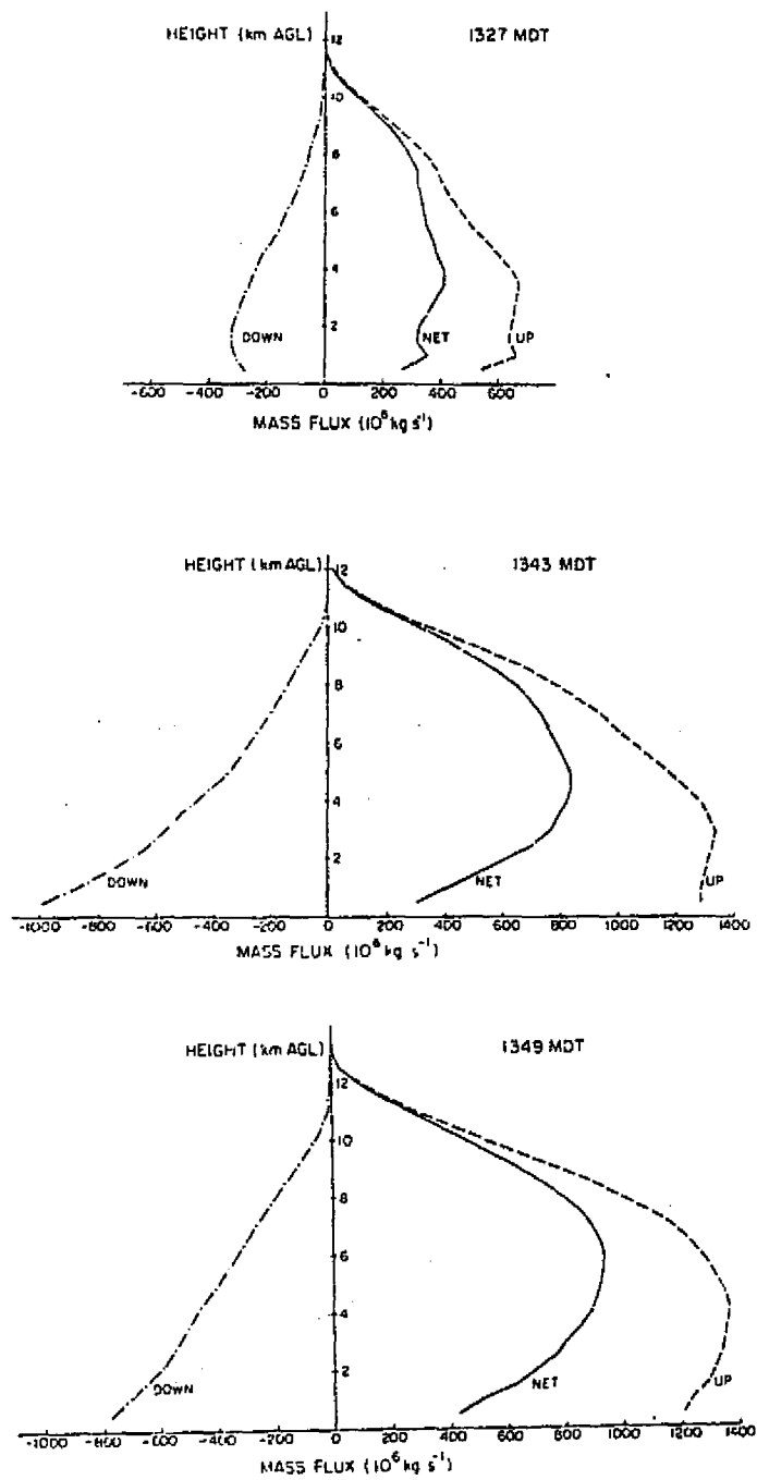
Fig. 5.12. Vertical profiles of mass flux for 1327, 1343 and 1349 time periods.
