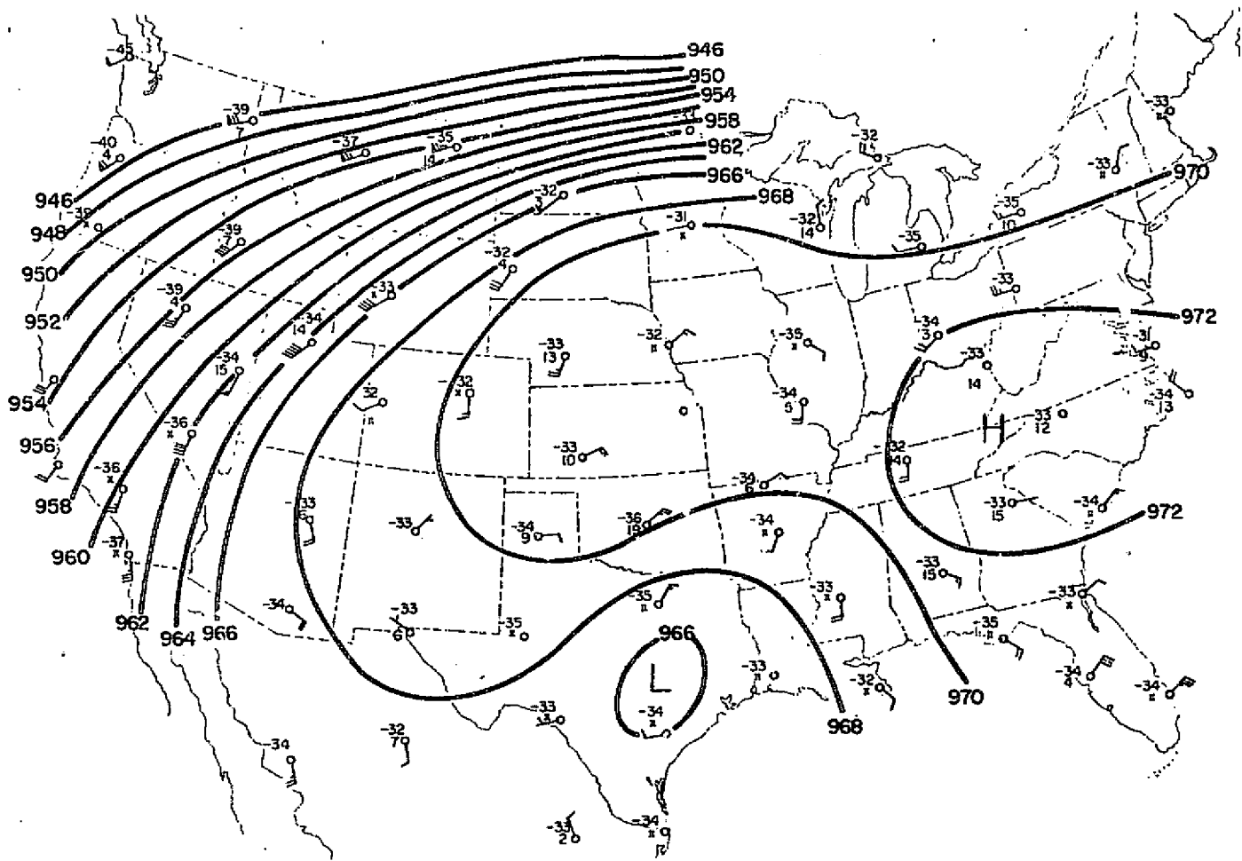
Fig. 4.5. 30 kpa analysis for 0600 MDT 20 July 1977. Height contours are labelled in decameters.
