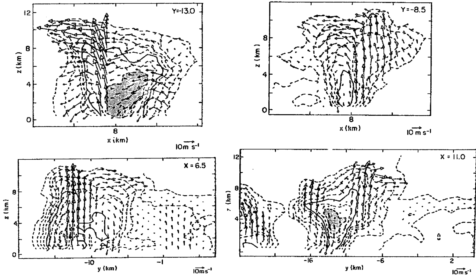
Fig. 5.3. Dual Doppler-derived velocity vectors (storm relative) in east-west and north-south vertical planes at 1327 MDT. Echo contours and vector scales as in Fig. 5.1.
