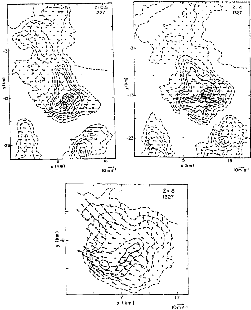
Fig. 5.1. Horizontal cross section of reflectivity and storm relative vectors. Echo contours are given in 5 dBZ intervals beginning at 10 dBZ, with 30 dBZ solid. Echo intensities greater than 40 dBZ are shaded. A 10 \text{ m s}^{-1} vector scale is shown in the lower right-hand corner of each panel.
