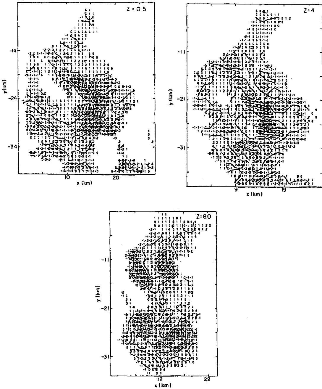
Fig. 5.16. Same as Fig. 5.15, for 1343 MDT.
