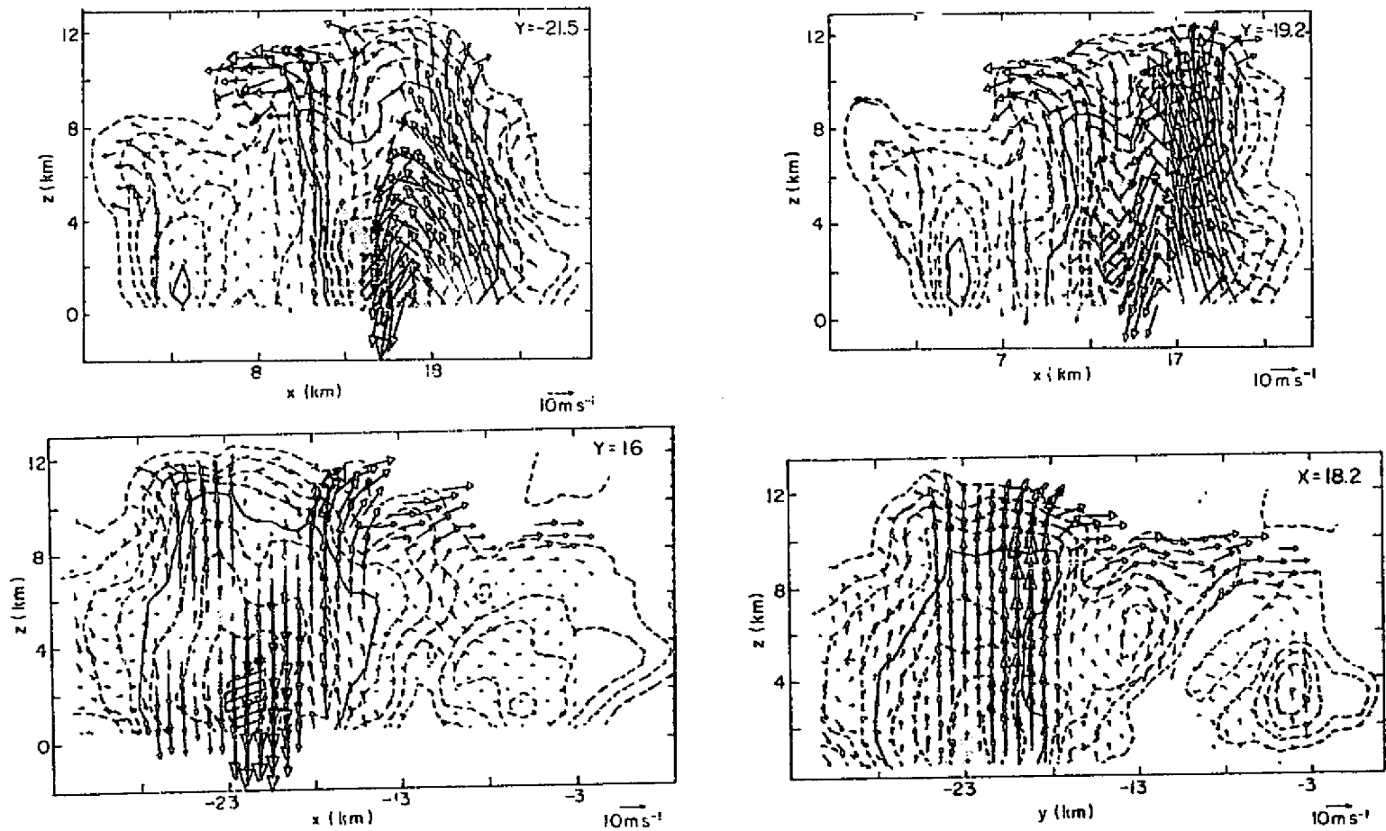
Fig. 5.10. Dual Doppler-derived velocity vectors (storm relative) in east-west and north-south planes at 1343 MDT. Echo contours and vector scales as in Fig. 5.1.
