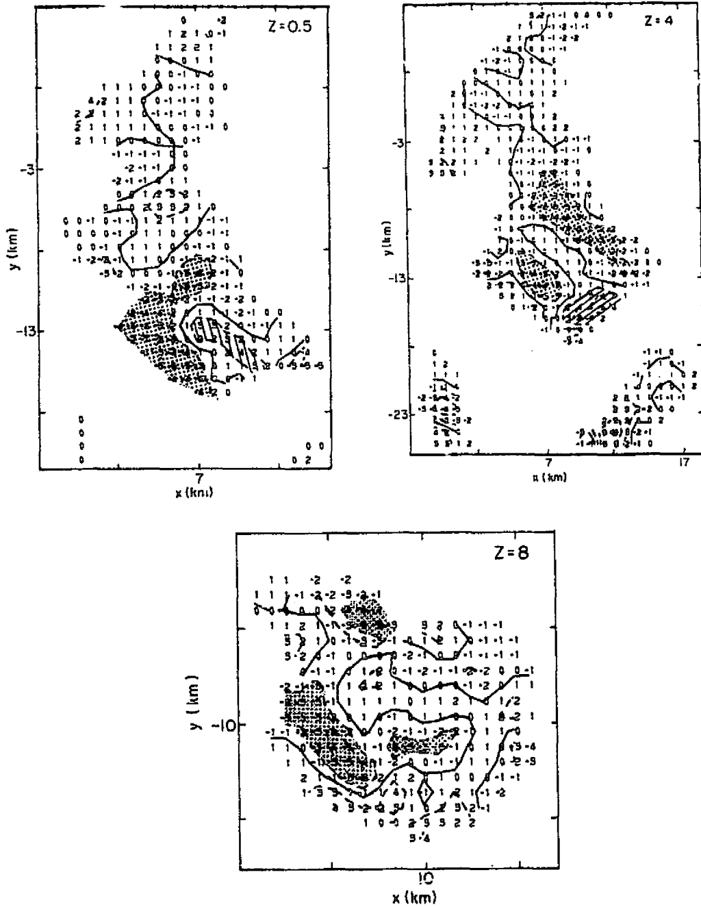
Fig. 5.15. Analyzed vorticity patterns for 1327 time period. Contours are in 2.0 \times 10^{-3} intervals. Hatched and stippled areas represent major cyclonic and anticyclonic vorticity regions, respectively.
