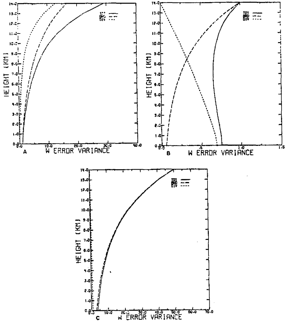
Fig. B.1. Vertical profiles of w error variance. Random errors in horizontal divergence are derived from two-radar analysis (curve labeled DIV) while uncertainty of boundary condition (curve labeled BND) is specified. Total w error variance profile (TOT) is sum of profiles DIV and BND. (A) error profiles for upward integration, with \sigma^2 w_1 = 1 \text{ m}^2 \text{ s}^{-2} ; (B) for downward integration; (C) as in Fig. B.1B, \sigma^2 w_N = 50 \text{ m}^2 \text{ s}^{-2} . From Ray et al. (1980)
