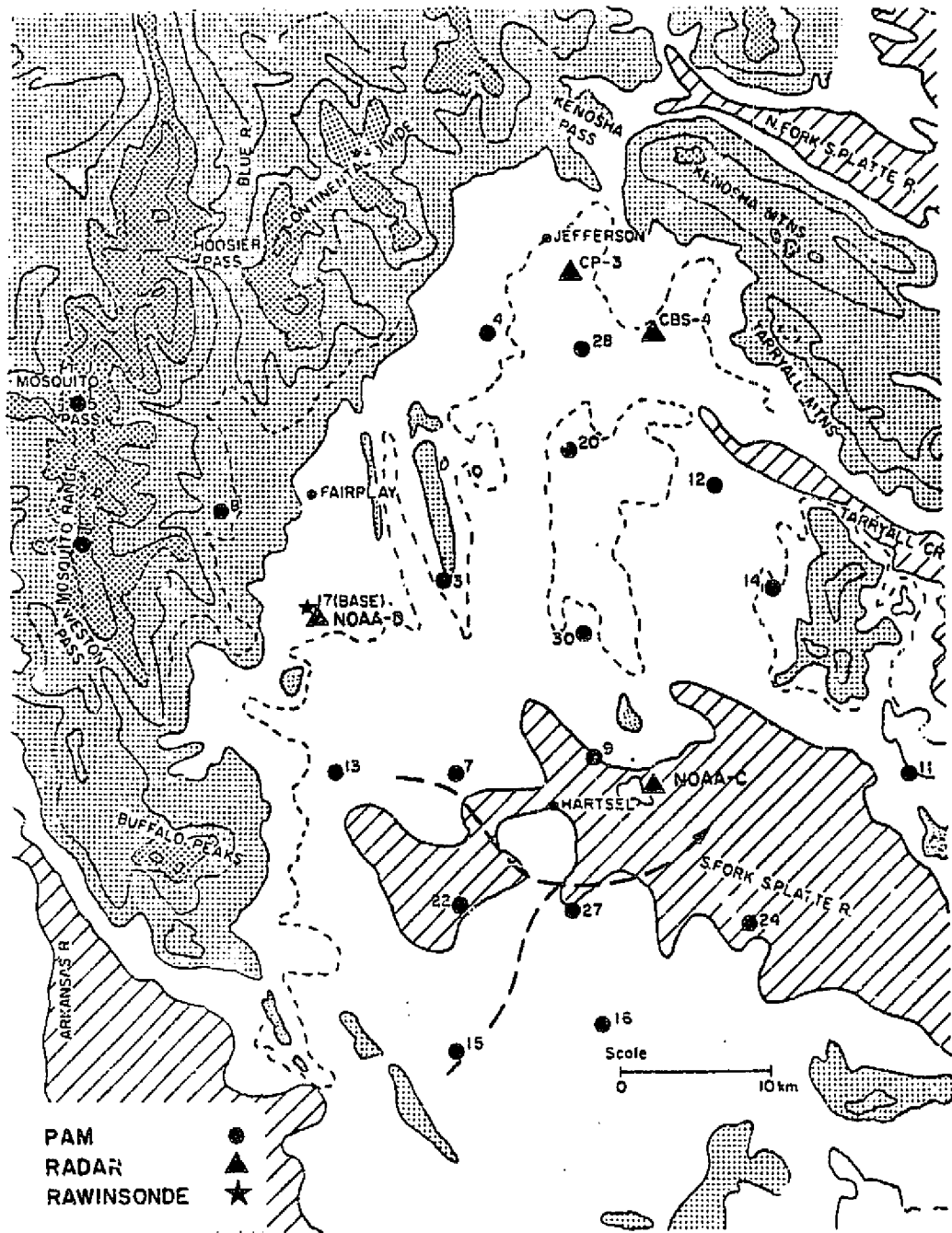
Fig. 3.1. Map of terrain in South Park, Colorado. Regions below 9000 ft. (2744 m) are hatched; regions above 10,000 ft. (3049m) are lightly shaded; and regions above 12,000 ft. (3657m) are heavily shaded; contours intervals are 1000 ft. (305 m). Dash line depicts trajectory of the storm.
