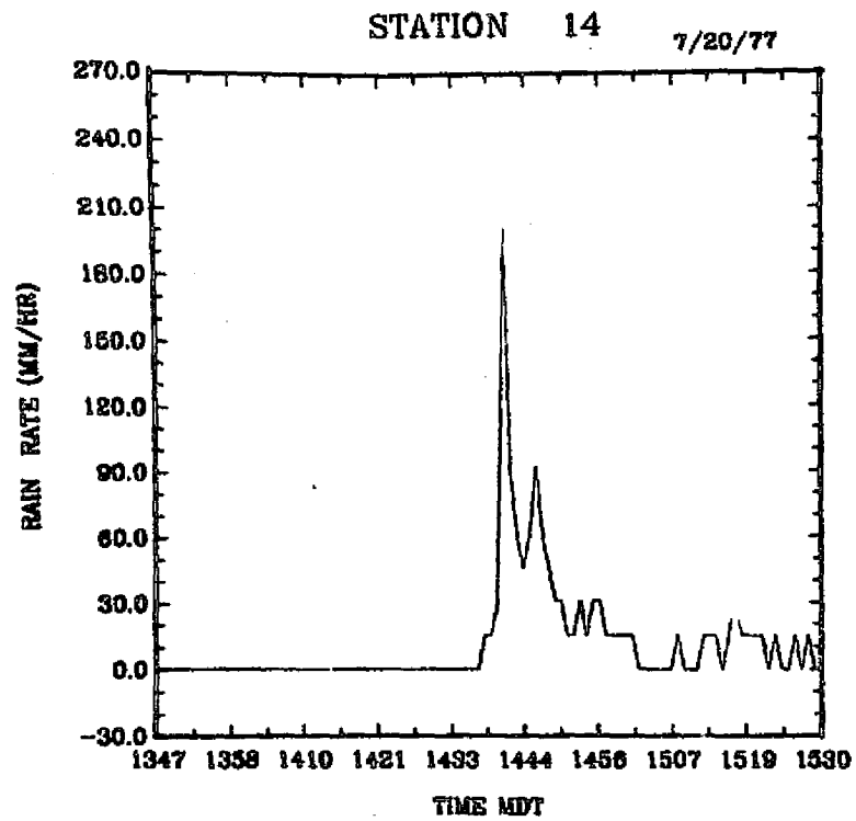
Fig. 4.16. One-minute rainfall rates for selected stations and time intervals. The rates are derived from PAM tipping-bucket raingauges.
