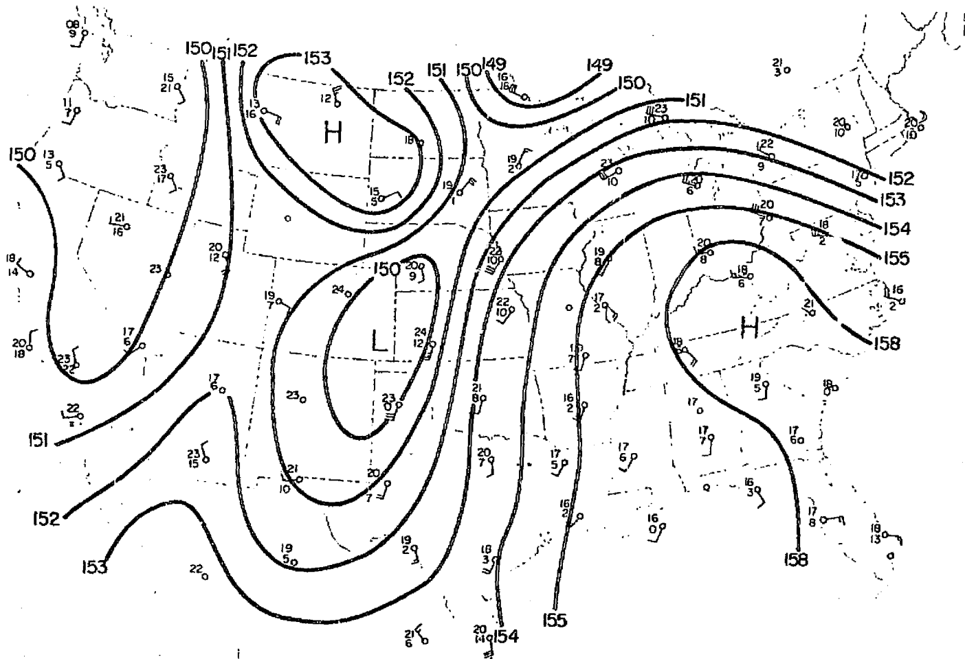
Fig. 4.2. 85 kpa analysis for 0600 MDT (12 GMT) 20 July 1977. Height contours are labelled in decameters.
