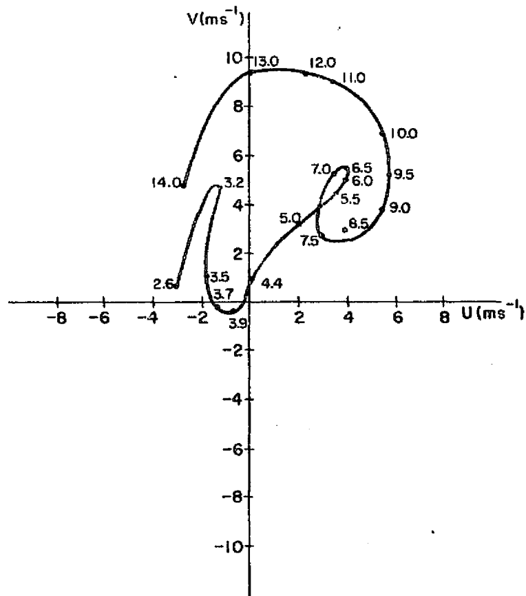
Fig. 4.9. Environmental wind hodograph derived from the 1003 MDT South Park sounding. Numbers adjacent to hodograph curve denote height in km MSL.
