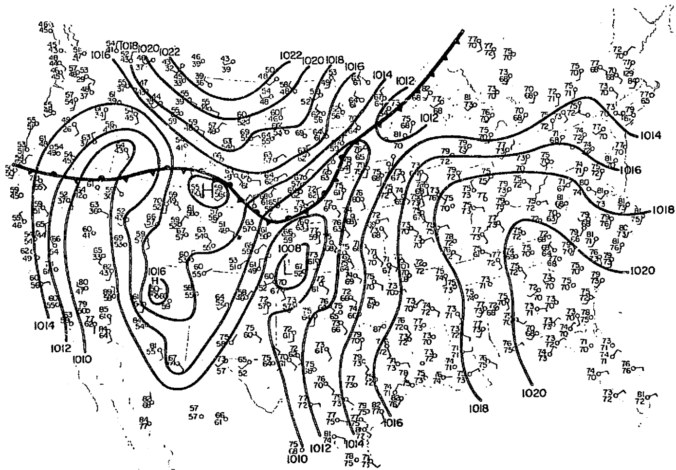
Fig. 4.1. Surface synoptic patterns for 0600 MDT 20 July 1977. The star denotes the location of South Park.
