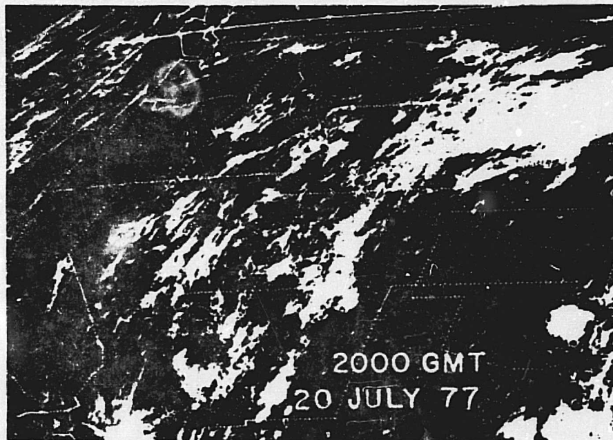
Fig. 4.6. Visible satellite images of the western United States, for 1900 and 2000 GMT, 20 July 1977. Dotted lines are state boundaries.
