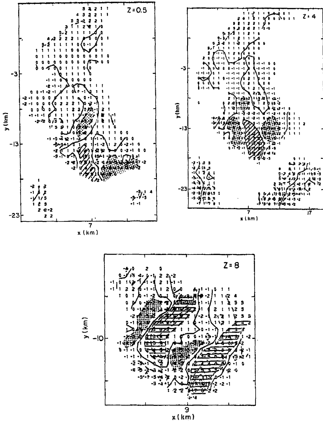
Fig. 5.4. Analyzed divergence patterns for 1327 time period. Contours are in 2.0 \times 10^{-3} intervals. Divergence > 2 \times 10^{-3} are cross hatched; and < -2.0 \times 10^{-3} are stippled.
