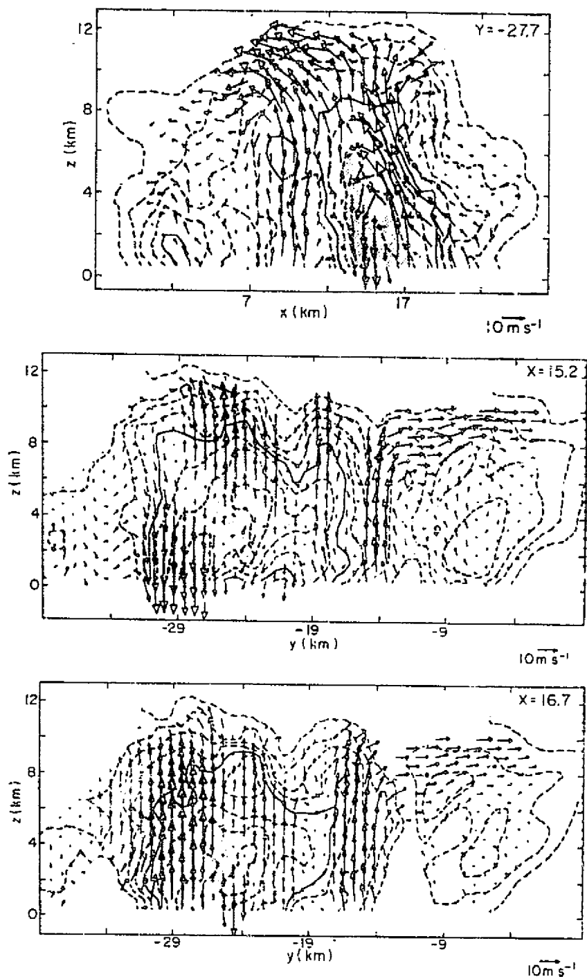
Fig. 5.7. Dual Doppler-derived velocity vectors (storm relative) in east-west and north-south planes at 1343 MDT. Echo contours and vector scales as in Fig. 5.1.
