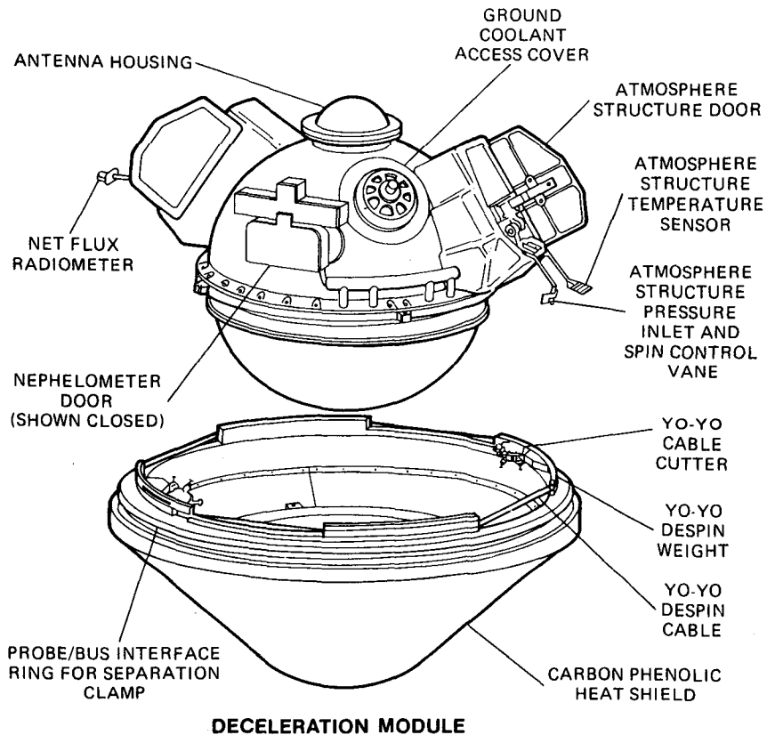
Figure 3-6. Small Probes
