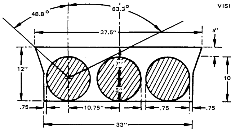
Figure 4-4. Tray Utilization Profiles
