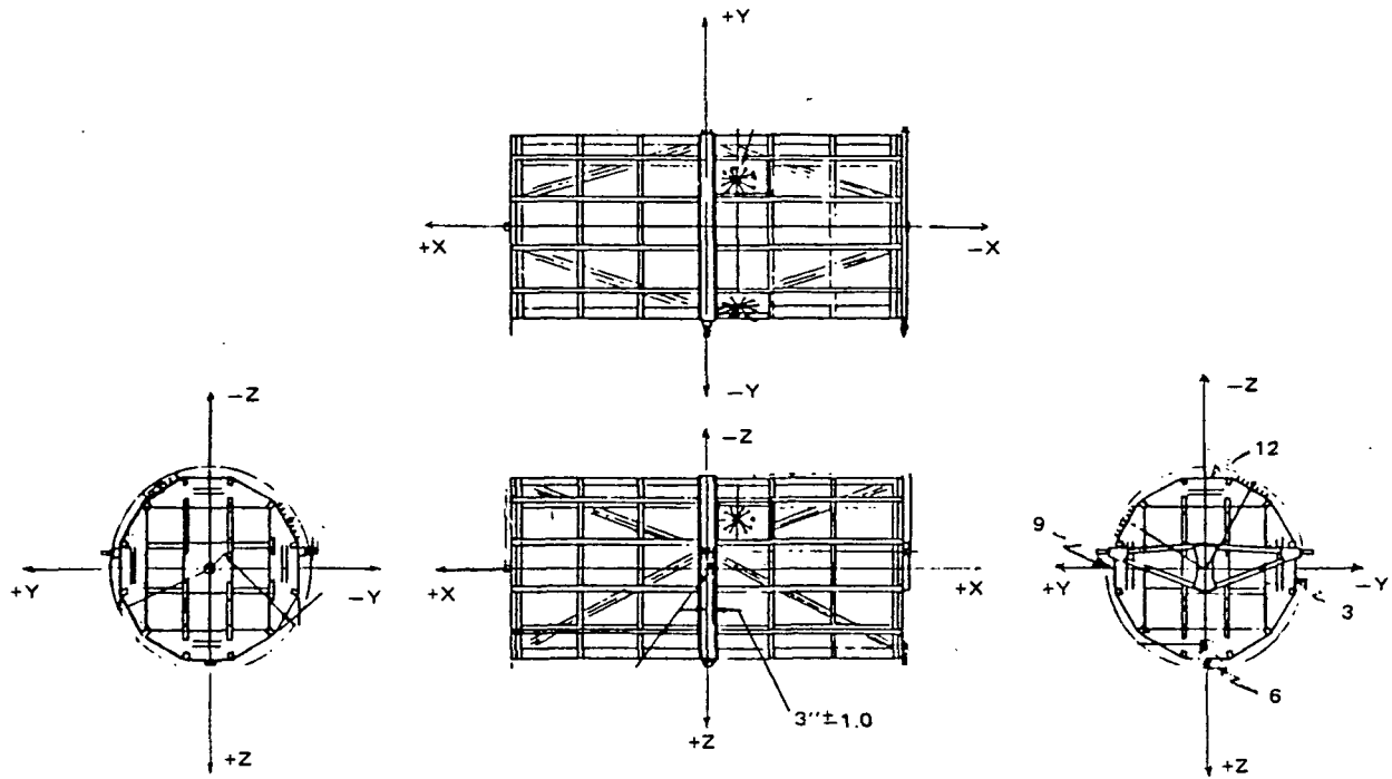
Figure 4-5. The LDEF Coordinate System
