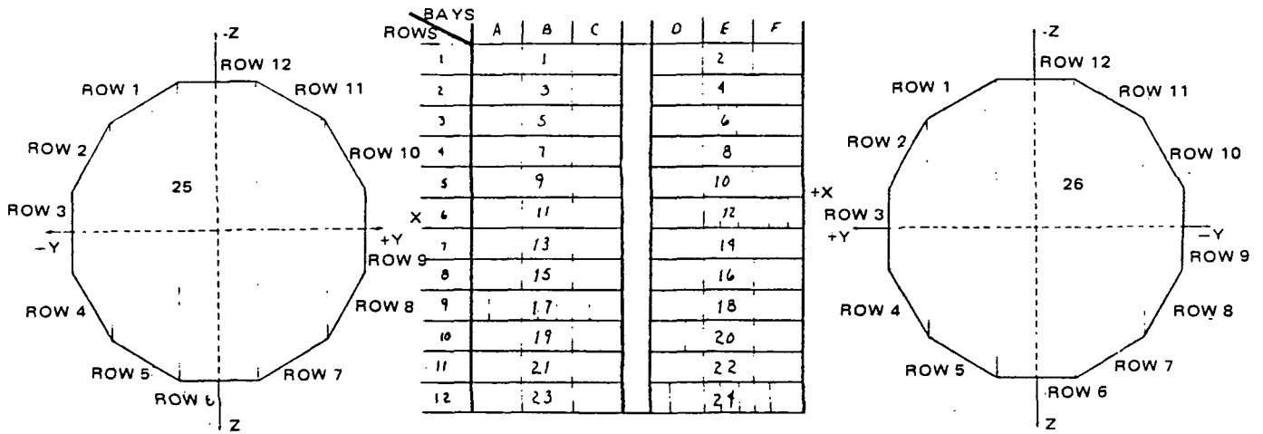
Figure 4-6. Definition of LDEF Rough-Surface Scattering Areas
