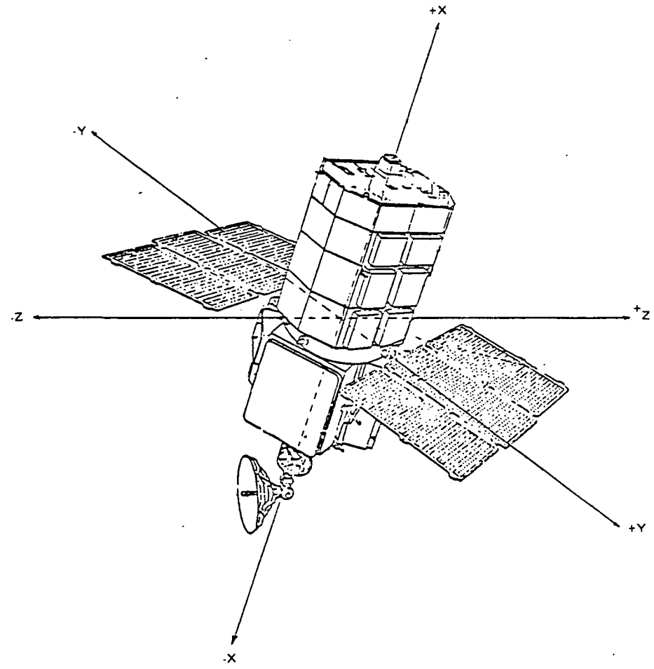
Figure 4-11. SMM Coordinate System
