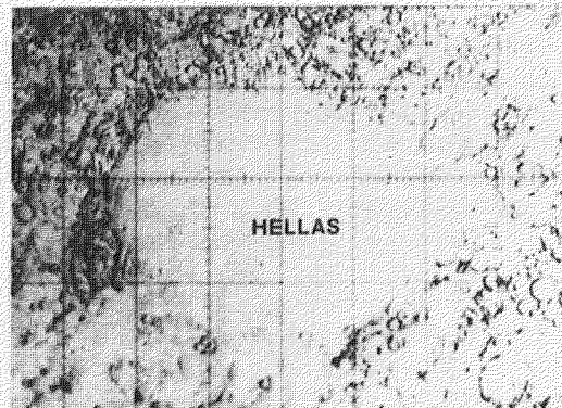
HELLAS (MARS)
