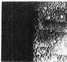
CALORIS (MERCURY)
