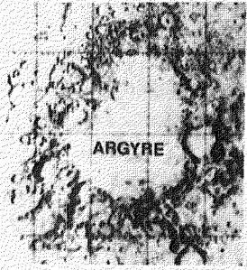
ARGYRE (MARS)
