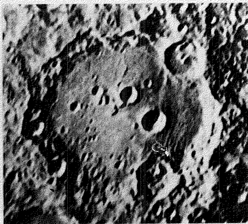
CLAVIUS (MOON)
