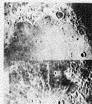
IMBRIUM (MOON)
