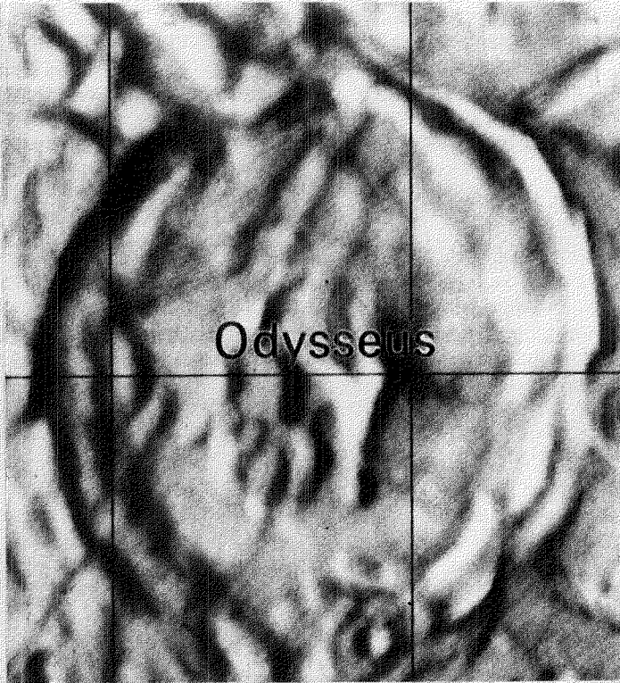
ODYSSEUS (TETHYS)
