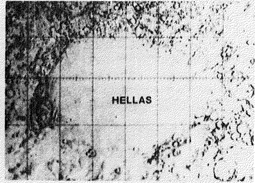
HELLAS (MARS)
