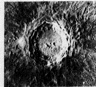
COPERNICUS (MOON)
