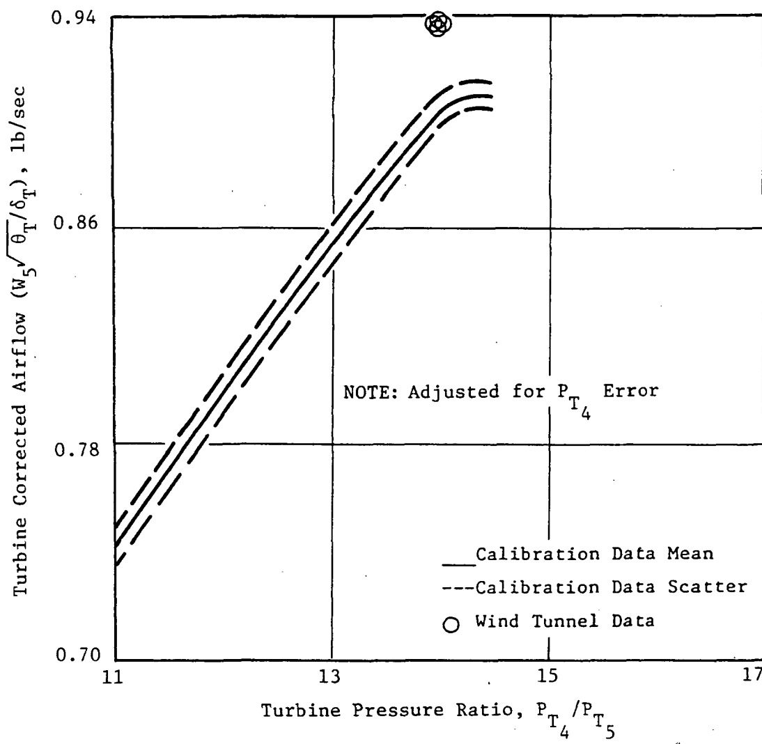
Figure 28f. E^3 Separate Flow Turbomachinery Characteristics.
