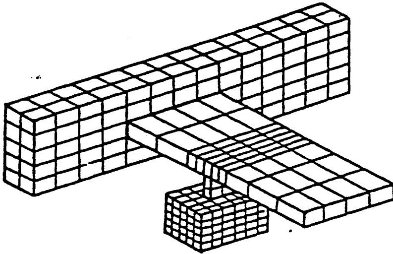
Computational space
