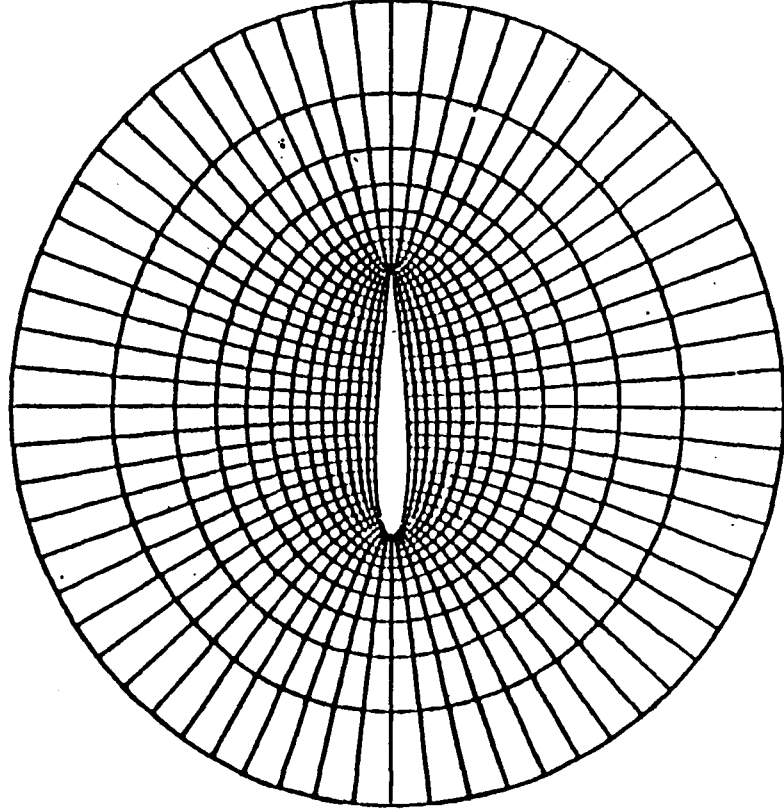
SINGLE-BLOCK GRID
