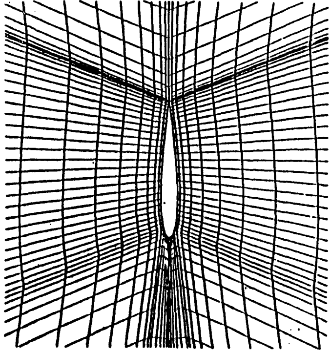
MULTIPLE-BLOCK GRID
