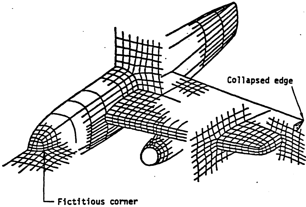
Physical space
