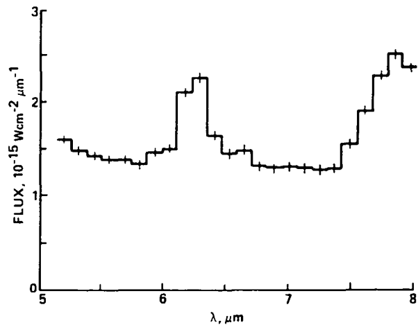
Figure 5. A spectrum of HD44179 (the Red Rectangle) obtained from the KAO with 12 min of integration. The unknown dust emission features near 6.2 and 7.7 \mu\text{m} are prominent.
