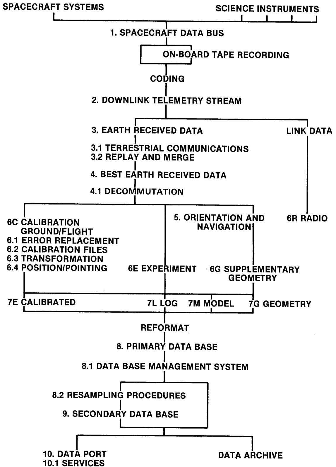
FIGURE 2.1 GENERAL DOWNLINK DATA FLOW
