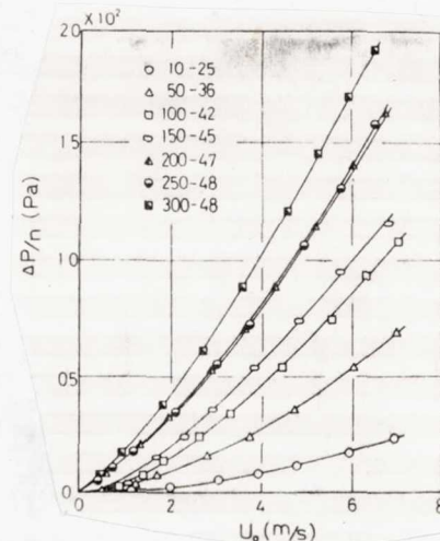
Figure 7. Pressure drop of each mesh
