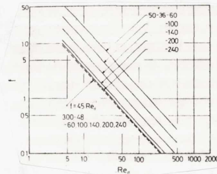
Figure 14. The changes of lamination number and coefficient of friction (arranged by wire diameter)
