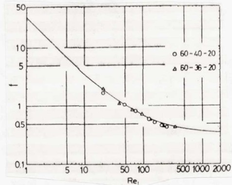
Figure 6. Pitch ratio and coefficient of friction
